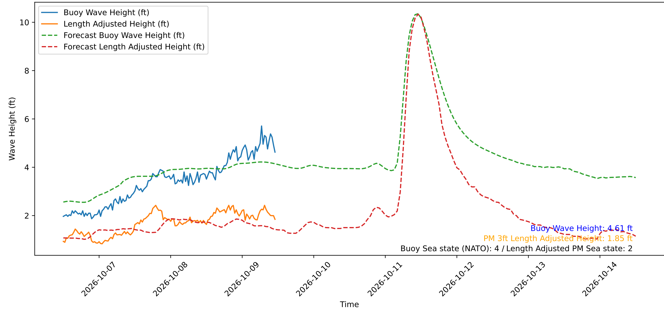
Wave Heights over Time for Red Beach at 2026-10-09 11:40:49
