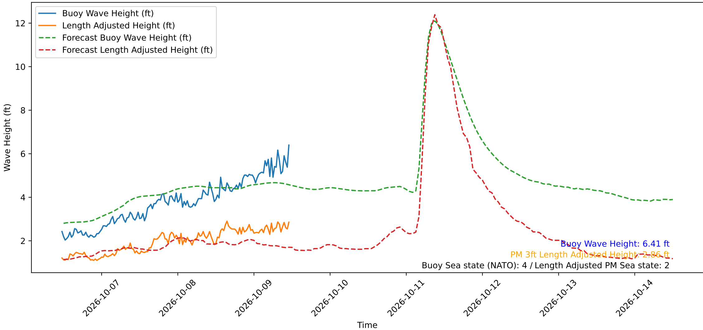
Wave Heights over Time for Oceanside Harbor at 2026-10-09 11:40:30
