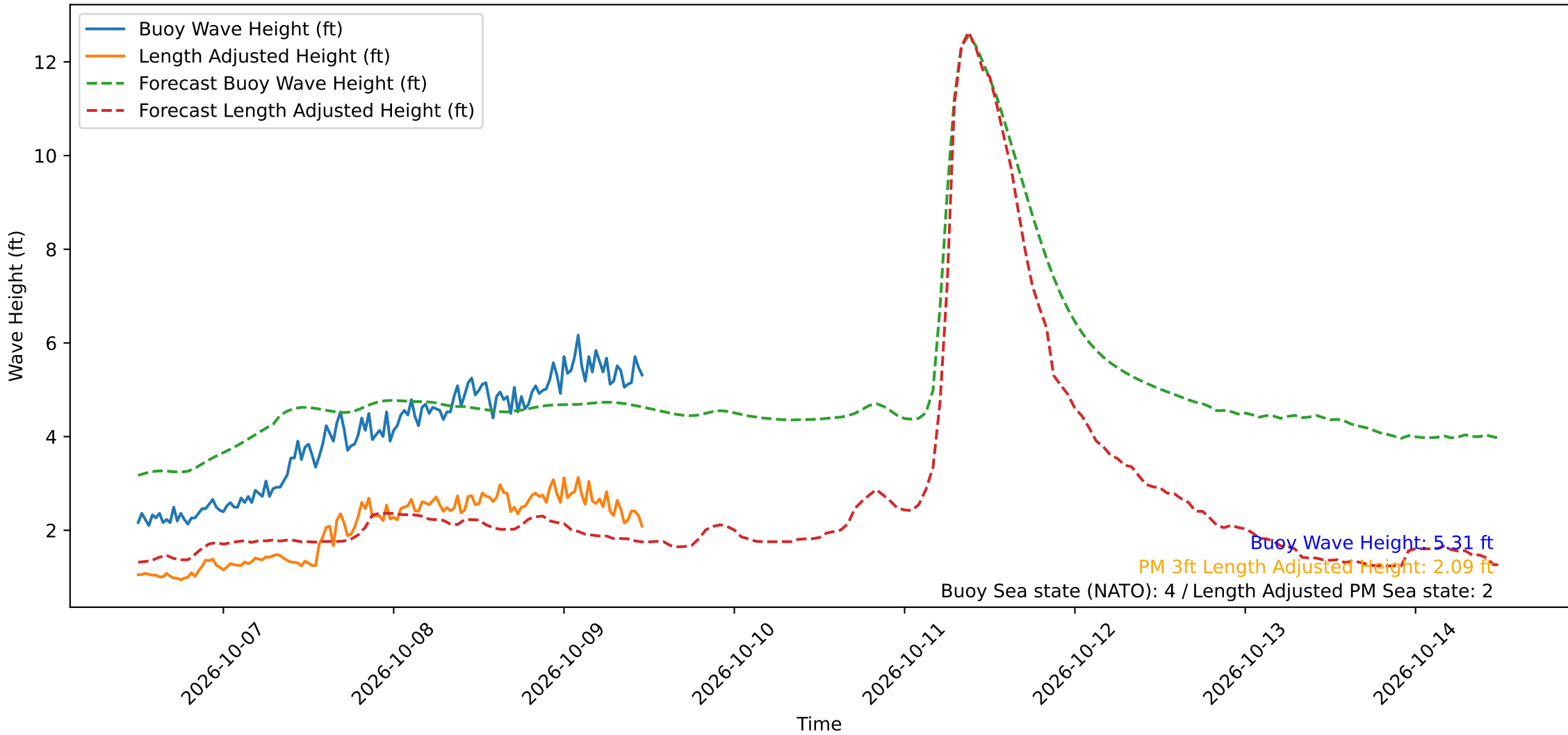
Wave Heights over Time for Green Beach at 2026-10-09 11:41:11
