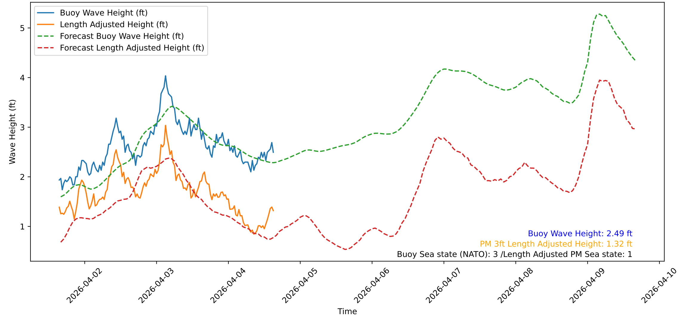
Wave Heights over Time for Oceanside Harbor at 2026-04-04 15:40:35
