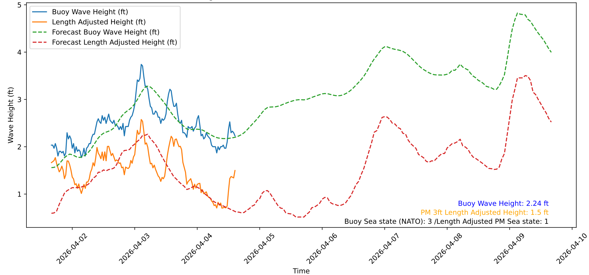
Wave Heights over Time for Red Beach at 2026-04-04 15:40:53
