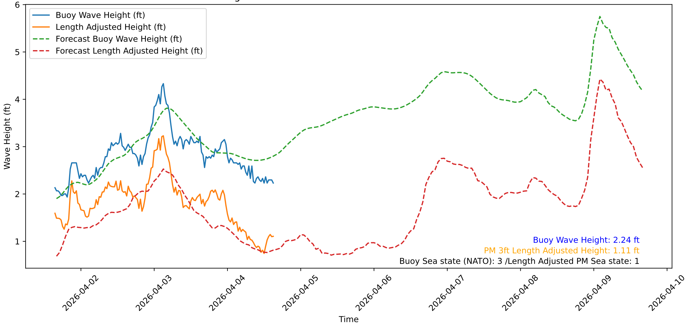
Wave Heights over Time for Green Beach at 2026-04-04 15:41:17
