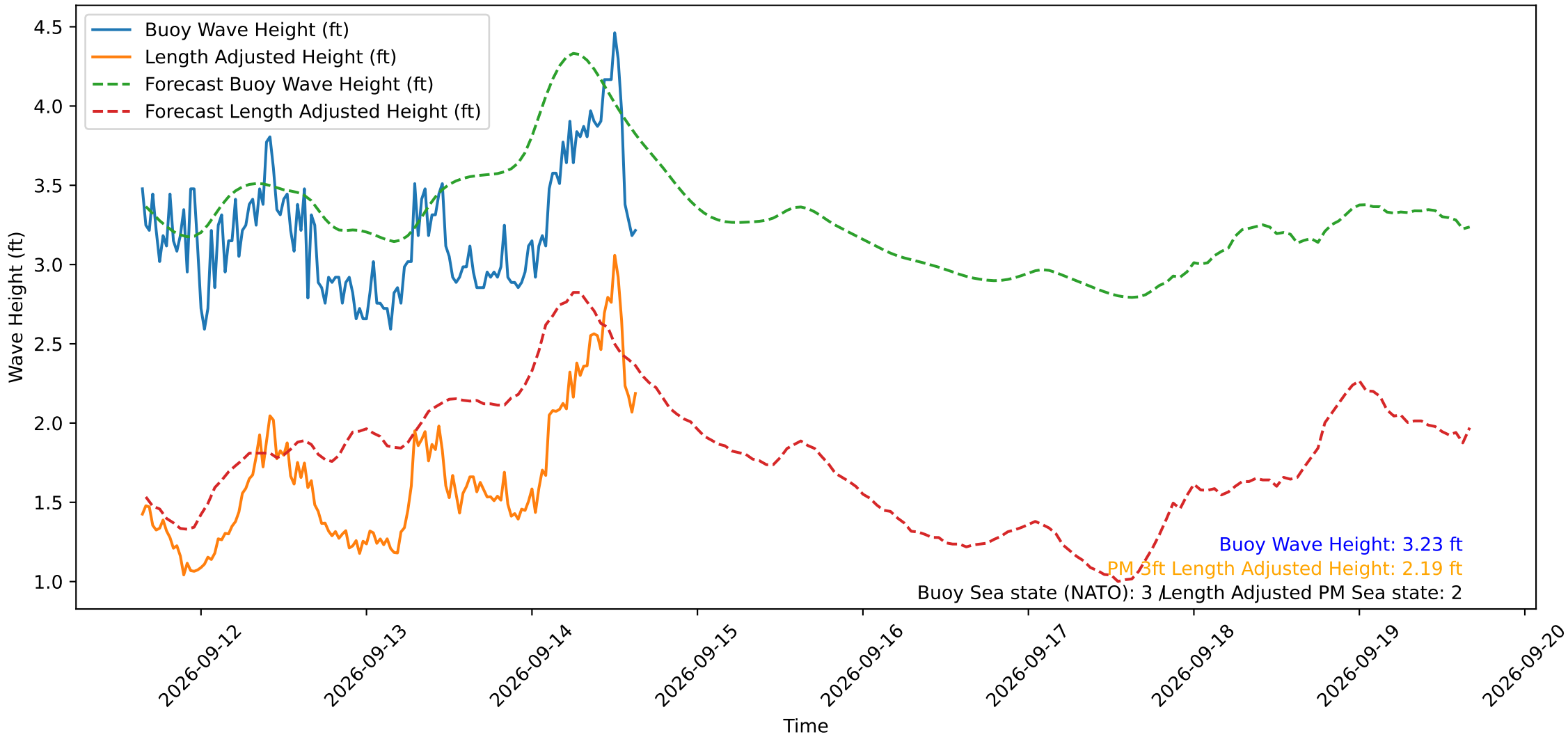
Wave Heights over Time for Oceanside Harbor at 2026-09-14 15:40:29
