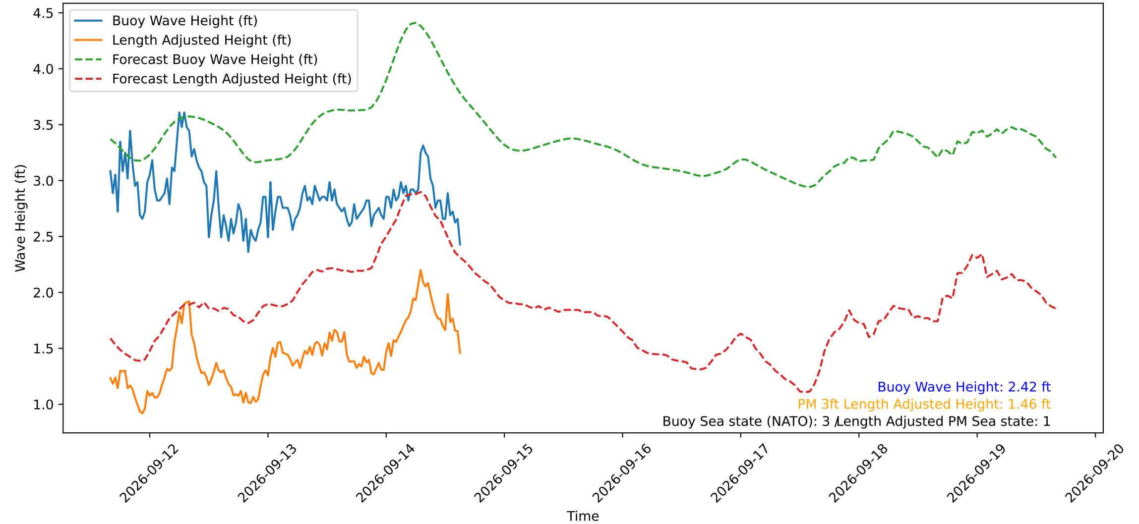
Wave Heights over Time for Green Beach at 2026-09-14 15:41:10
