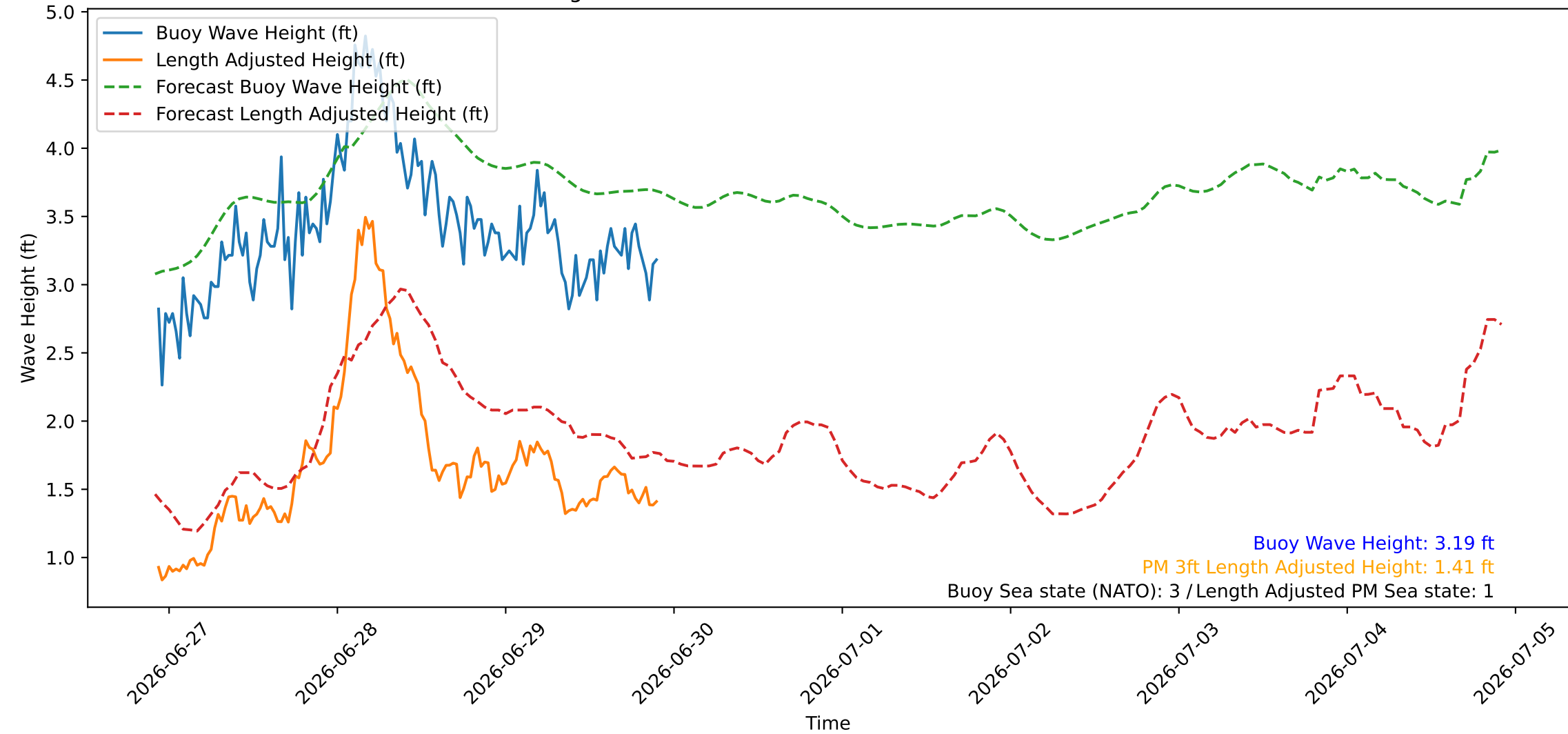
Wave Heights over Time for Green Beach at 2026-06-29 22:21:09
