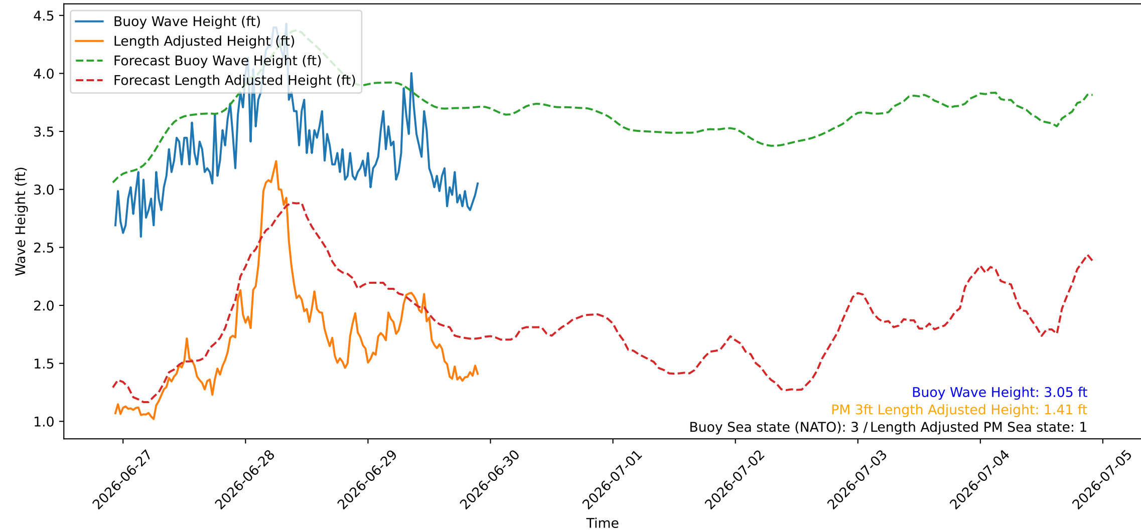
Wave Heights over Time for Oceanside Harbor at 2026-06-29 22:20:26
