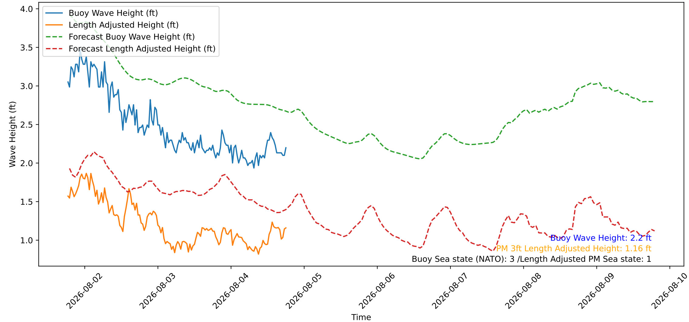
Wave Heights over Time for Green Beach at 2026-08-04 18:41:10
