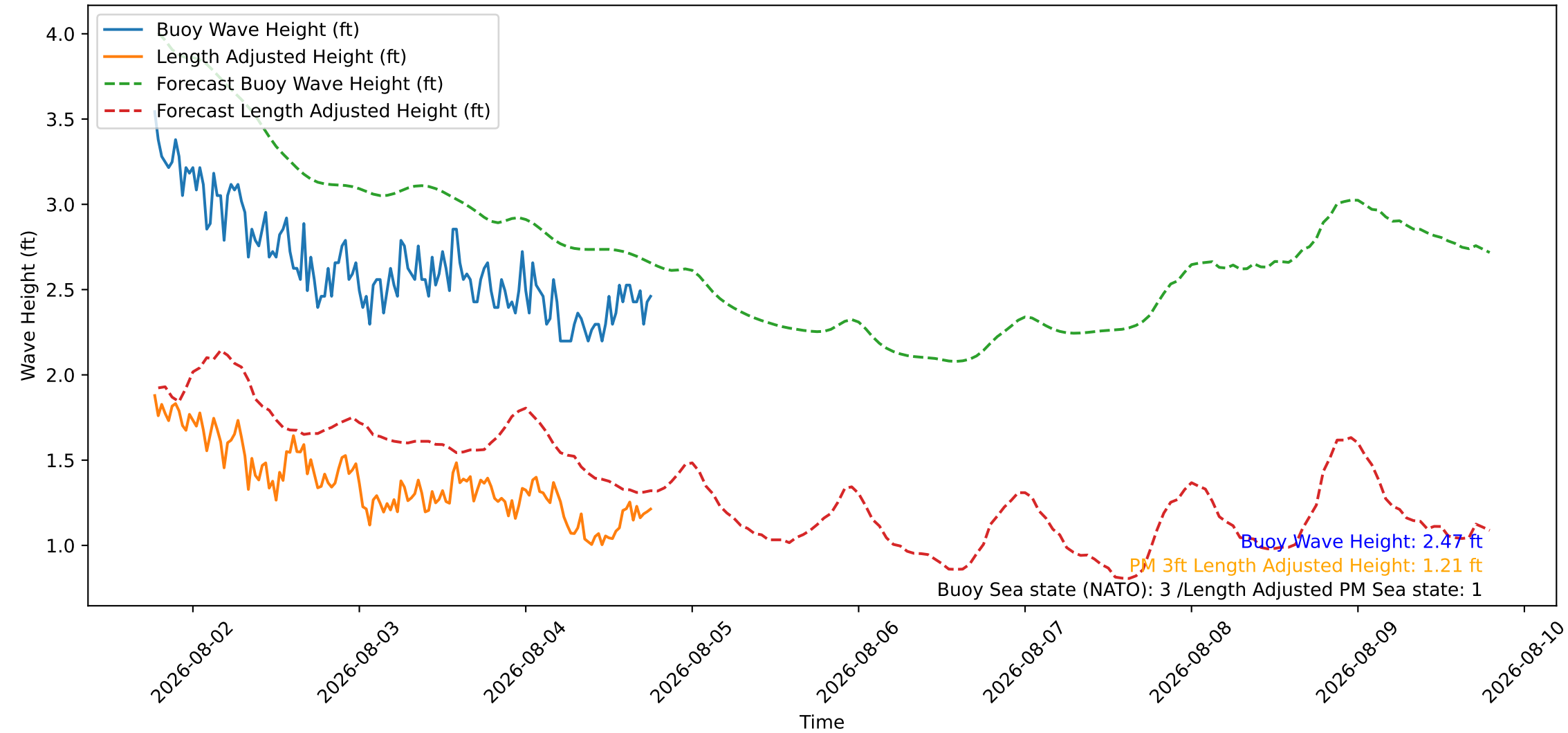
Wave Heights over Time for Oceanside Harbor at 2026-08-04 18:40:27
