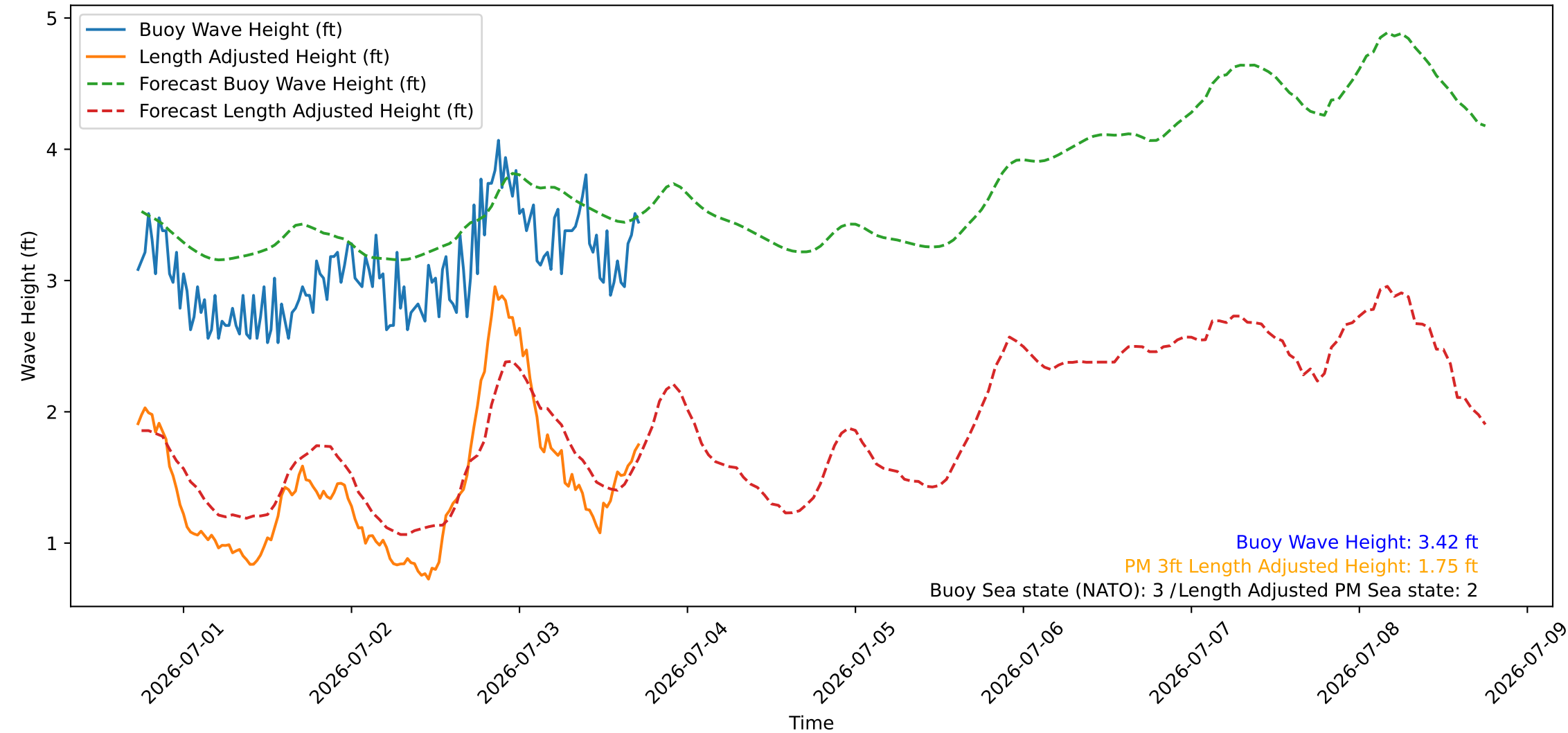
Wave Heights over Time for Green Beach at 2026-07-03 17:41:08
