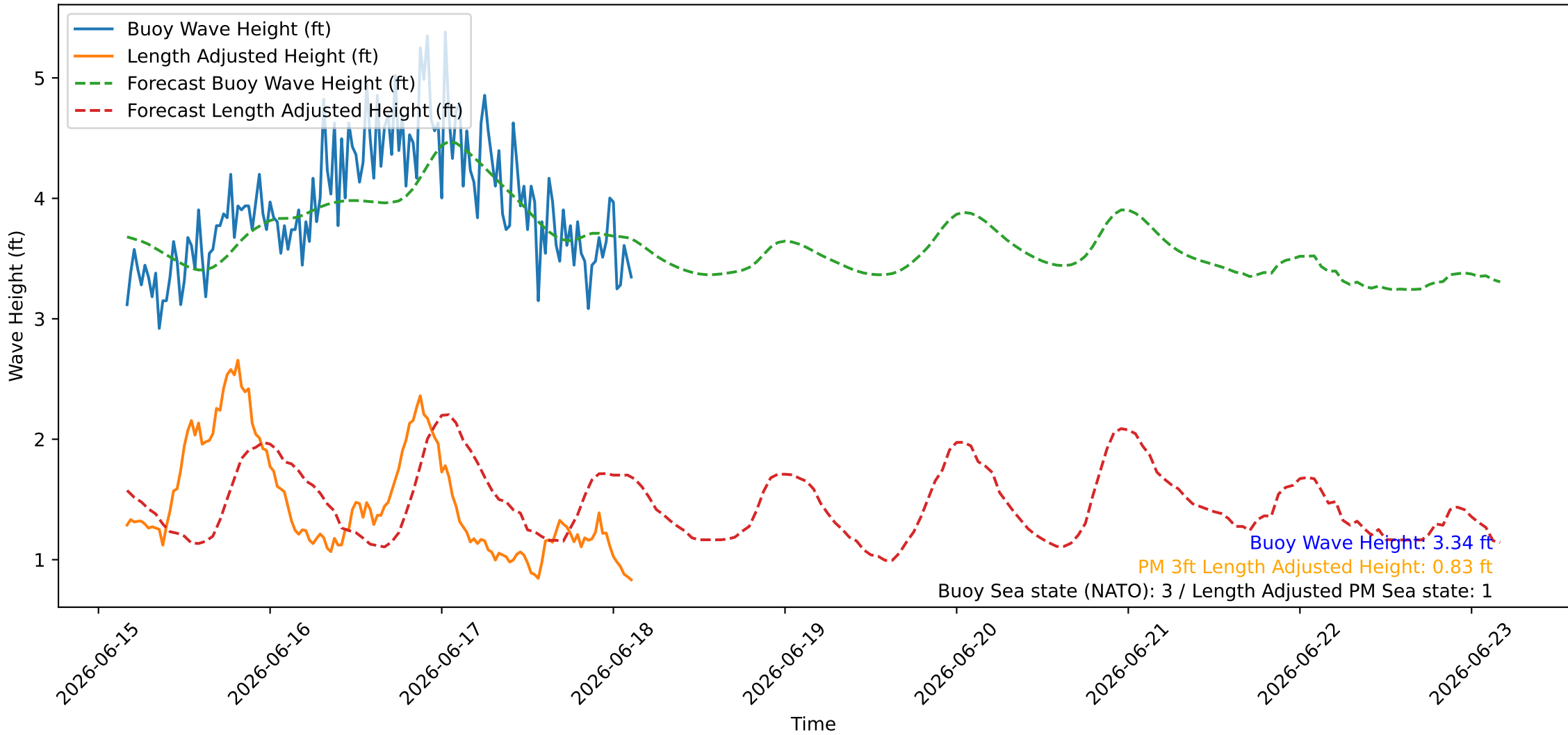
Wave Heights over Time for Red Beach at 2026-06-18 03:30:47
