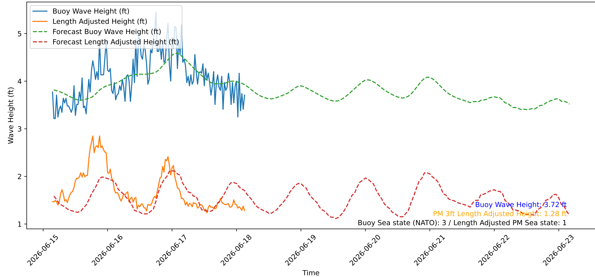
Wave Heights over Time for Oceanside Harbor at 2026-06-18 03:30:27
