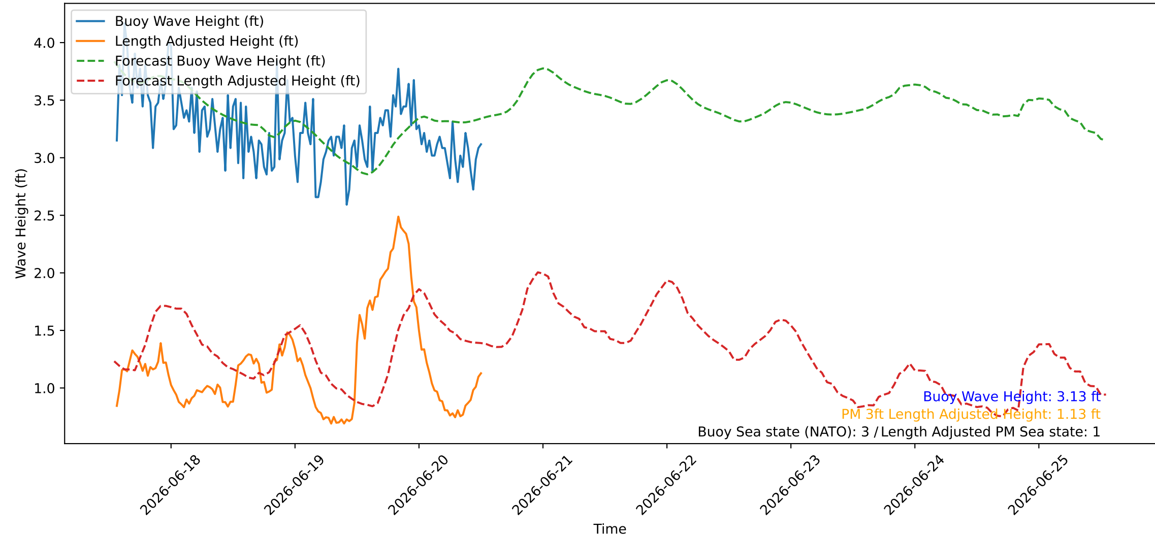
Wave Heights over Time for Red Beach at 2026-06-20 13:00:45
