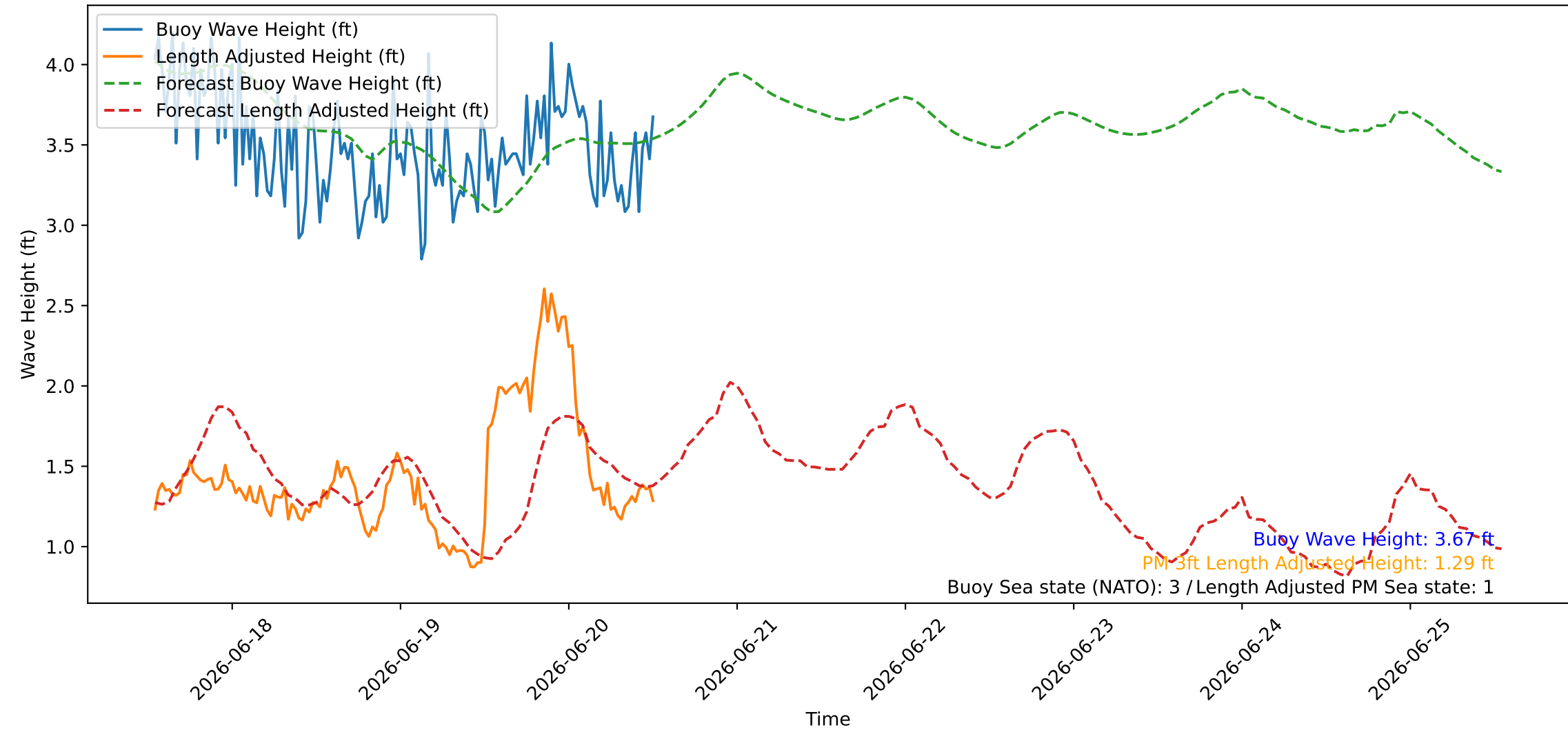
Wave Heights over Time for Oceanside Harbor at 2026-06-20 13:00:26
