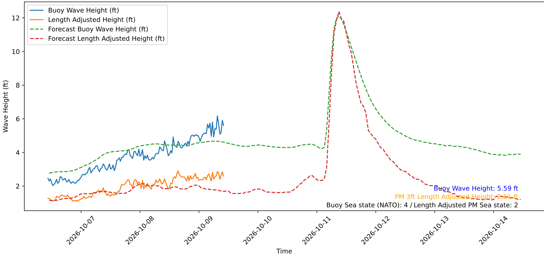
Wave Heights over Time for Oceanside Harbor at 2026-10-09 10:40:29
