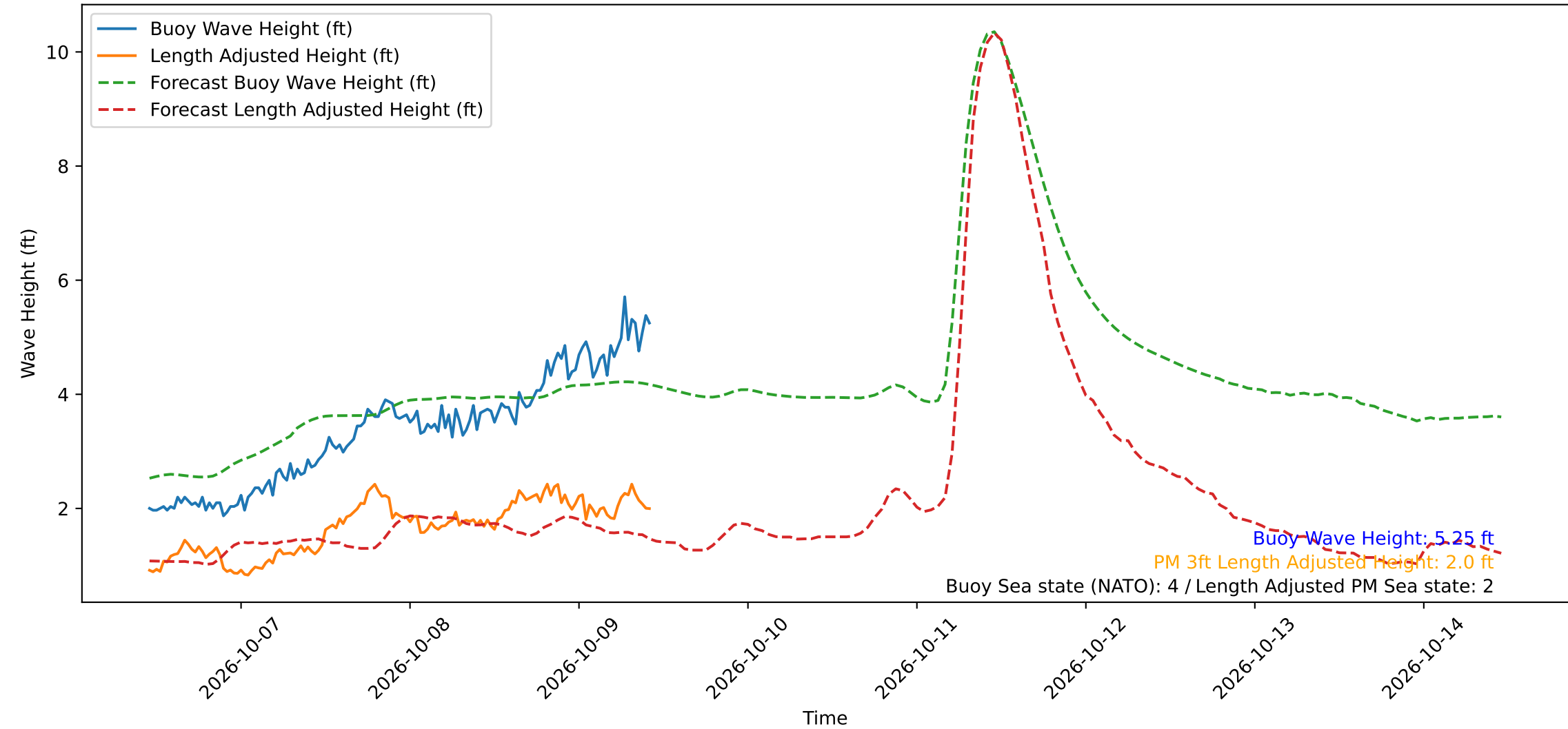
Wave Heights over Time for Red Beach at 2026-10-09 10:40:48
