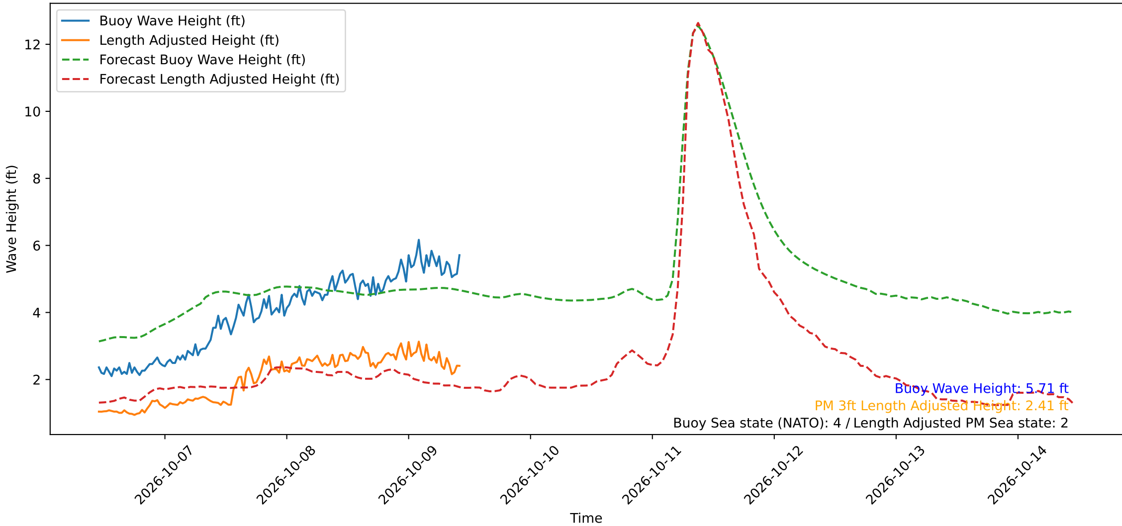
Wave Heights over Time for Green Beach at 2026-10-09 10:41:10
