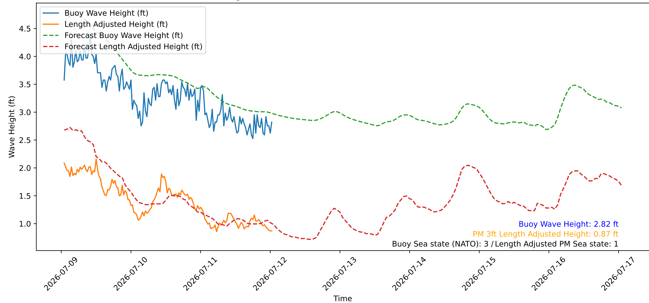
Wave Heights over Time for Green Beach at 2026-07-12 01:11:07
