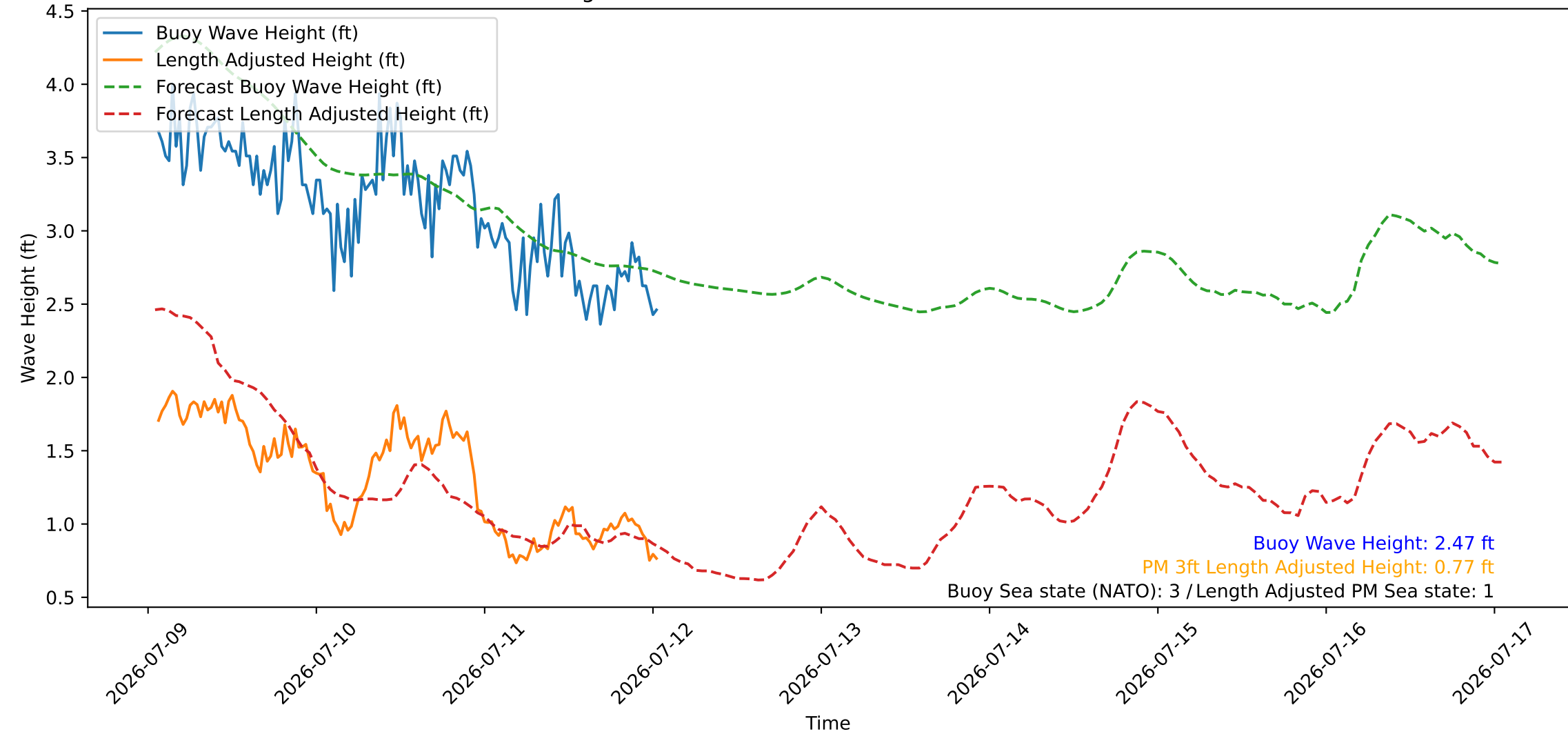
Wave Heights over Time for Red Beach at 2026-07-12 01:10:45
