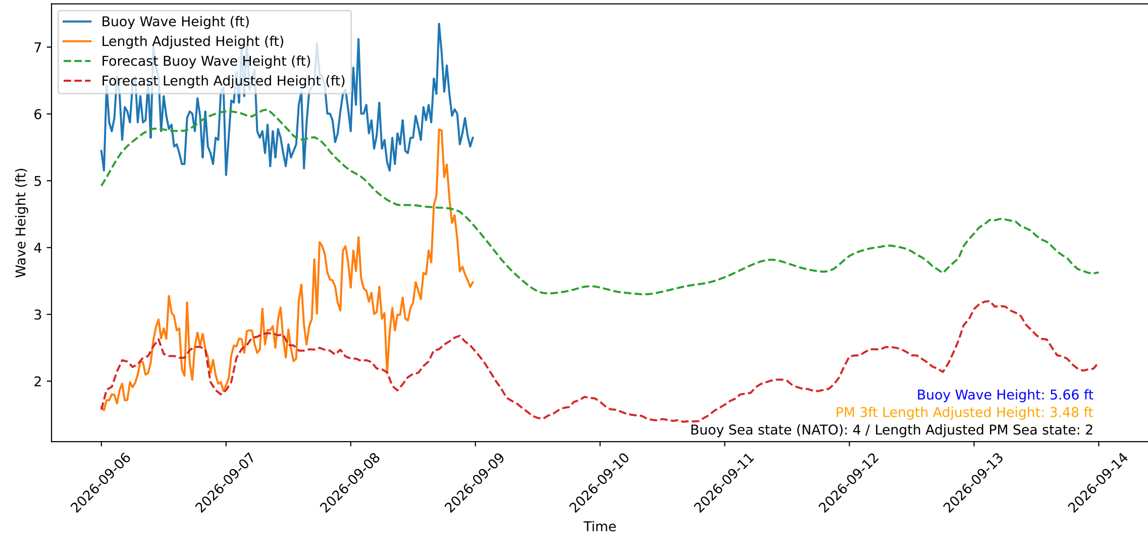
Wave Heights over Time for Oceanside Harbor at 2026-09-09 00:00:30
