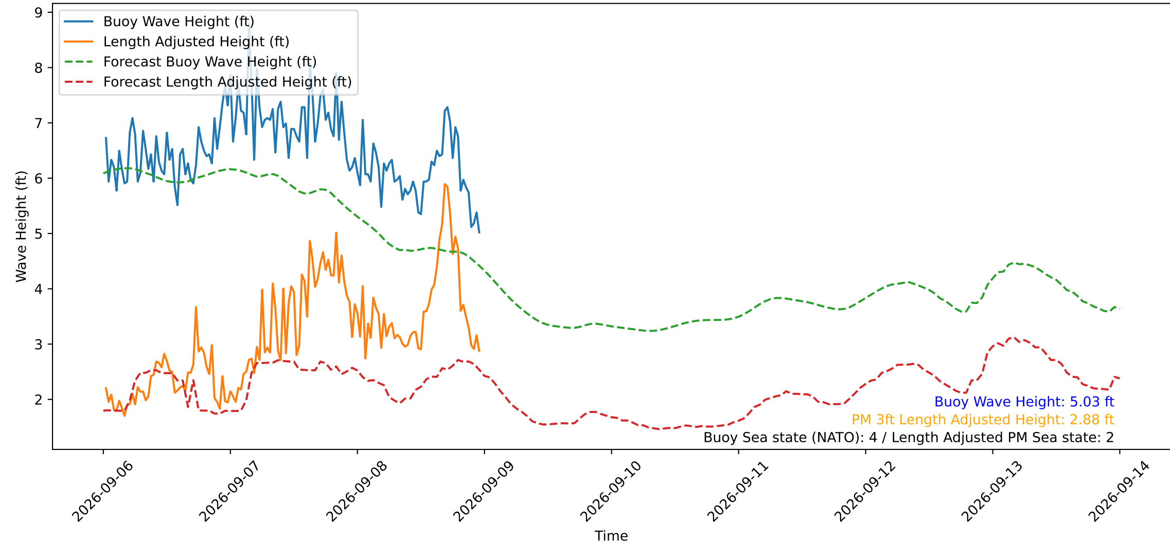
Wave Heights over Time for Green Beach at 2026-09-09 00:01:12
