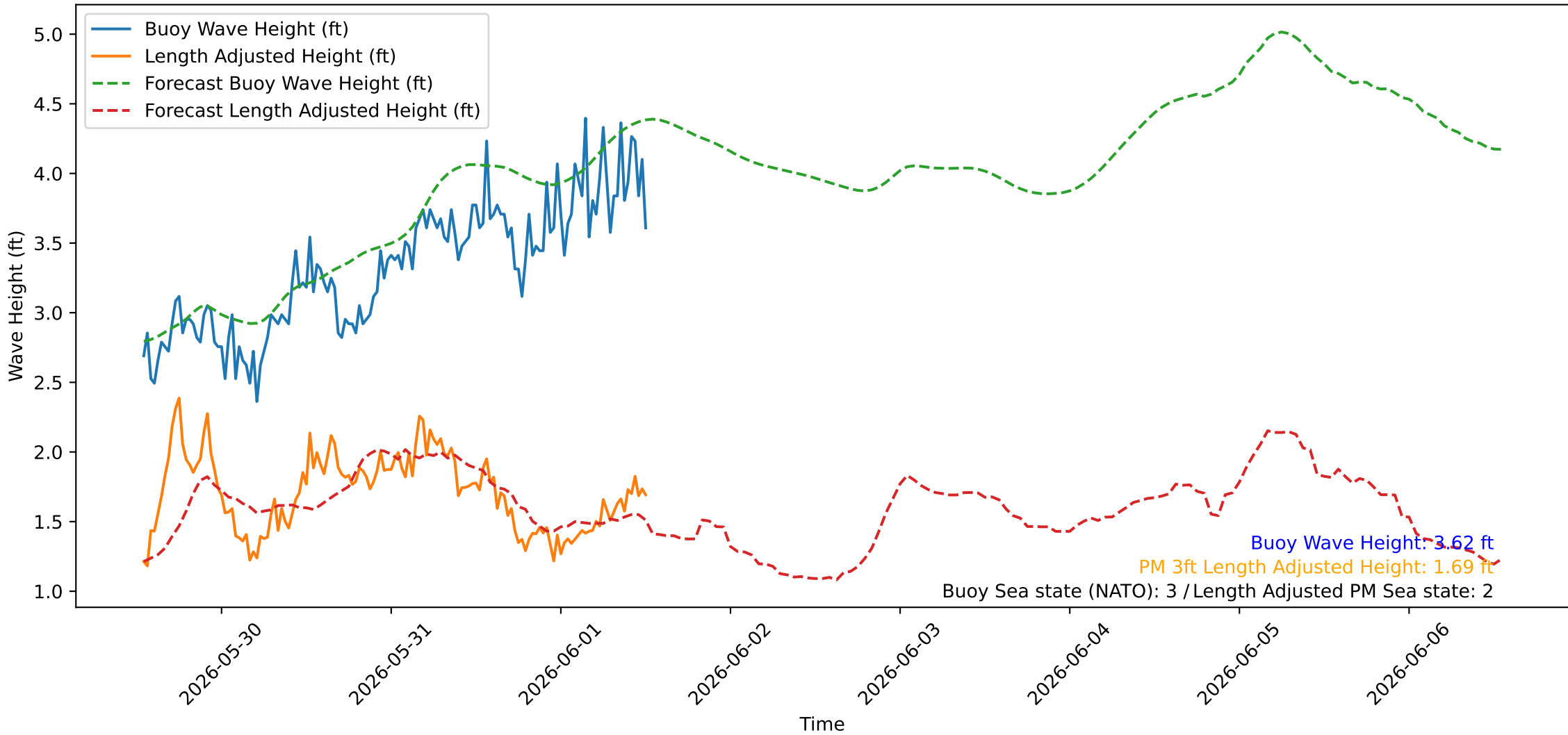
Wave Heights over Time for Oceanside Harbor at 2026-06-01 12:50:26
