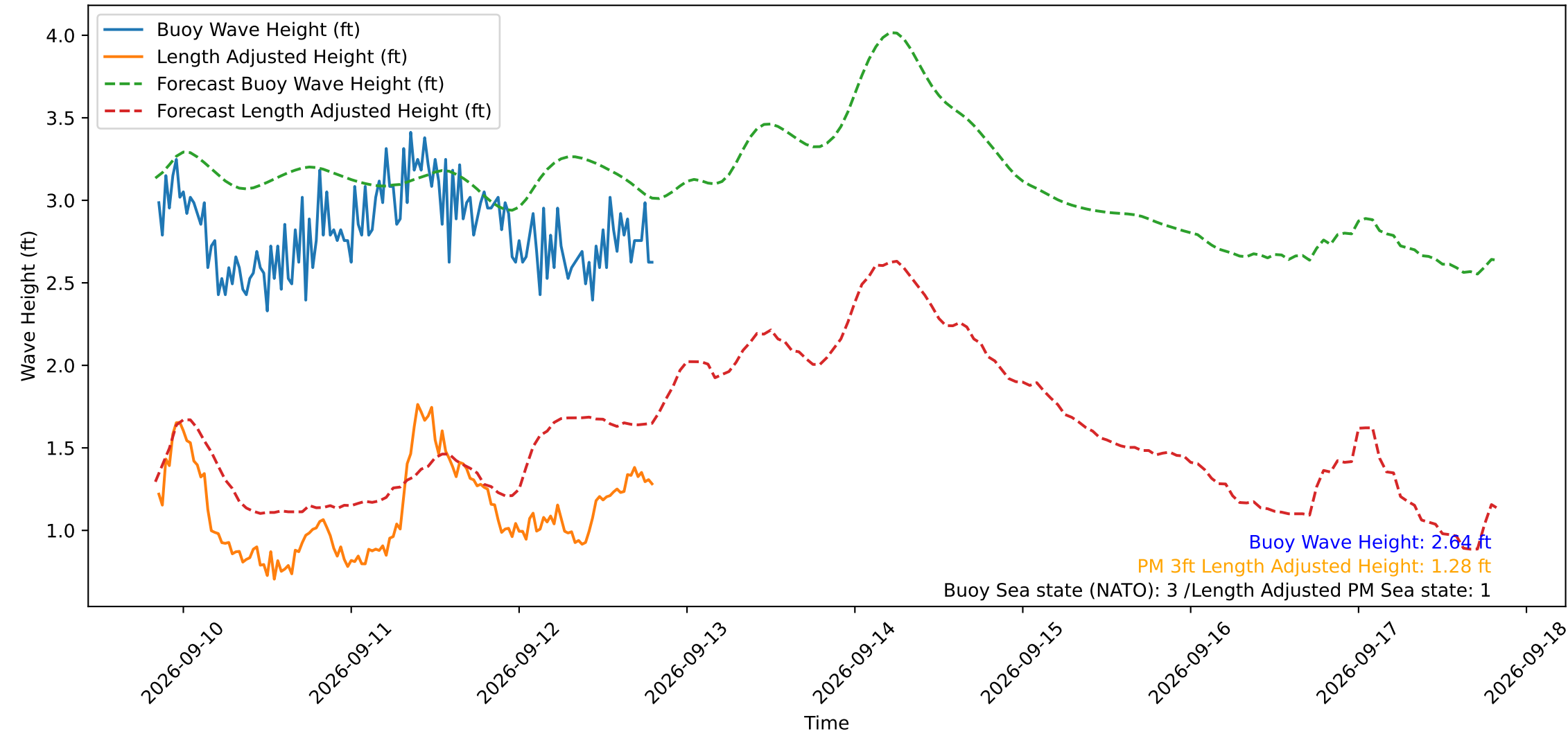
Wave Heights over Time for Red Beach at 2026-09-12 20:00:49
