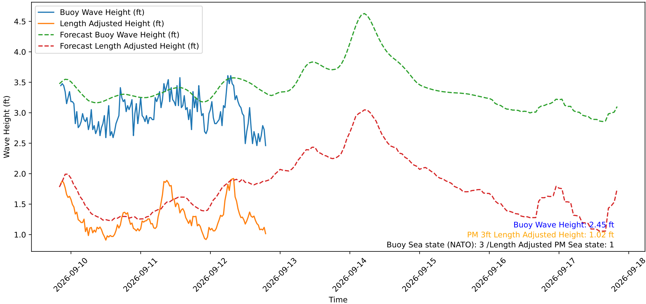
Wave Heights over Time for Green Beach at 2026-09-12 20:01:11
