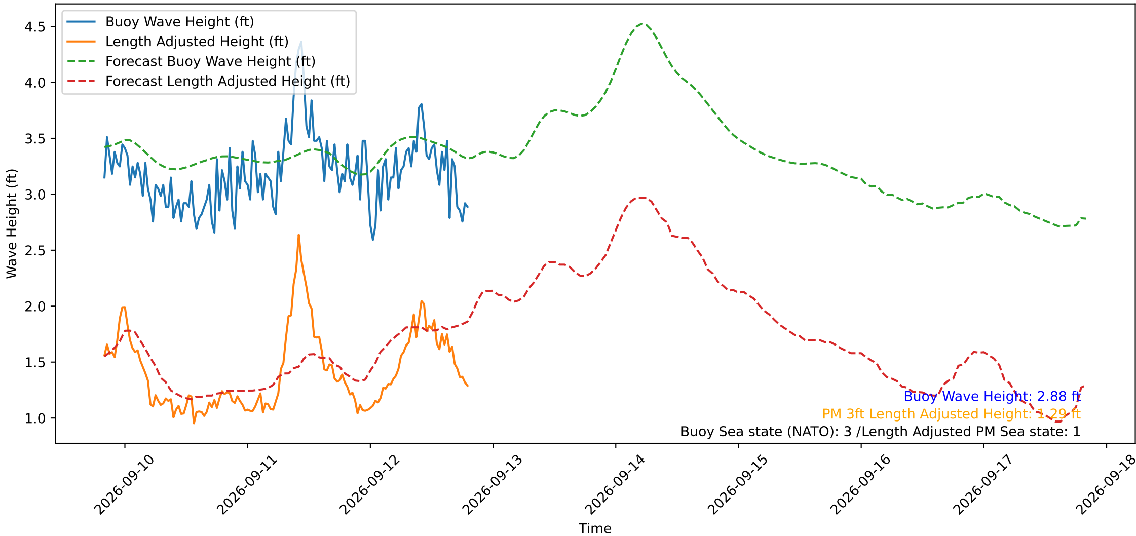
Wave Heights over Time for Oceanside Harbor at 2026-09-12 20:00:29
