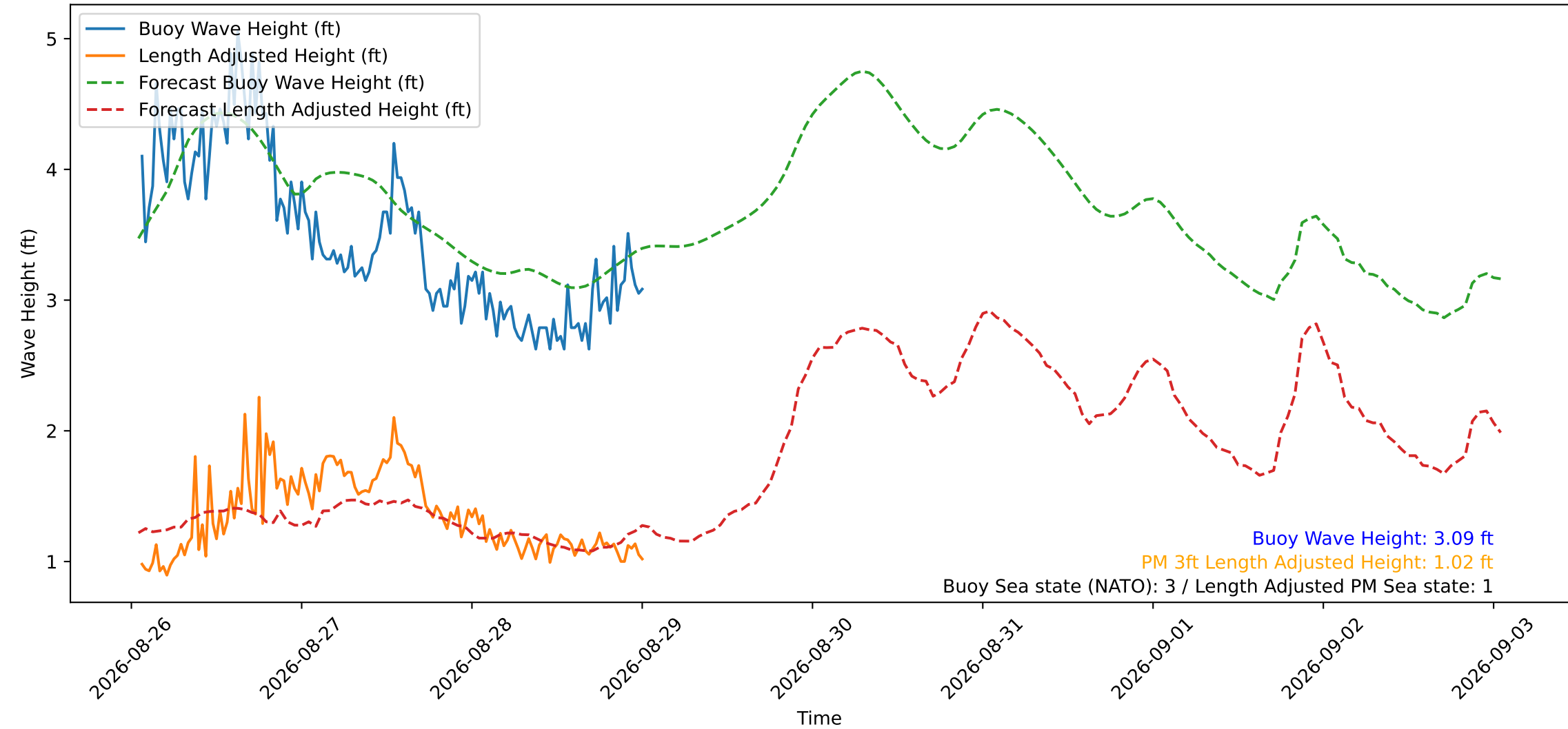
Wave Heights over Time for Red Beach at 2026-08-29 01:00:50
