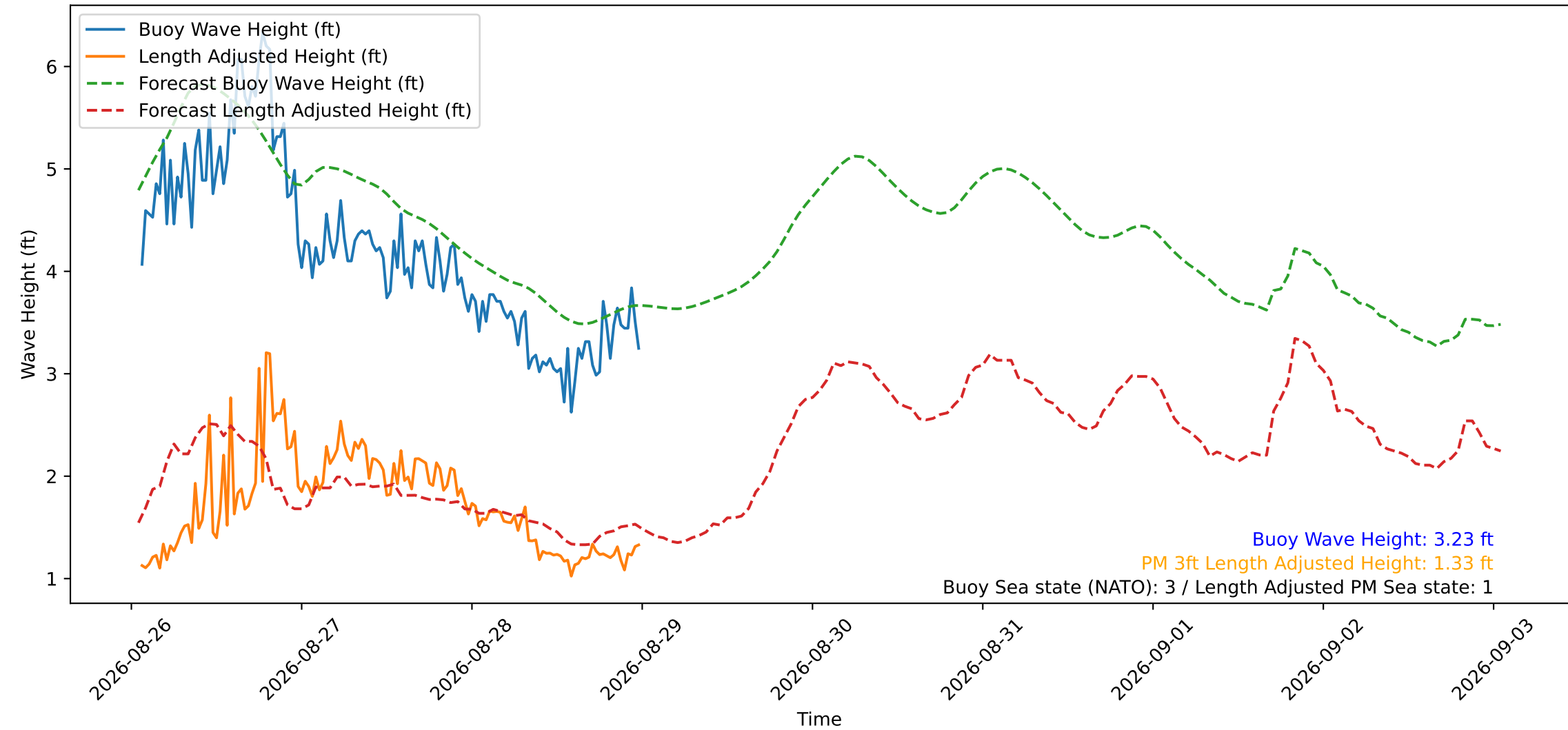
Wave Heights over Time for Green Beach at 2026-08-29 01:01:13
