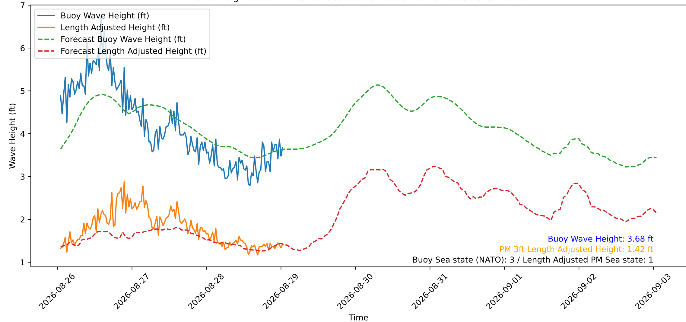
Wave Heights over Time for Oceanside Harbor at 2026-08-29 01:00:31
