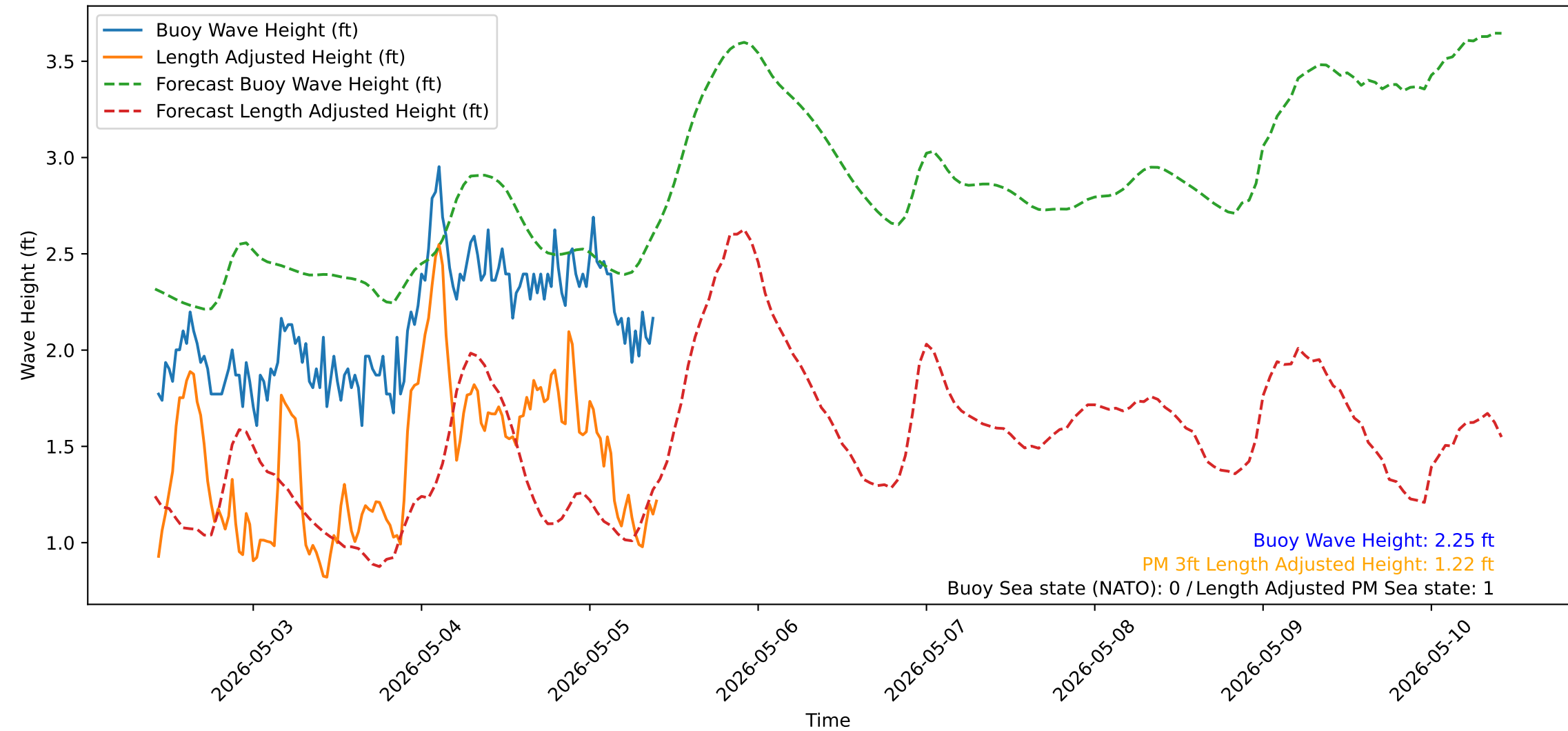
Wave Heights over Time for Red Beach at 2026-05-05 10:10:51
