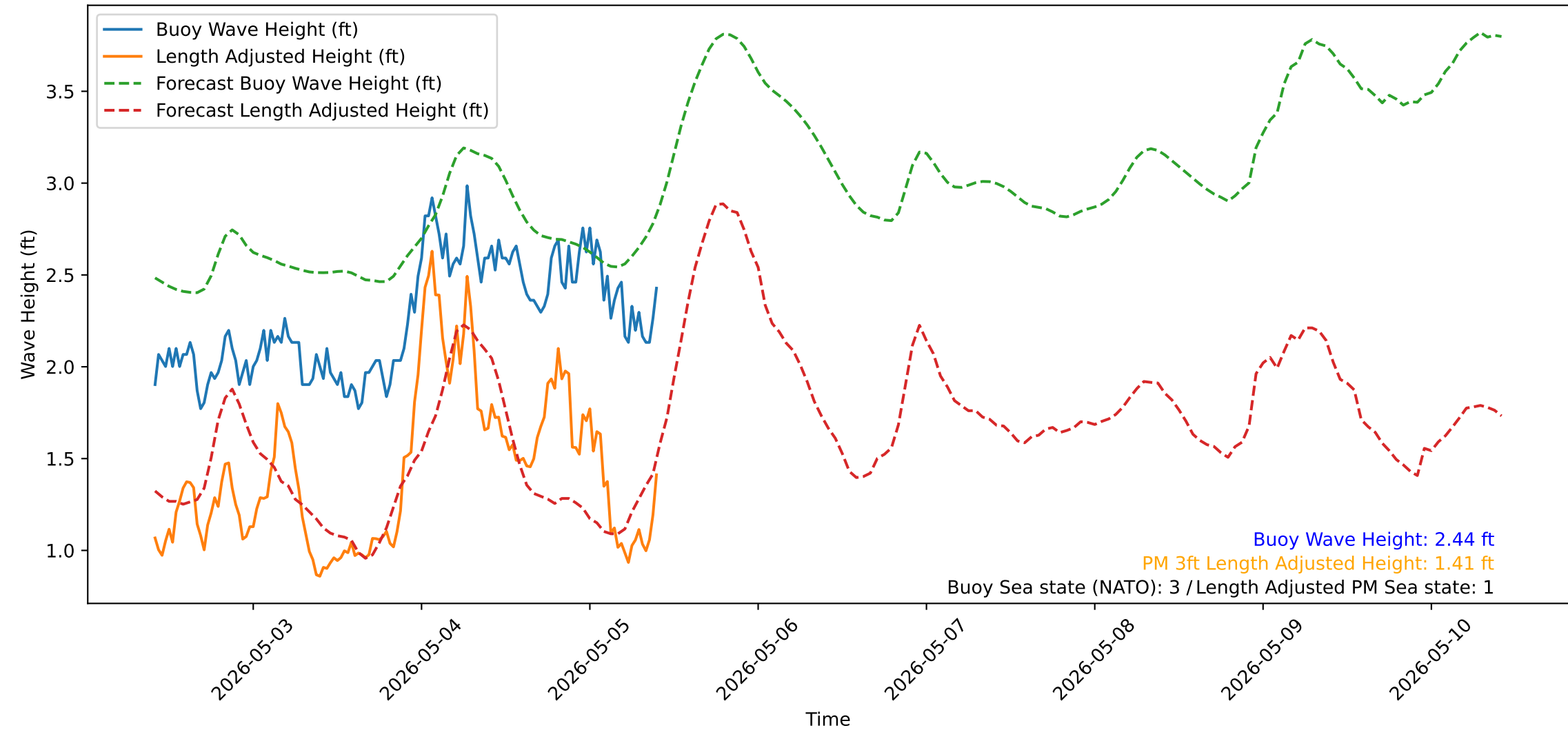
Wave Heights over Time for Green Beach at 2026-05-05 10:11:13
