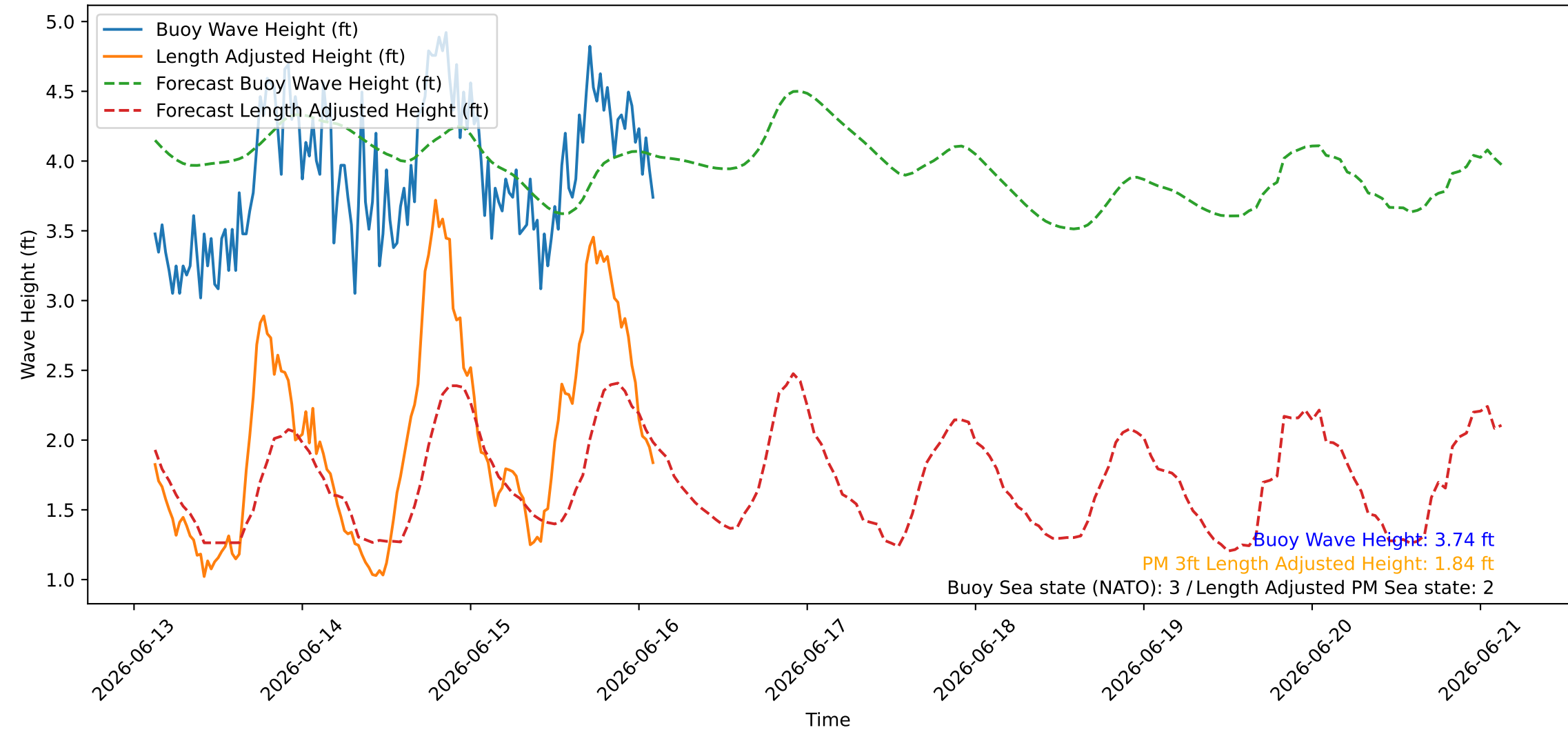
Wave Heights over Time for Green Beach at 2026-06-16 02:51:09
