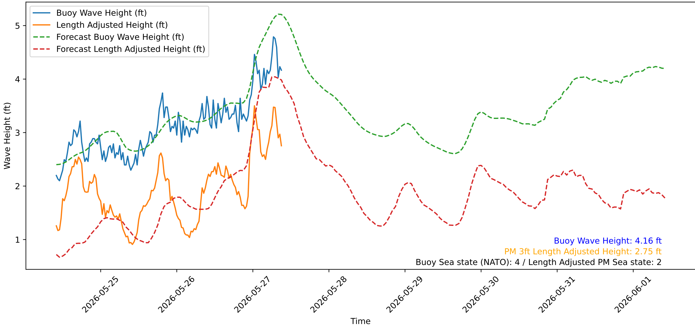
Wave Heights over Time for Red Beach at 2026-05-27 09:50:47
