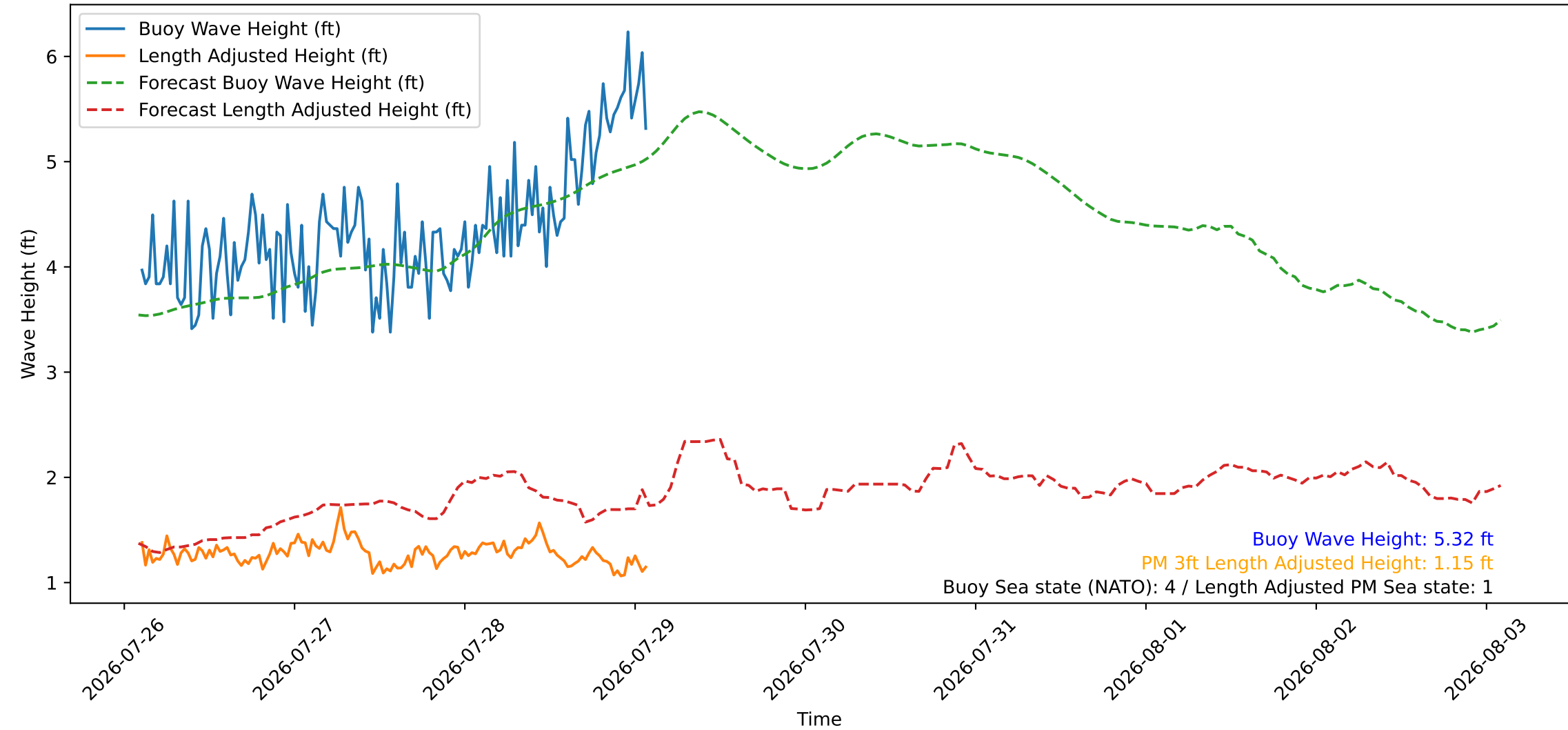
Wave Heights over Time for Green Beach at 2026-07-29 02:21:10
