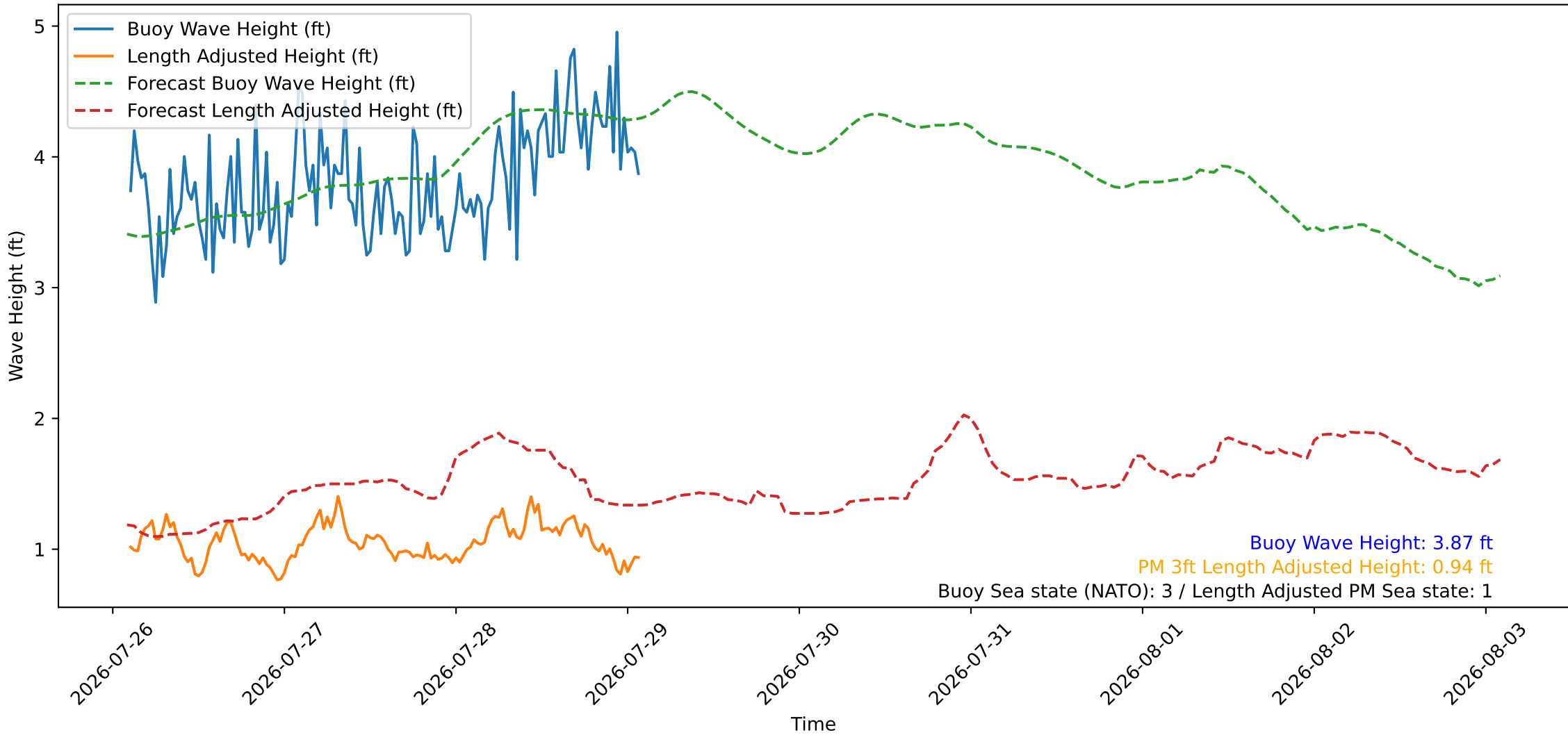
Wave Heights over Time for Red Beach at 2026-07-29 02:20:48
