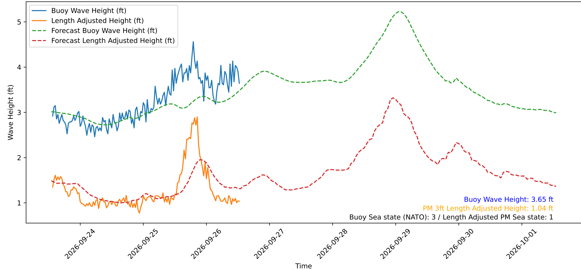
Wave Heights over Time for Green Beach at 2026-09-26 13:21:14
