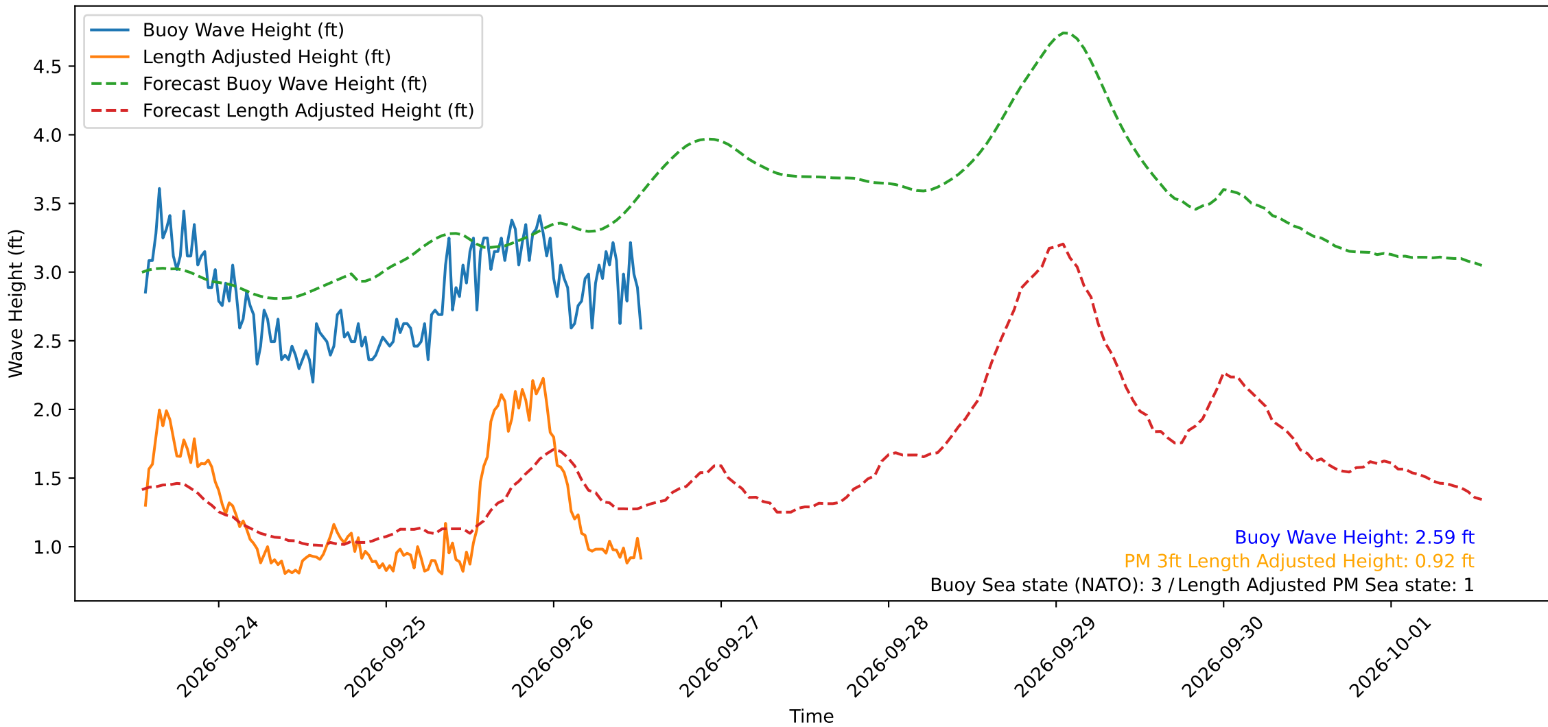
Wave Heights over Time for Oceanside Harbor at 2026-09-26 13:20:29
