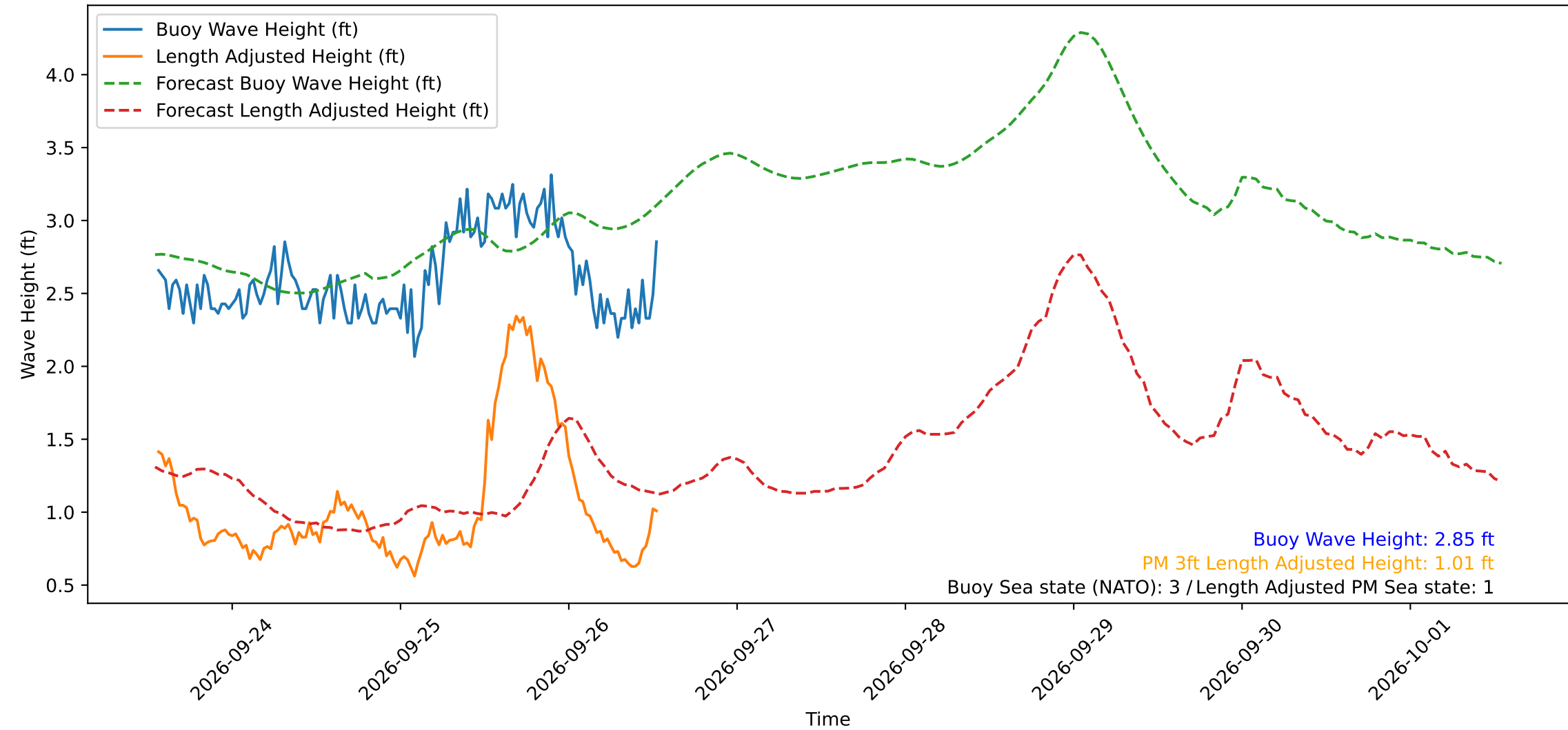
Wave Heights over Time for Red Beach at 2026-09-26 13:20:50
