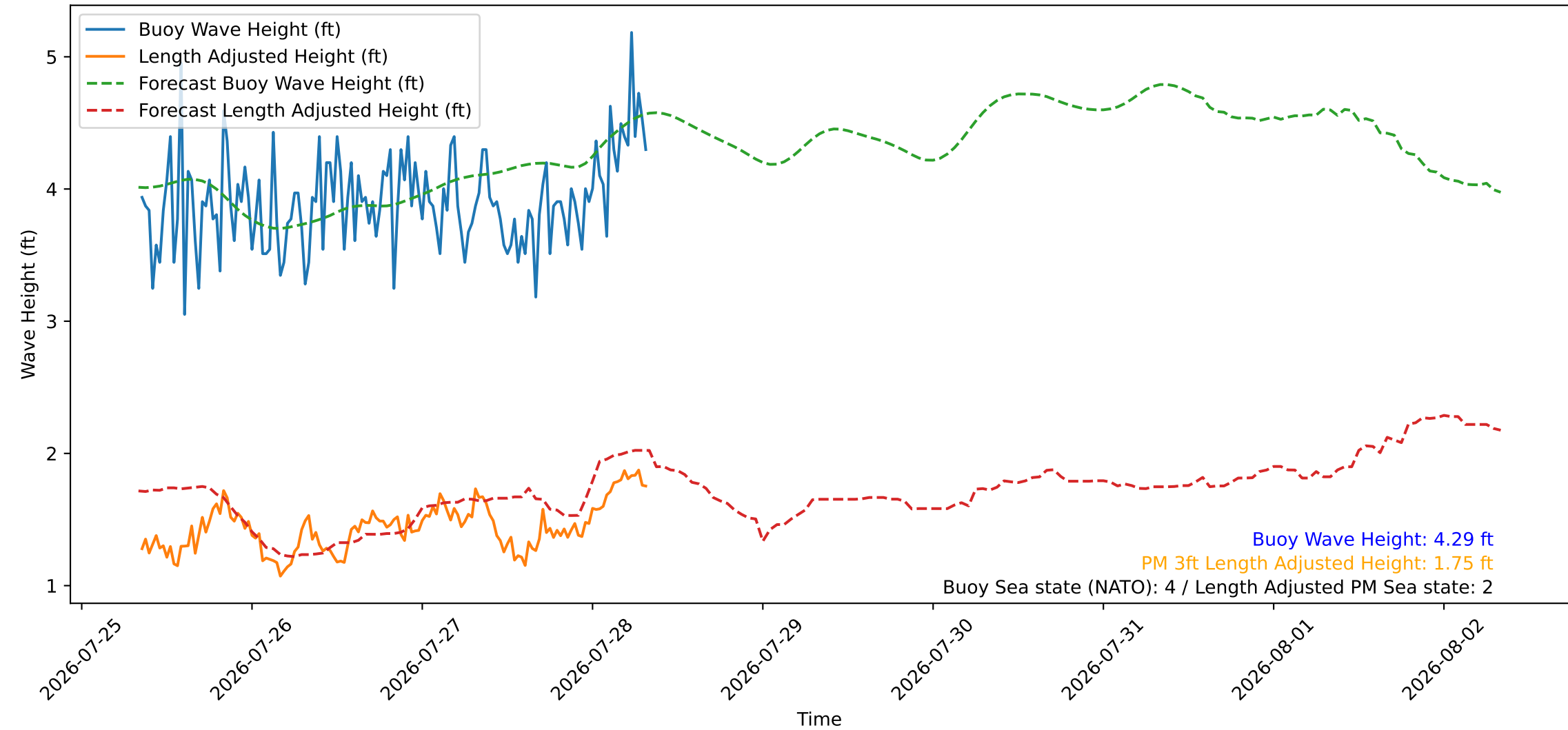
Wave Heights over Time for Oceanside Harbor at 2026-07-28 08:20:27
