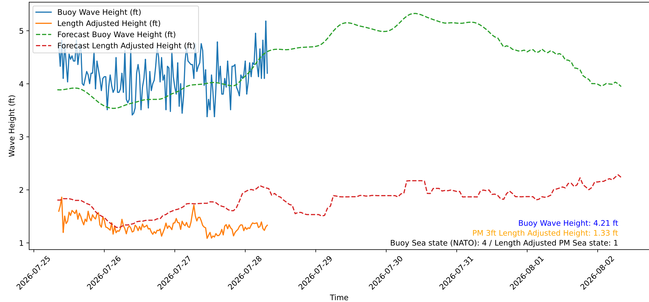
Wave Heights over Time for Green Beach at 2026-07-28 08:21:11
