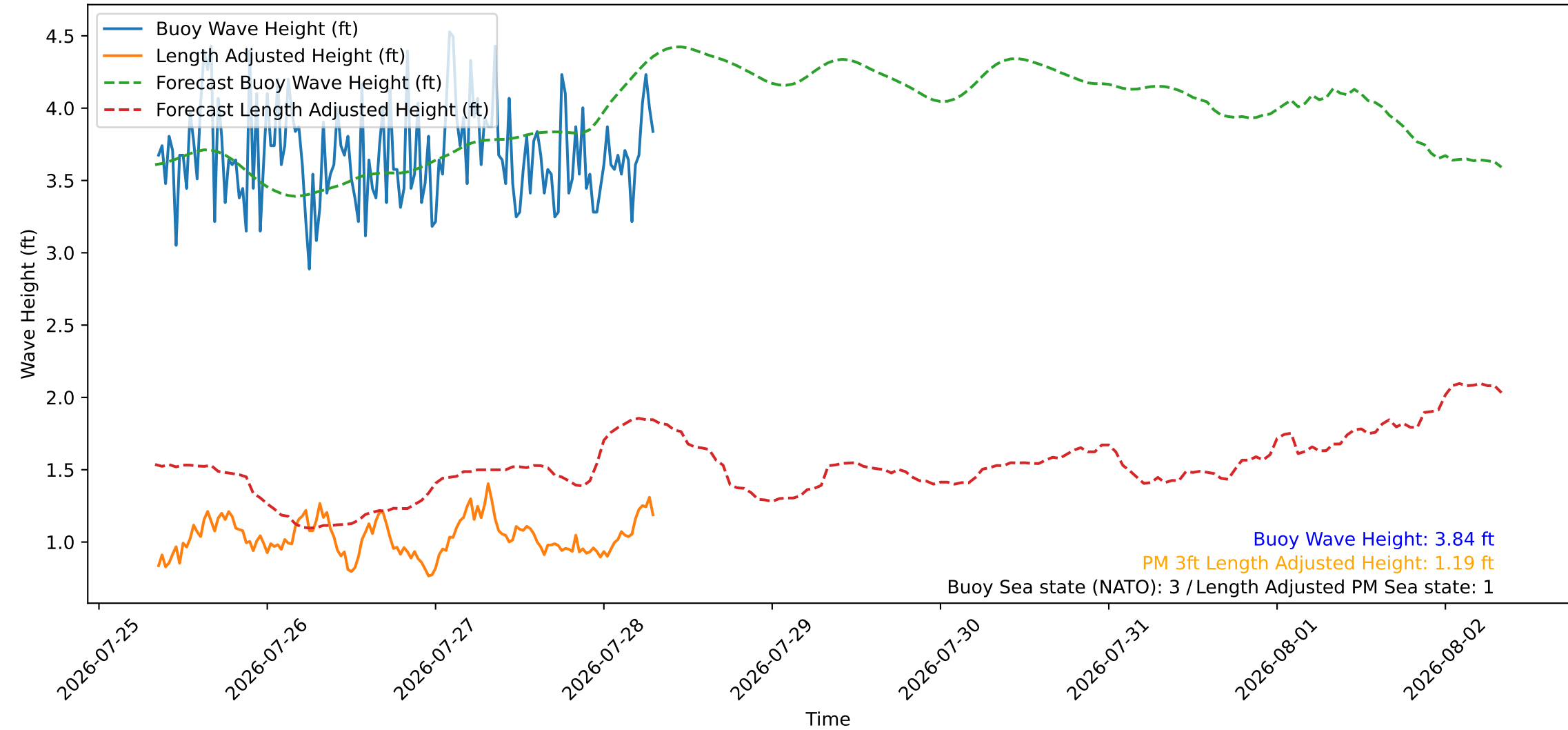
Wave Heights over Time for Red Beach at 2026-07-28 08:20:48
