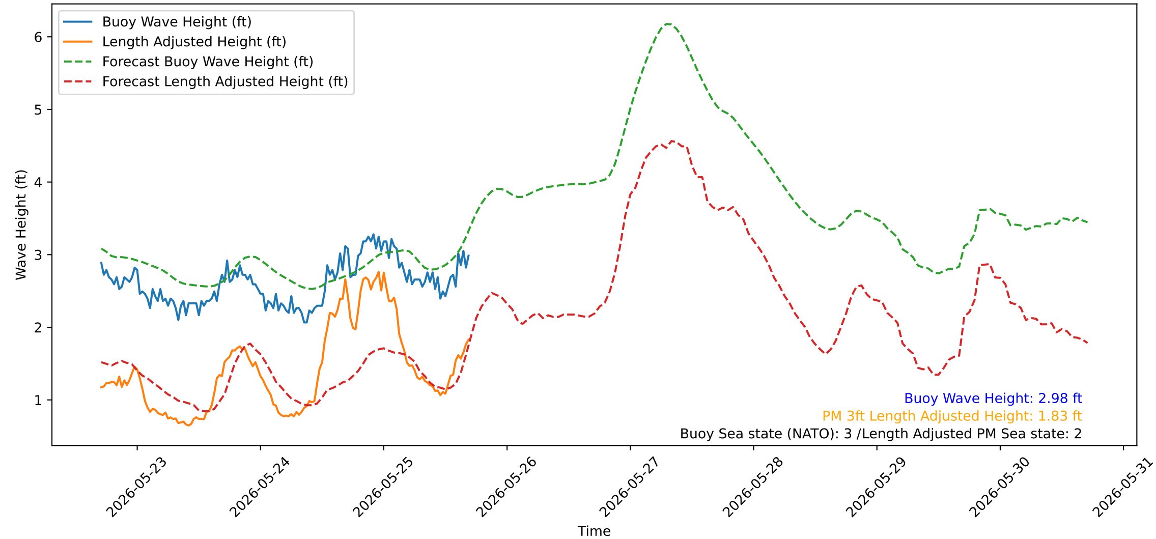
Wave Heights over Time for Green Beach at 2026-05-25 17:11:12
