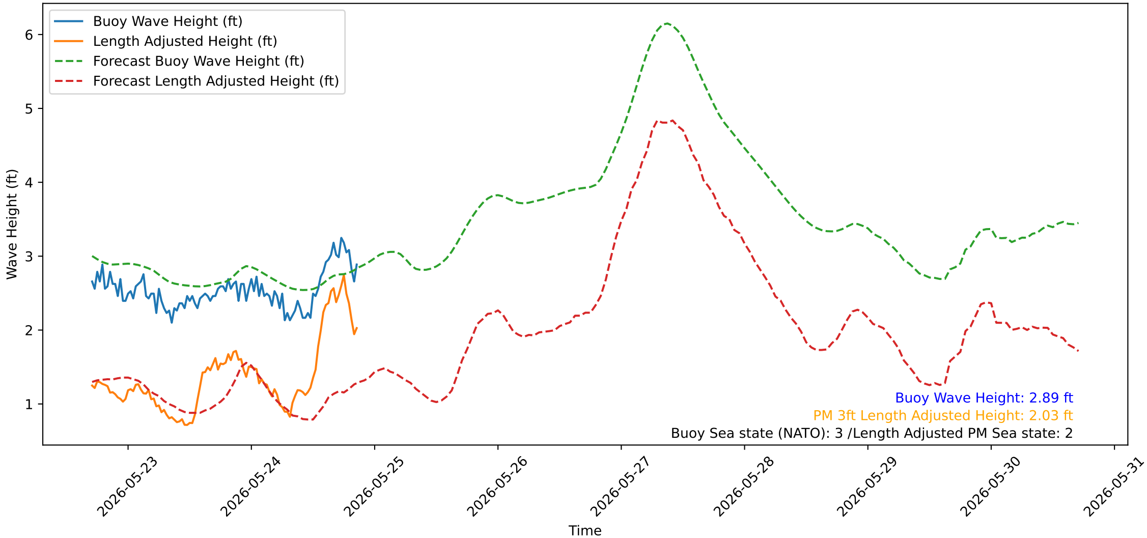
Wave Heights over Time for Oceanside Harbor at 2026-05-25 17:10:30
