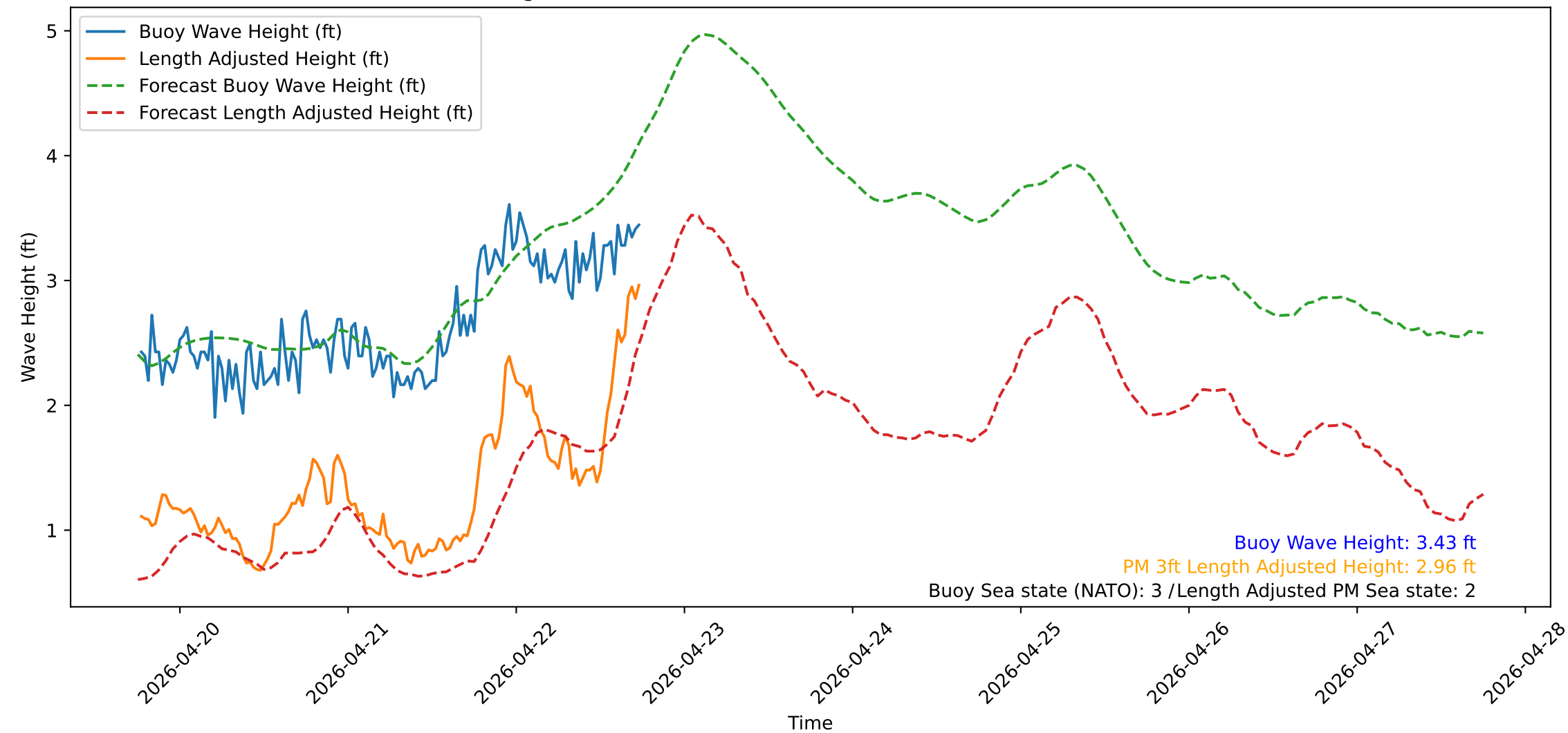
Wave Heights over Time for Oceanside Harbor at 2026-04-22 18:20:31
