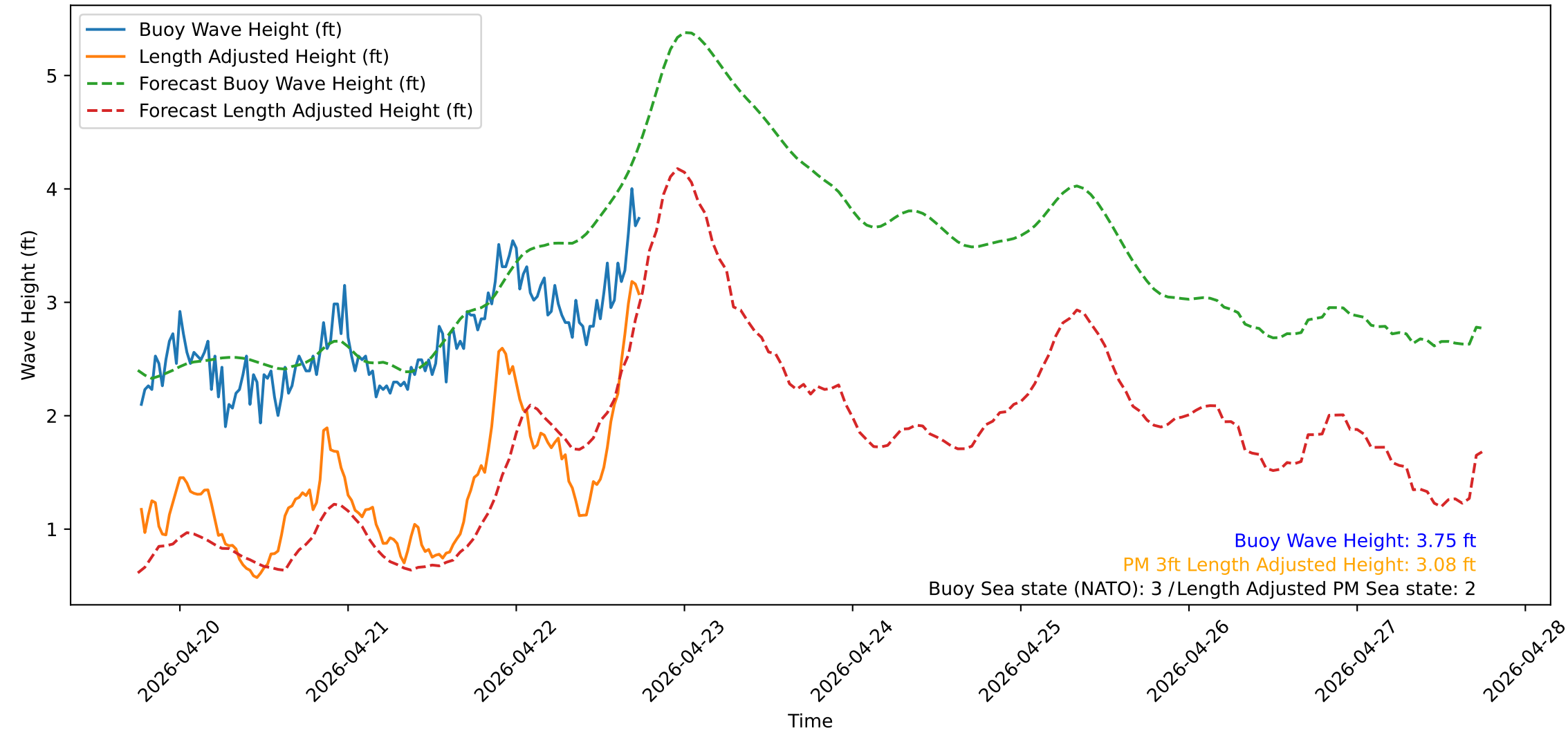
Wave Heights over Time for Green Beach at 2026-04-22 18:21:14
