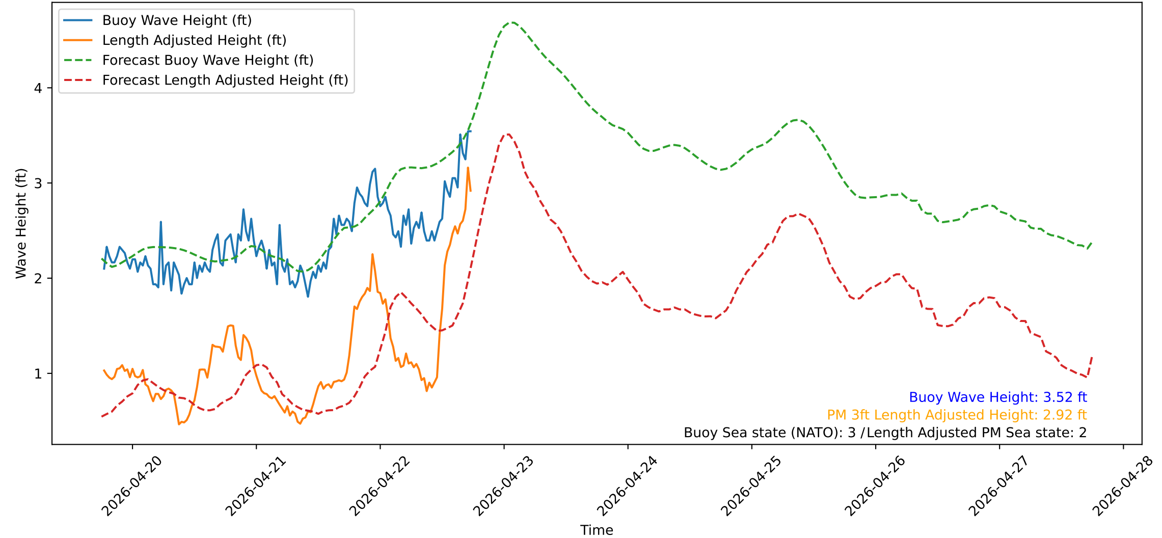
Wave Heights over Time for Red Beach at 2026-04-22 18:20:52
