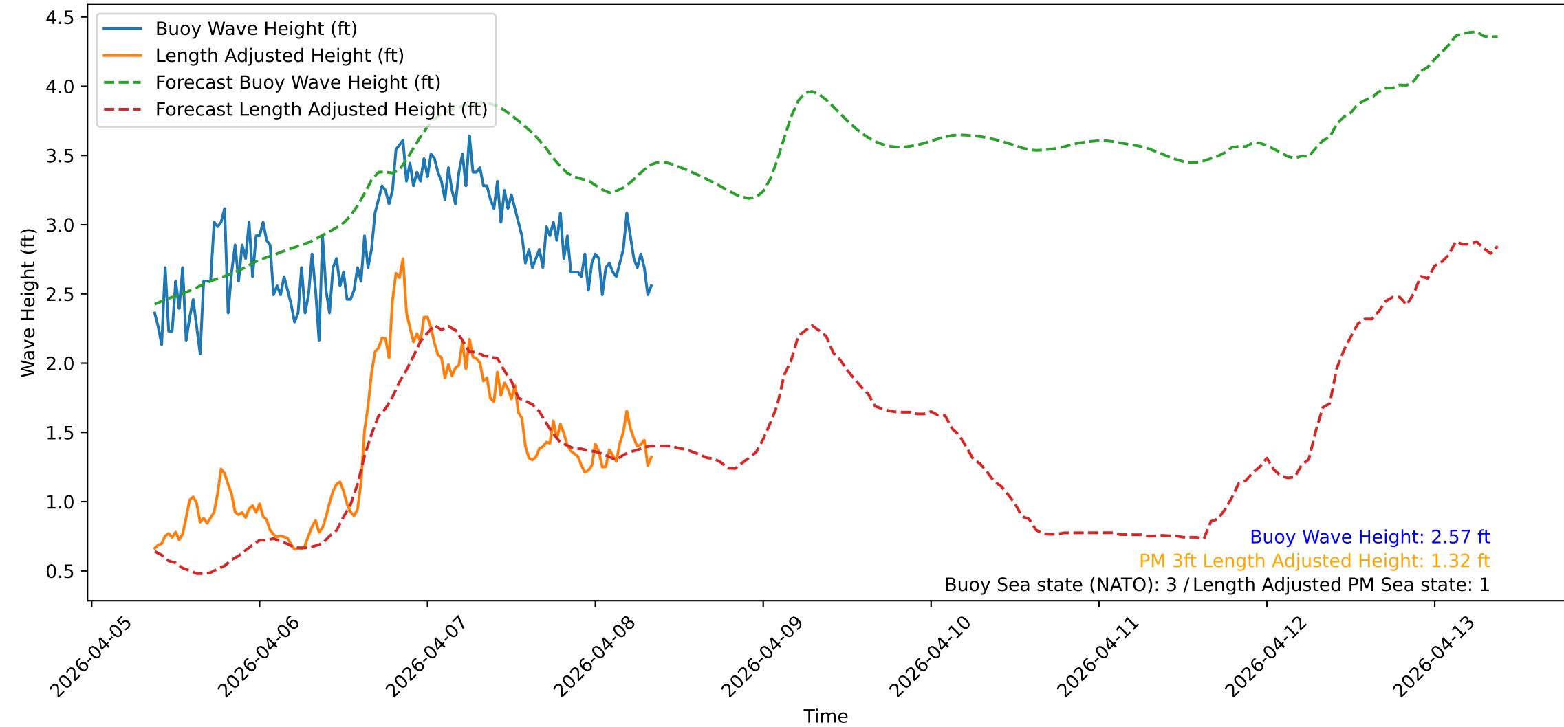
Wave Heights over Time for Oceanside Harbor at 2026-04-08 08:50:32
