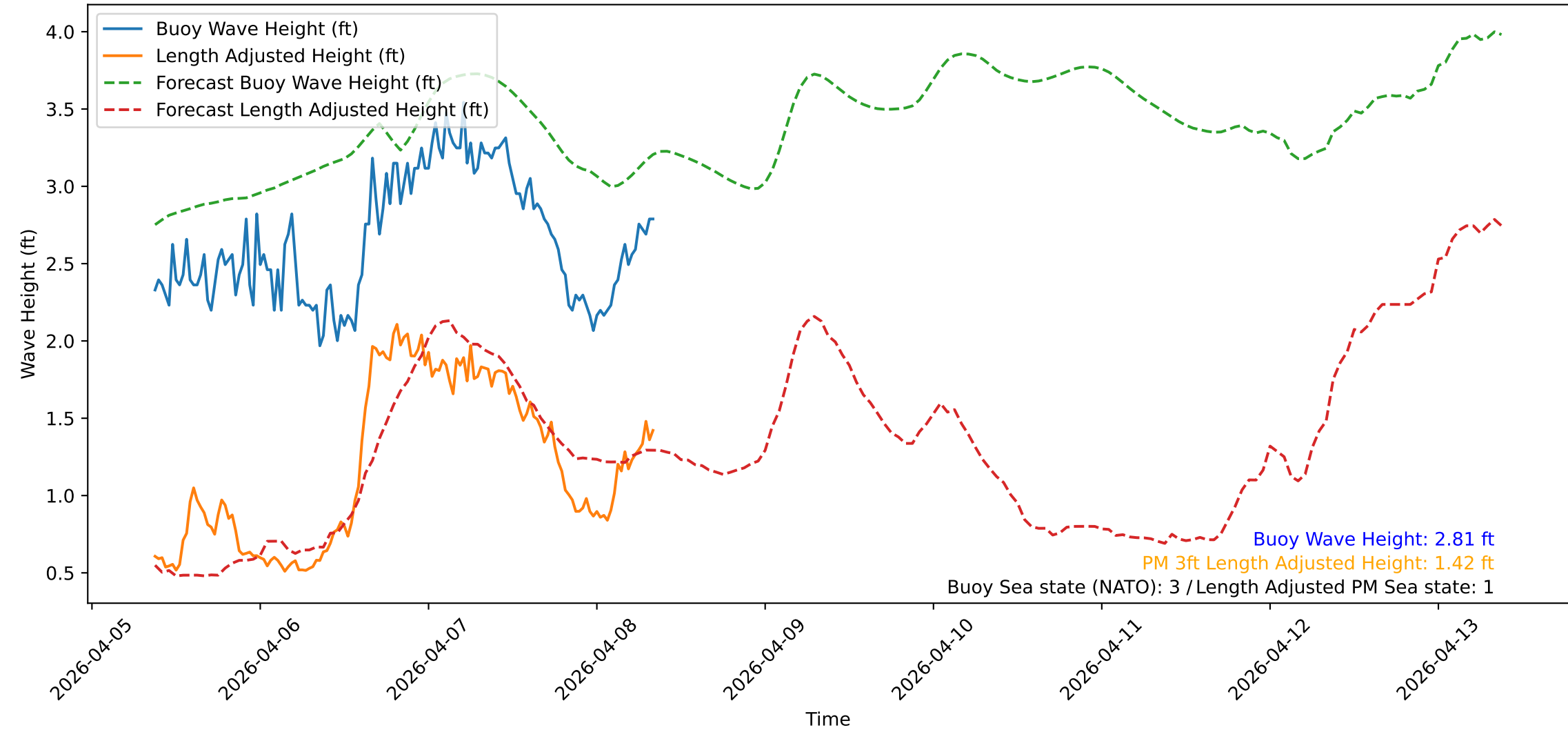
Wave Heights over Time for Red Beach at 2026-04-08 08:50:49
