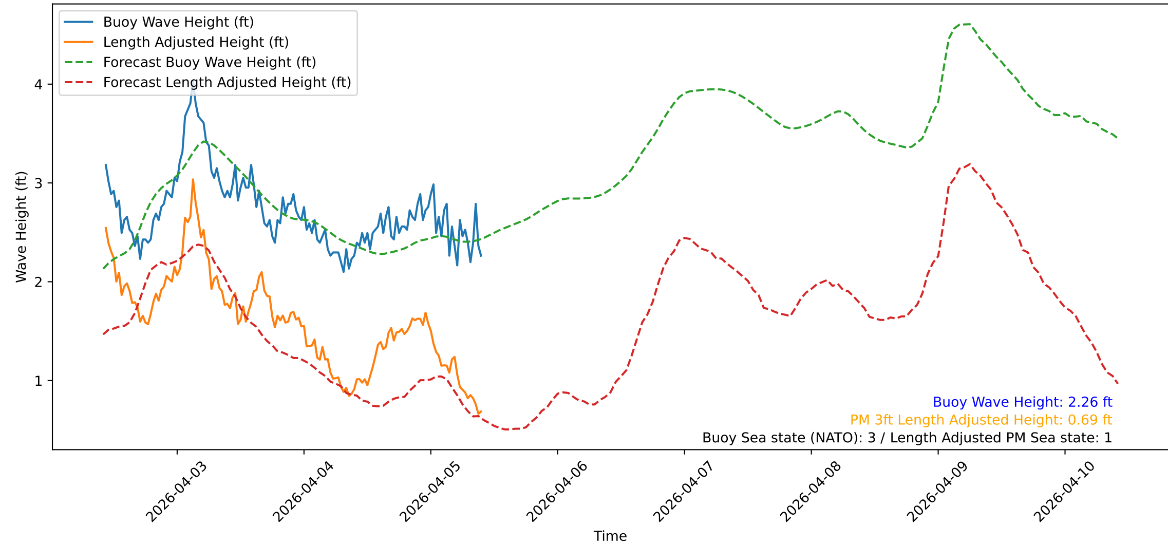
Wave Heights over Time for Oceanside Harbor at 2026-04-05 10:20:31
