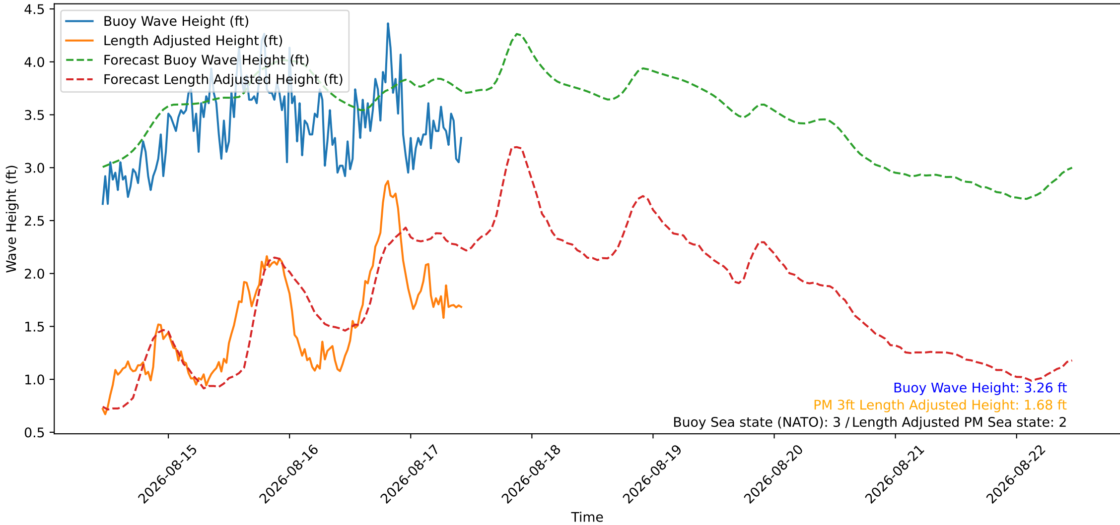
Wave Heights over Time for Green Beach at 2026-08-17 10:41:09
