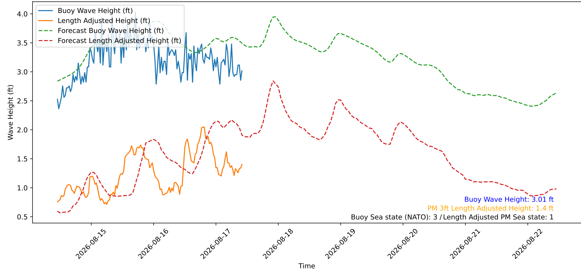
Wave Heights over Time for Red Beach at 2026-08-17 10:40:46
