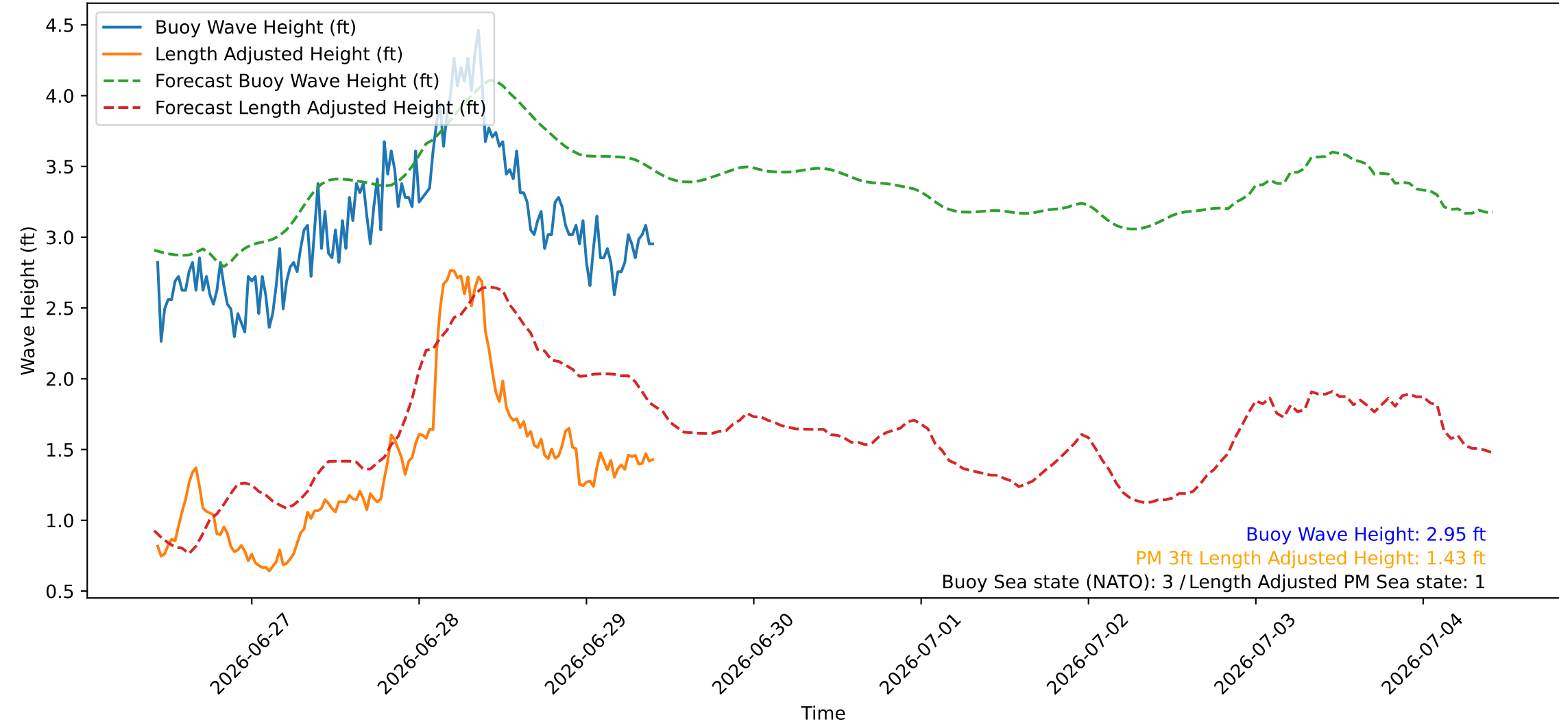
Wave Heights over Time for Red Beach at 2026-06-29 10:20:46
