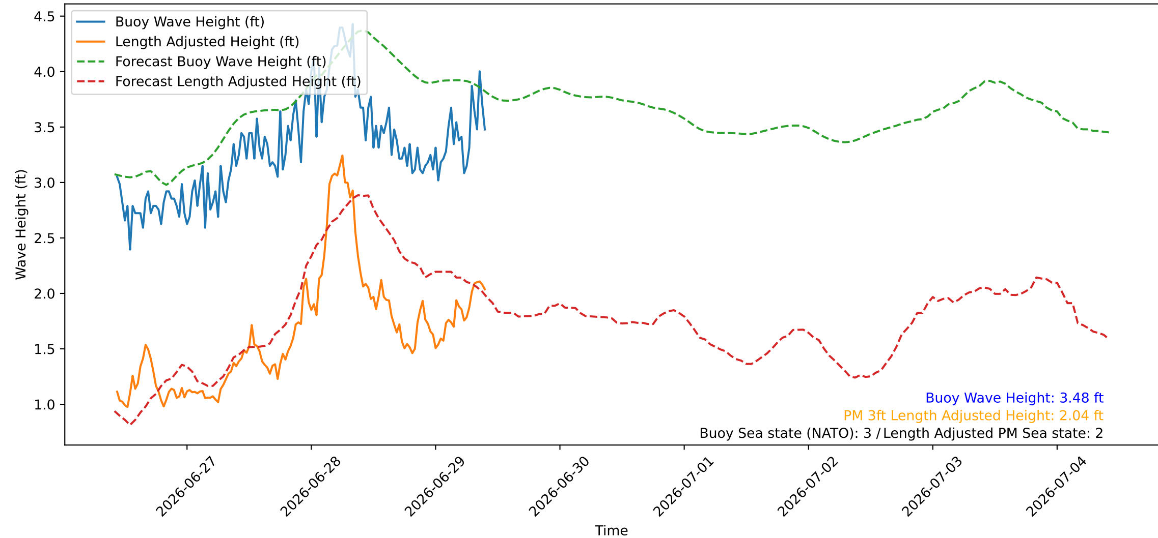
Wave Heights over Time for Oceanside Harbor at 2026-06-29 10:20:26
