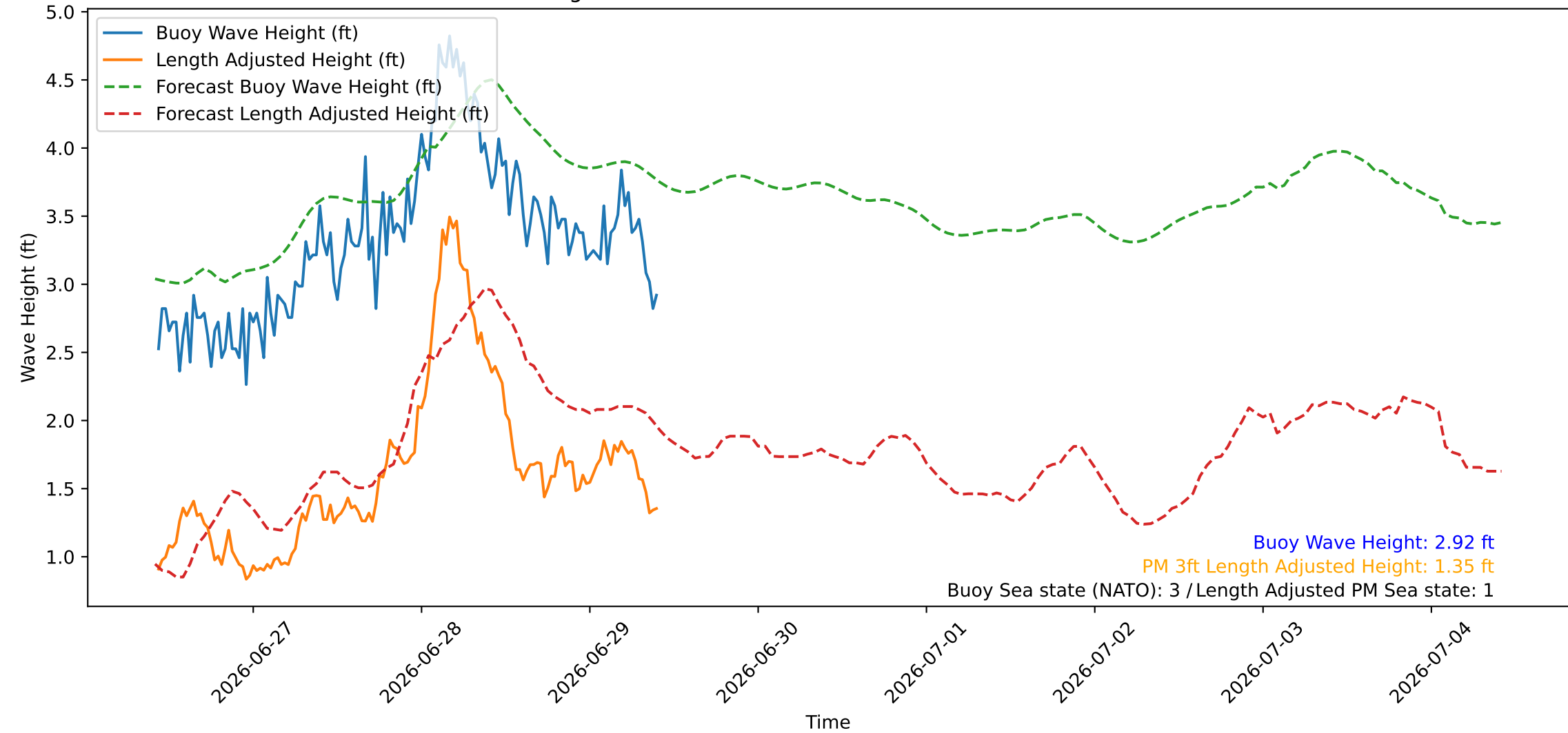
Wave Heights over Time for Green Beach at 2026-06-29 10:21:08
