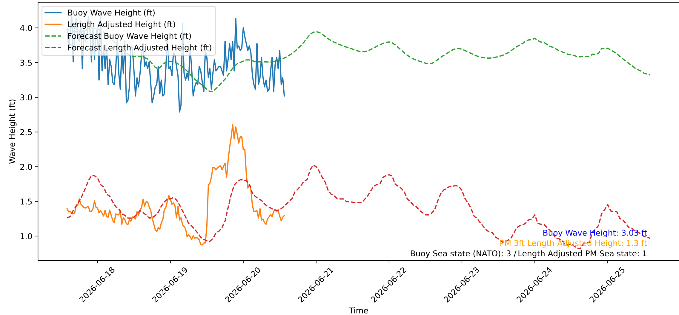
Wave Heights over Time for Oceanside Harbor at 2026-06-20 14:00:26
