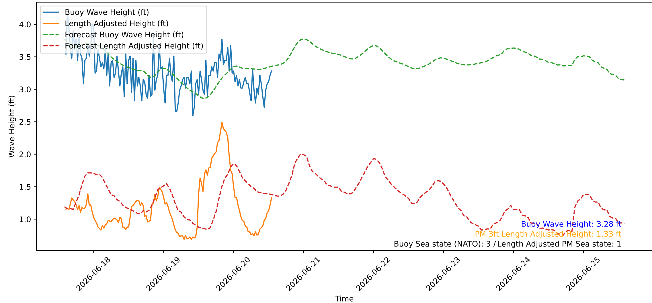
Wave Heights over Time for Red Beach at 2026-06-20 14:00:45
