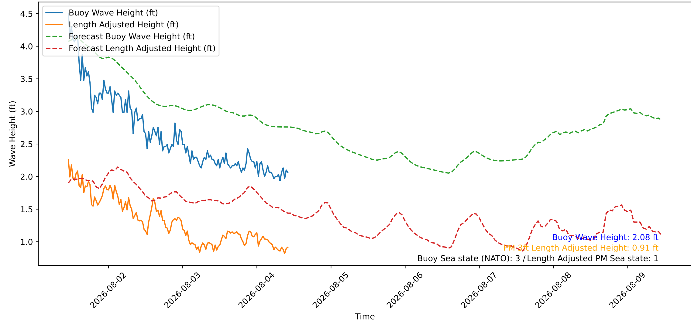
Wave Heights over Time for Green Beach at 2026-08-04 10:51:09
