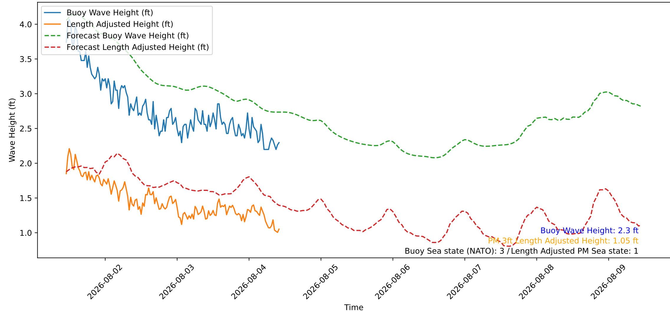
Wave Heights over Time for Oceanside Harbor at 2026-08-04 10:50:26
