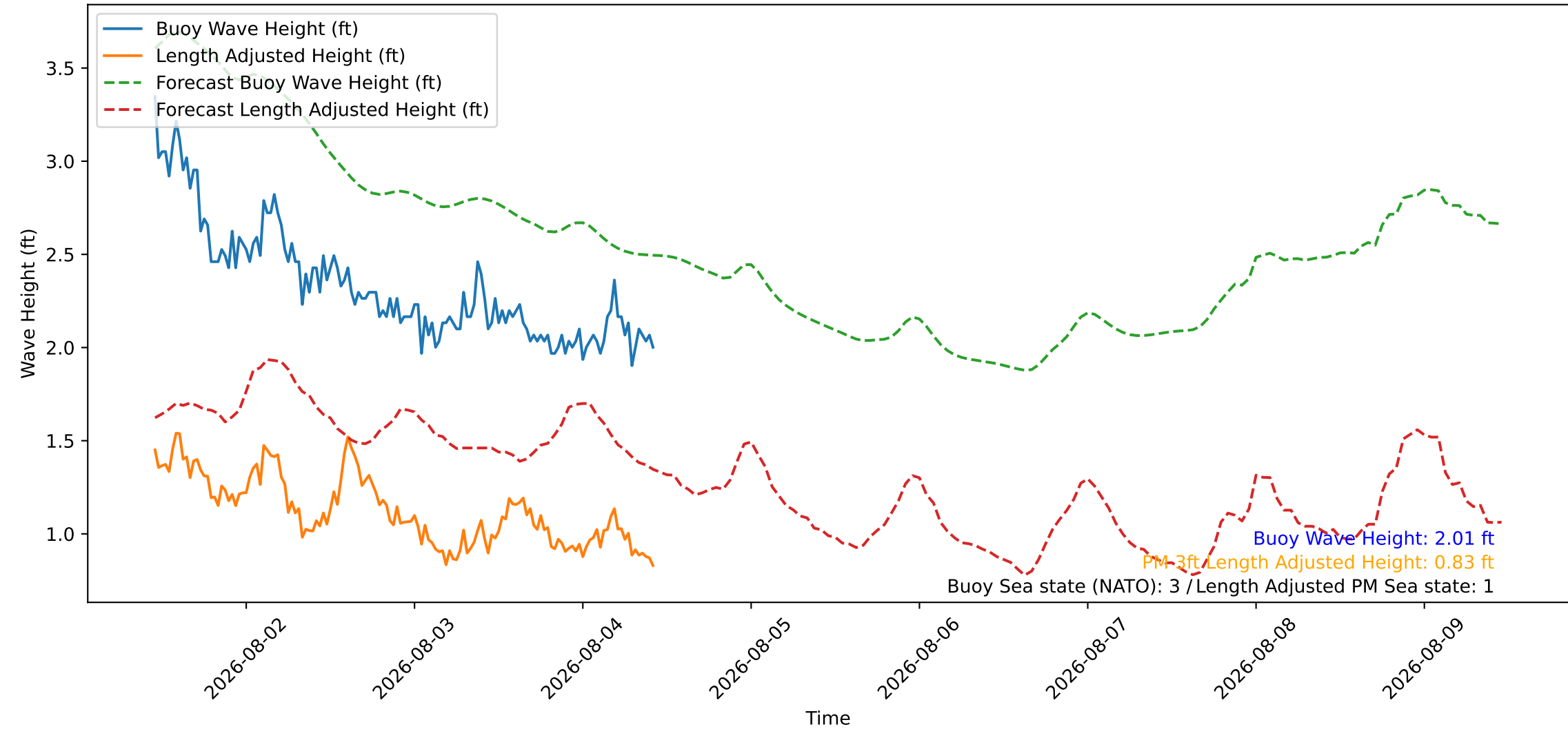
Wave Heights over Time for Red Beach at 2026-08-04 10:50:47
