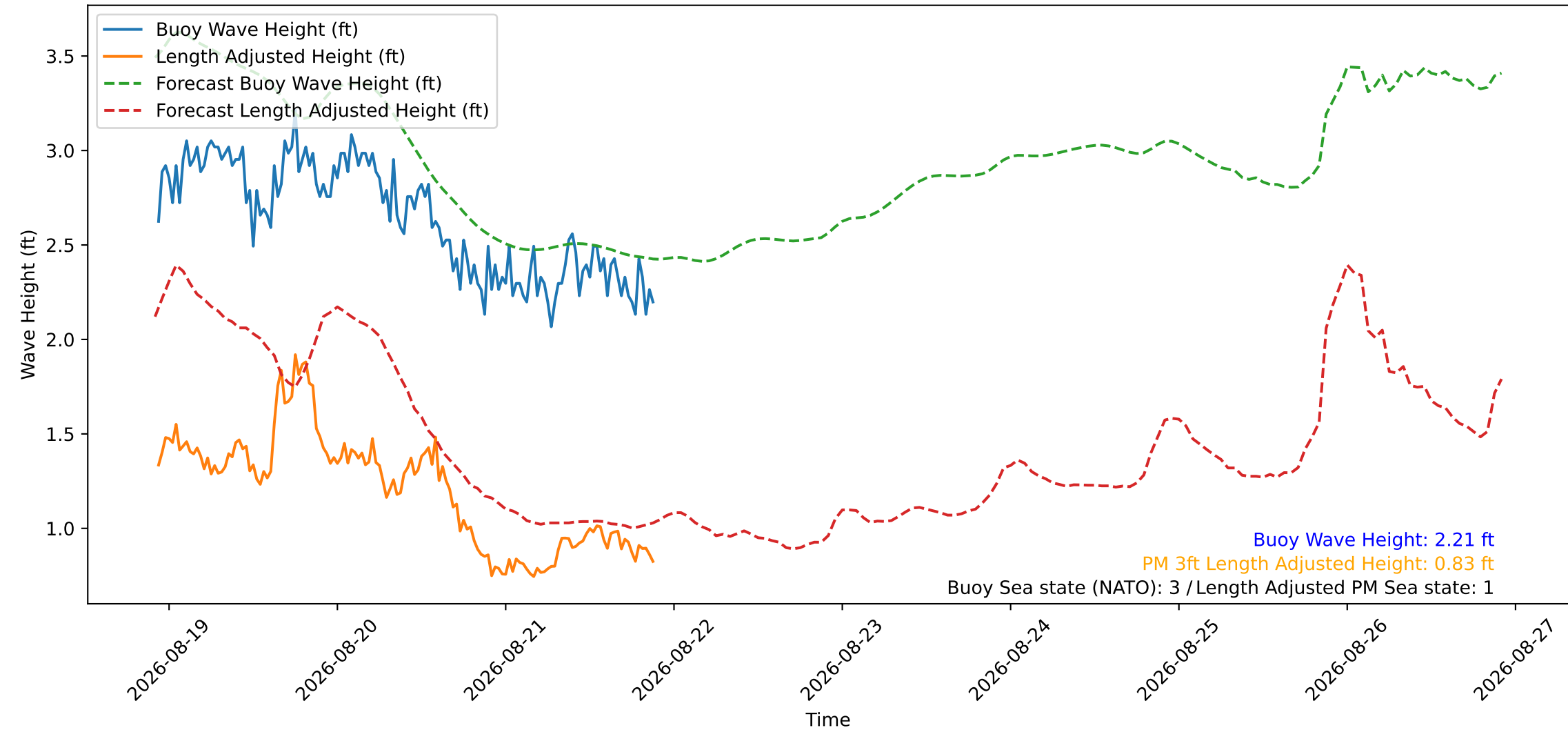
Wave Heights over Time for Red Beach at 2026-08-21 22:00:48
