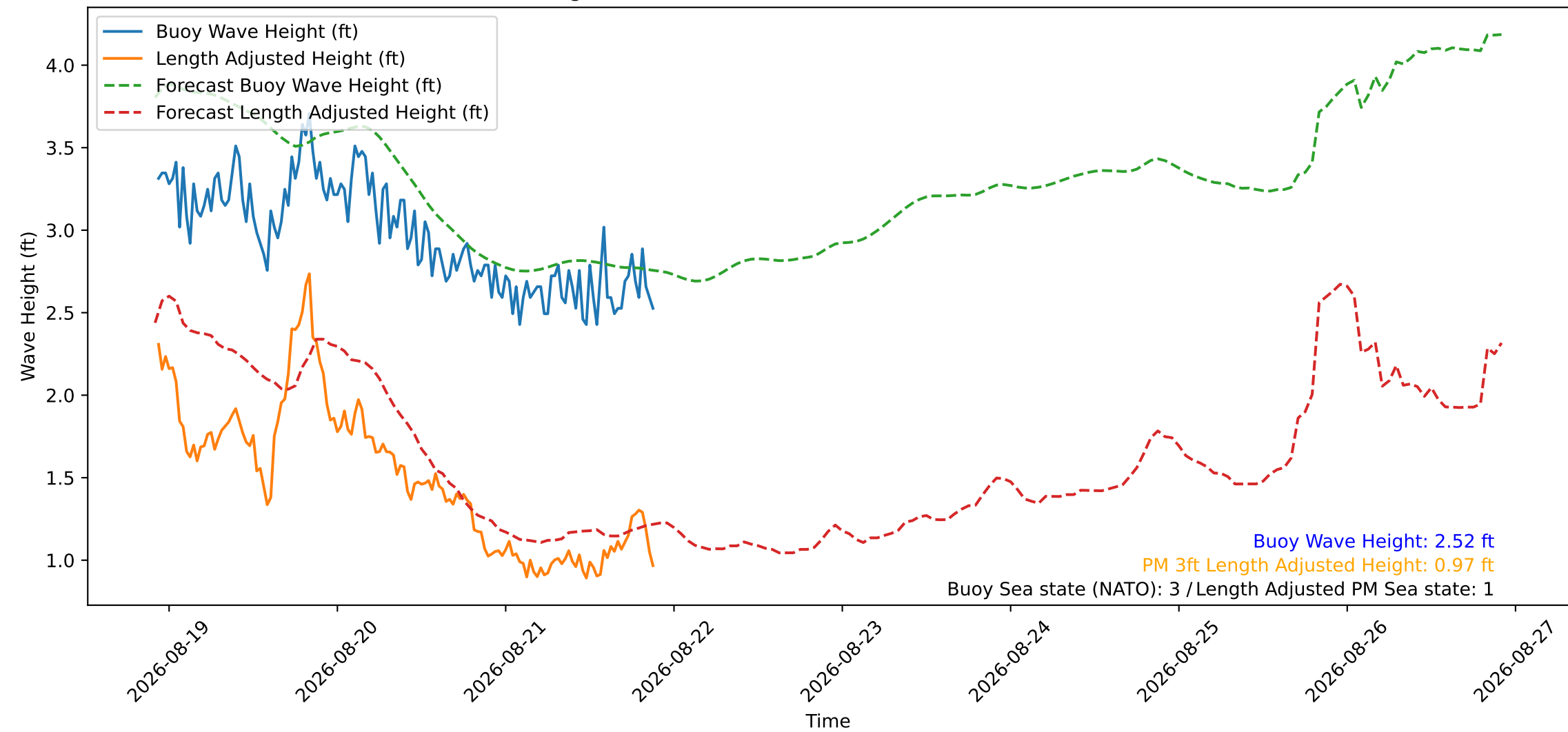
Wave Heights over Time for Green Beach at 2026-08-21 22:01:11
