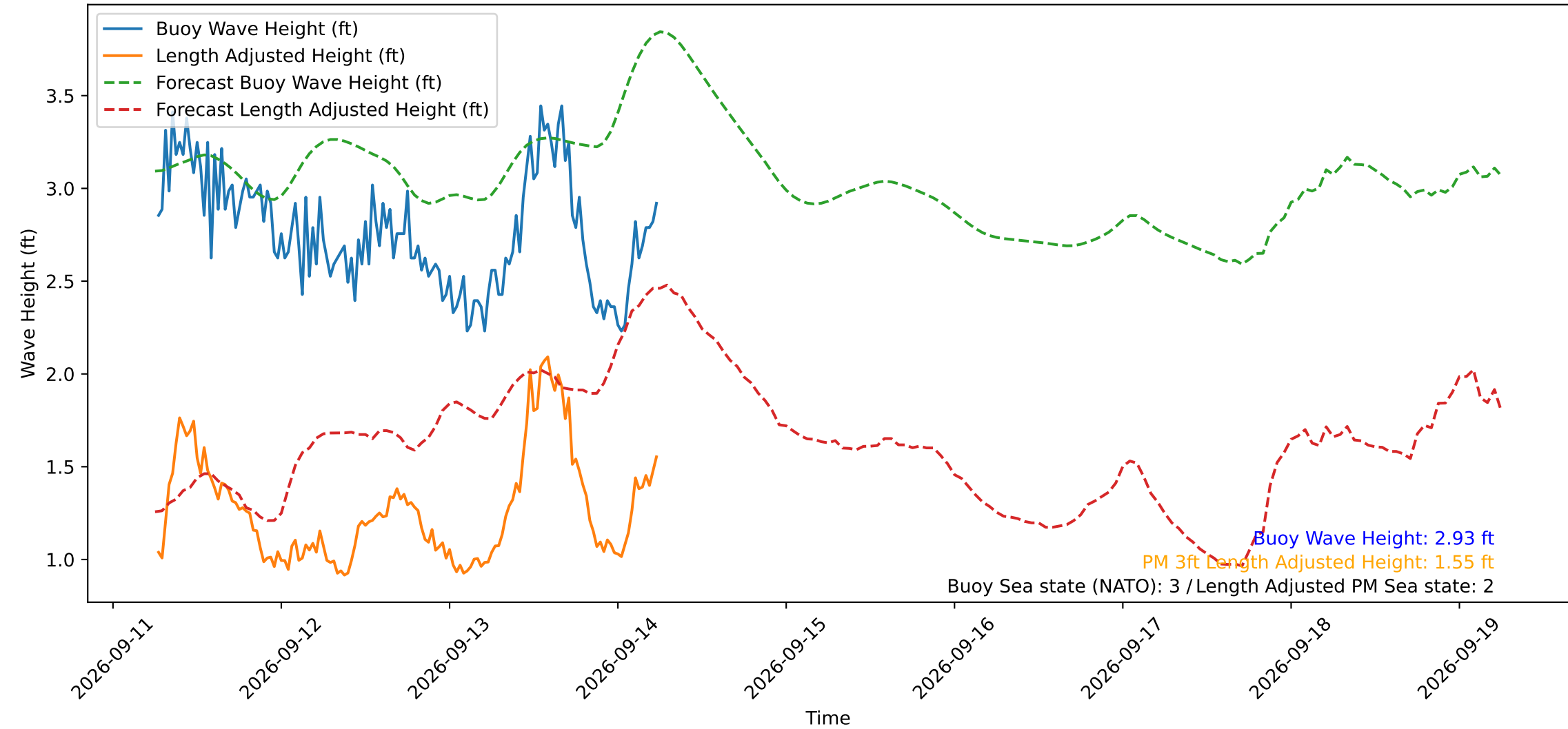
Wave Heights over Time for Red Beach at 2026-09-14 06:20:50
