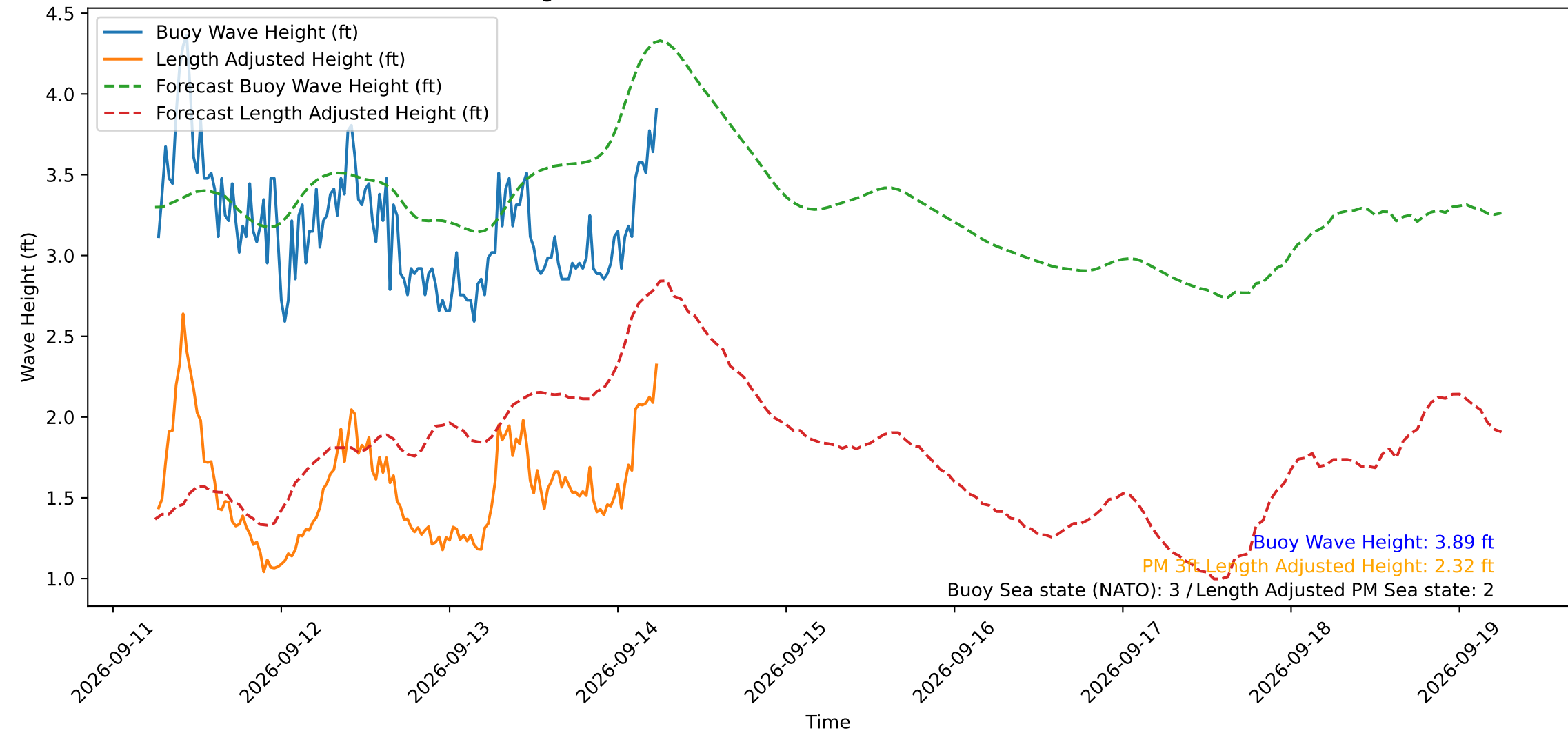
Wave Heights over Time for Oceanside Harbor at 2026-09-14 06:20:29
