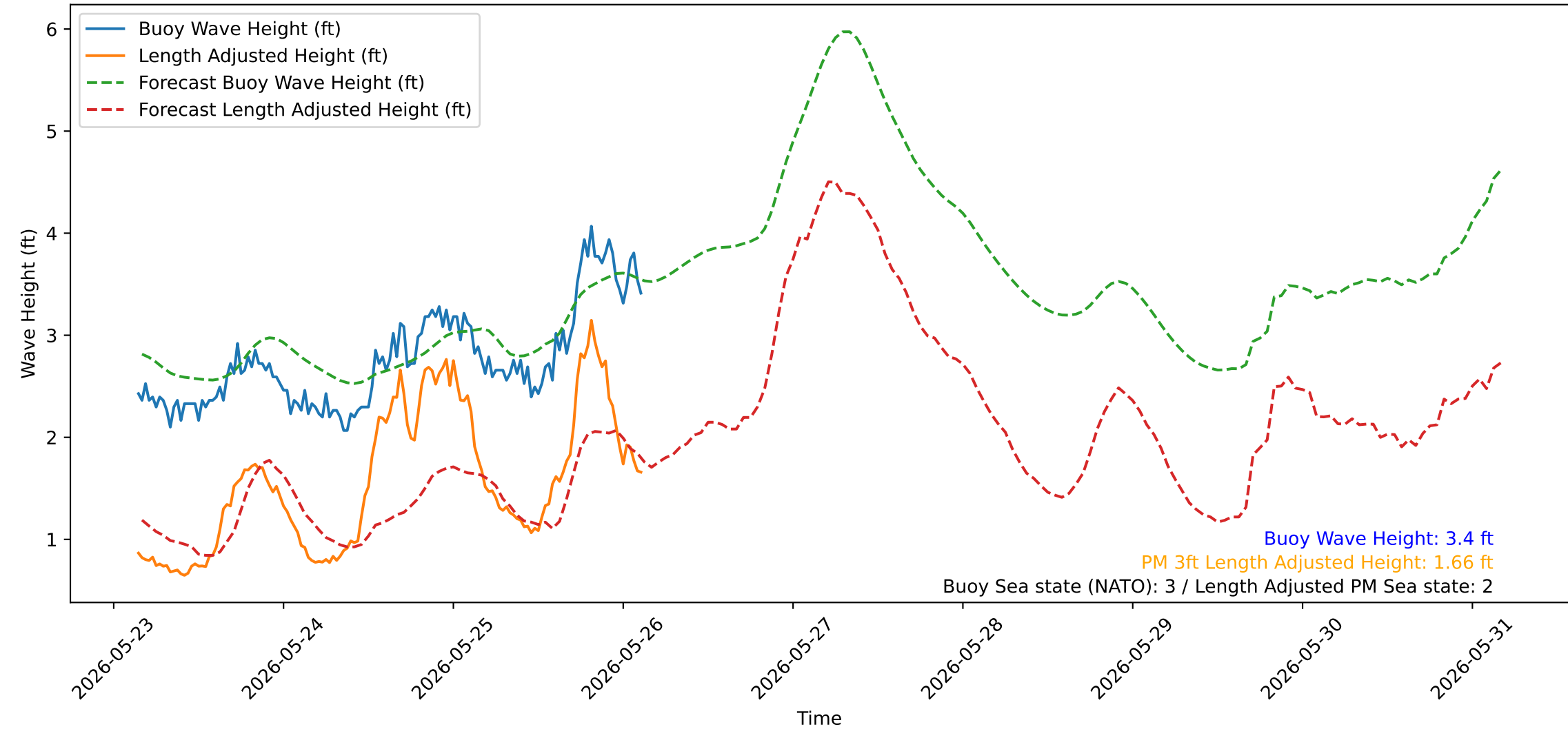
Wave Heights over Time for Green Beach at 2026-05-26 03:31:11
