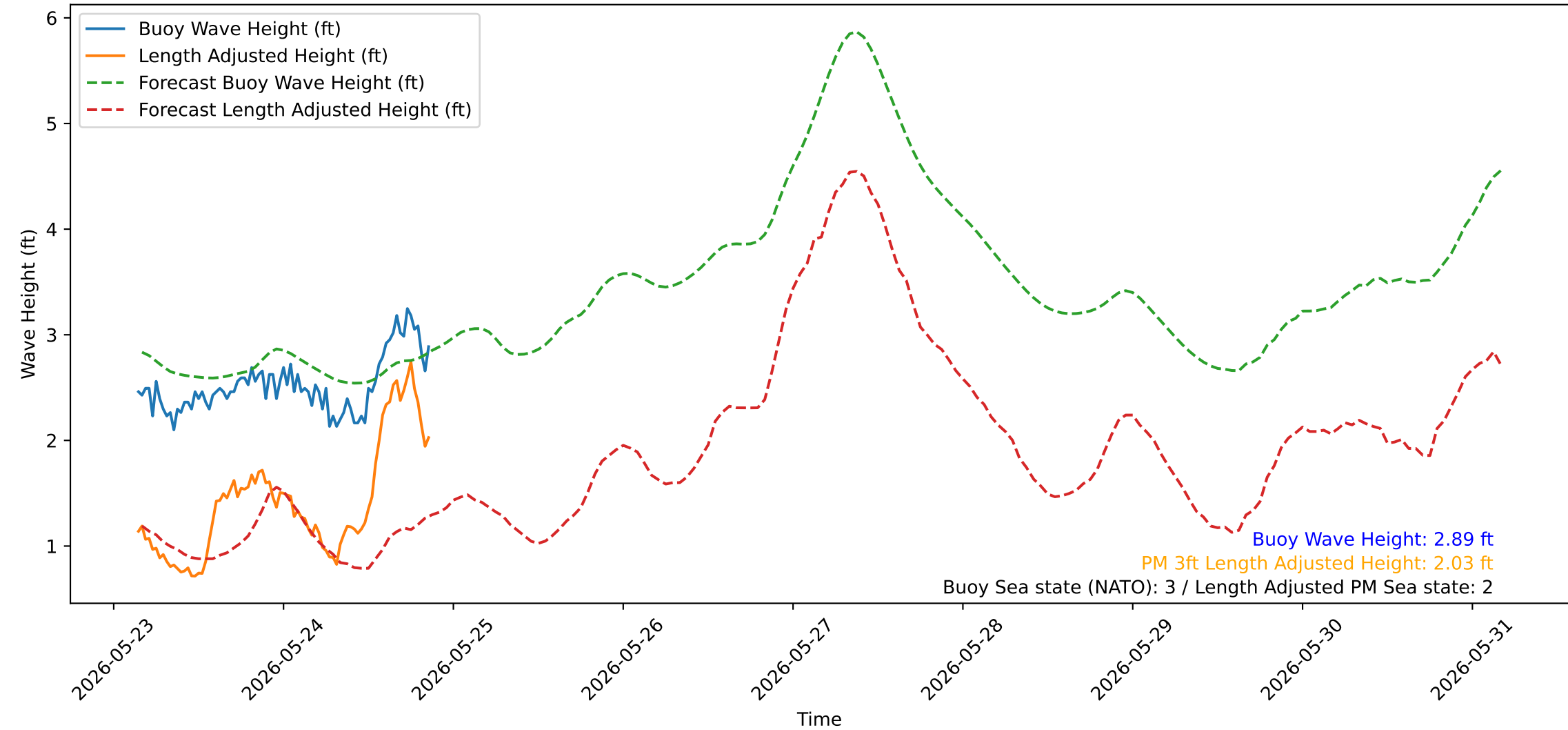
Wave Heights over Time for Oceanside Harbor at 2026-05-26 03:30:29
