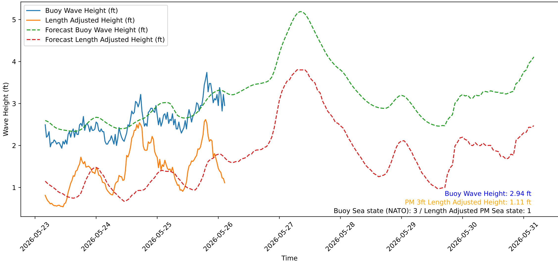
Wave Heights over Time for Red Beach at 2026-05-26 03:30:48
