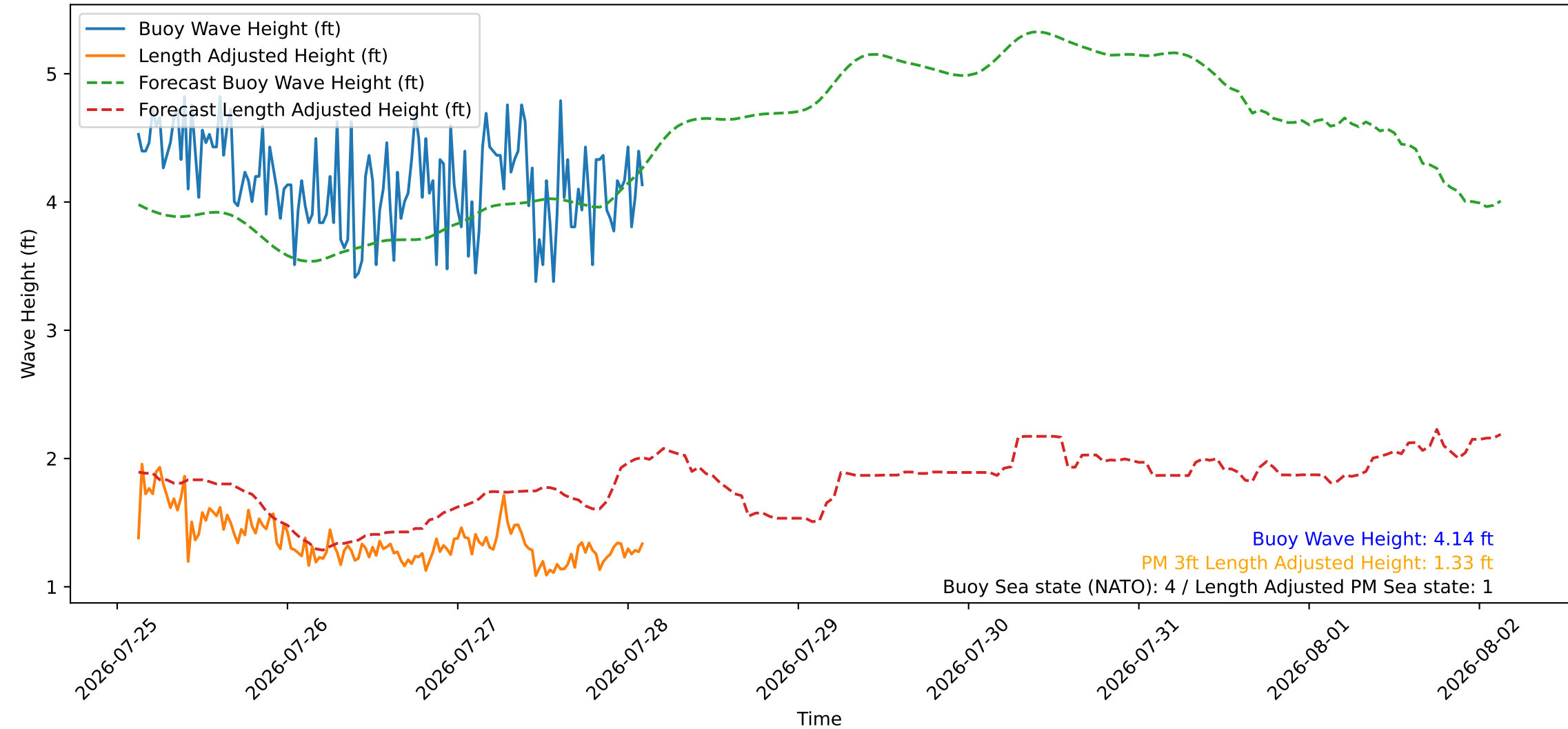
Wave Heights over Time for Green Beach at 2026-07-28 03:01:09
