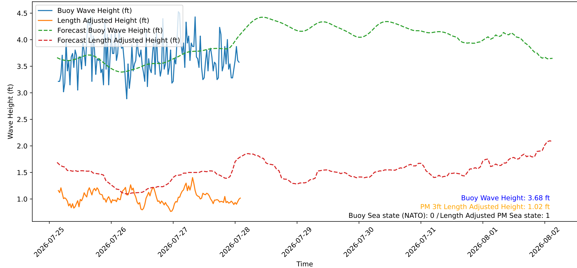
Wave Heights over Time for Red Beach at 2026-07-28 03:00:46
