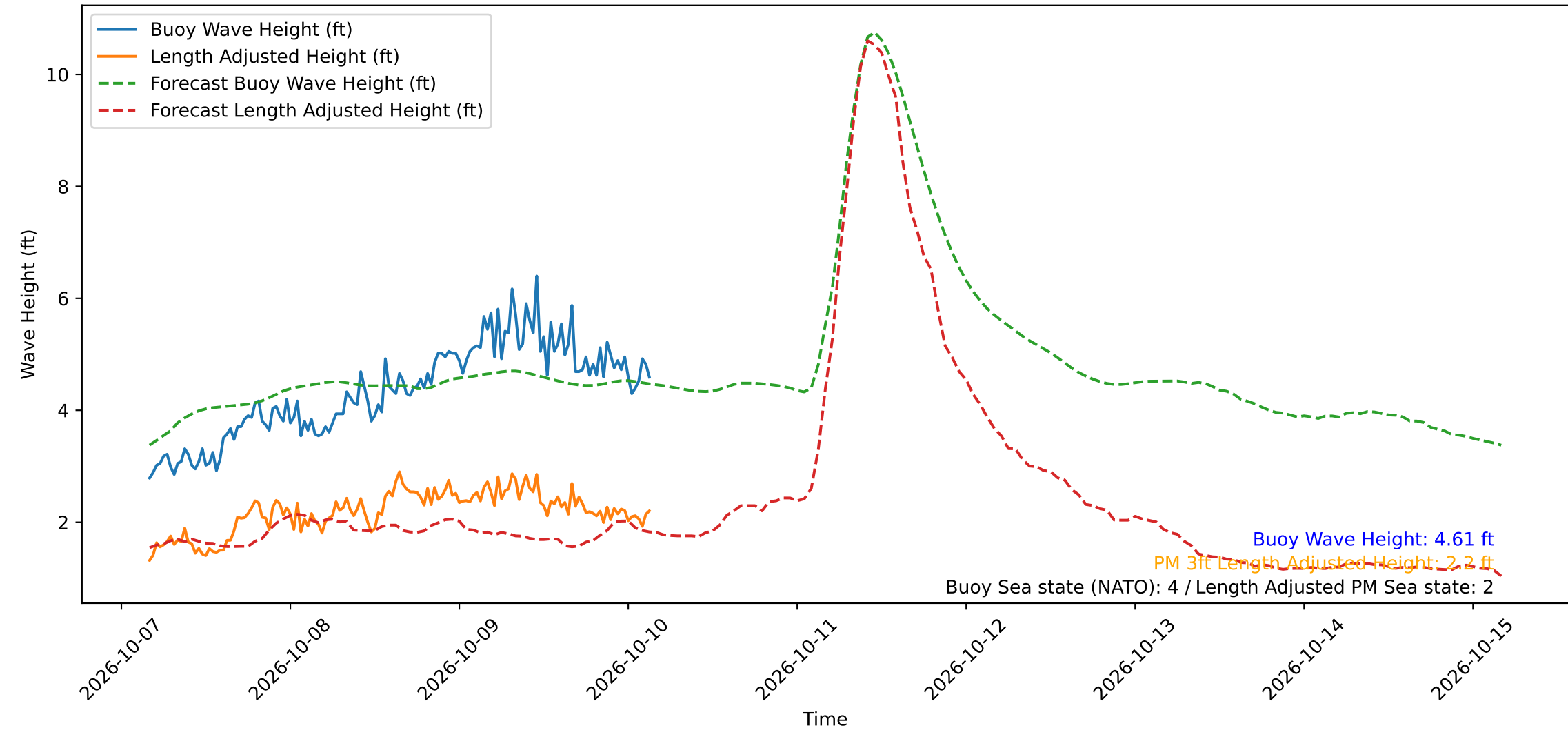
Wave Heights over Time for Oceanside Harbor at 2026-10-10 04:00:29
