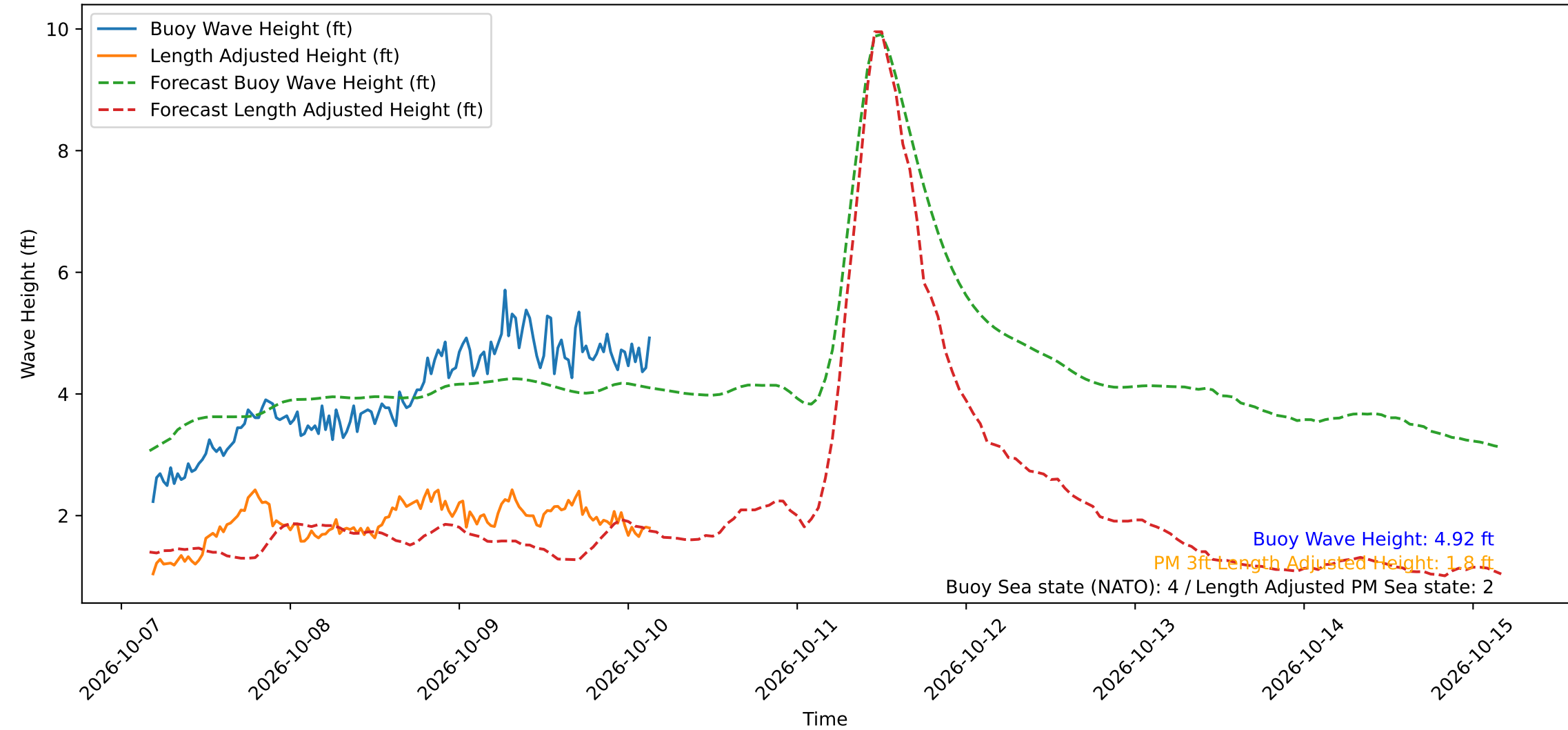
Wave Heights over Time for Red Beach at 2026-10-10 04:00:49
