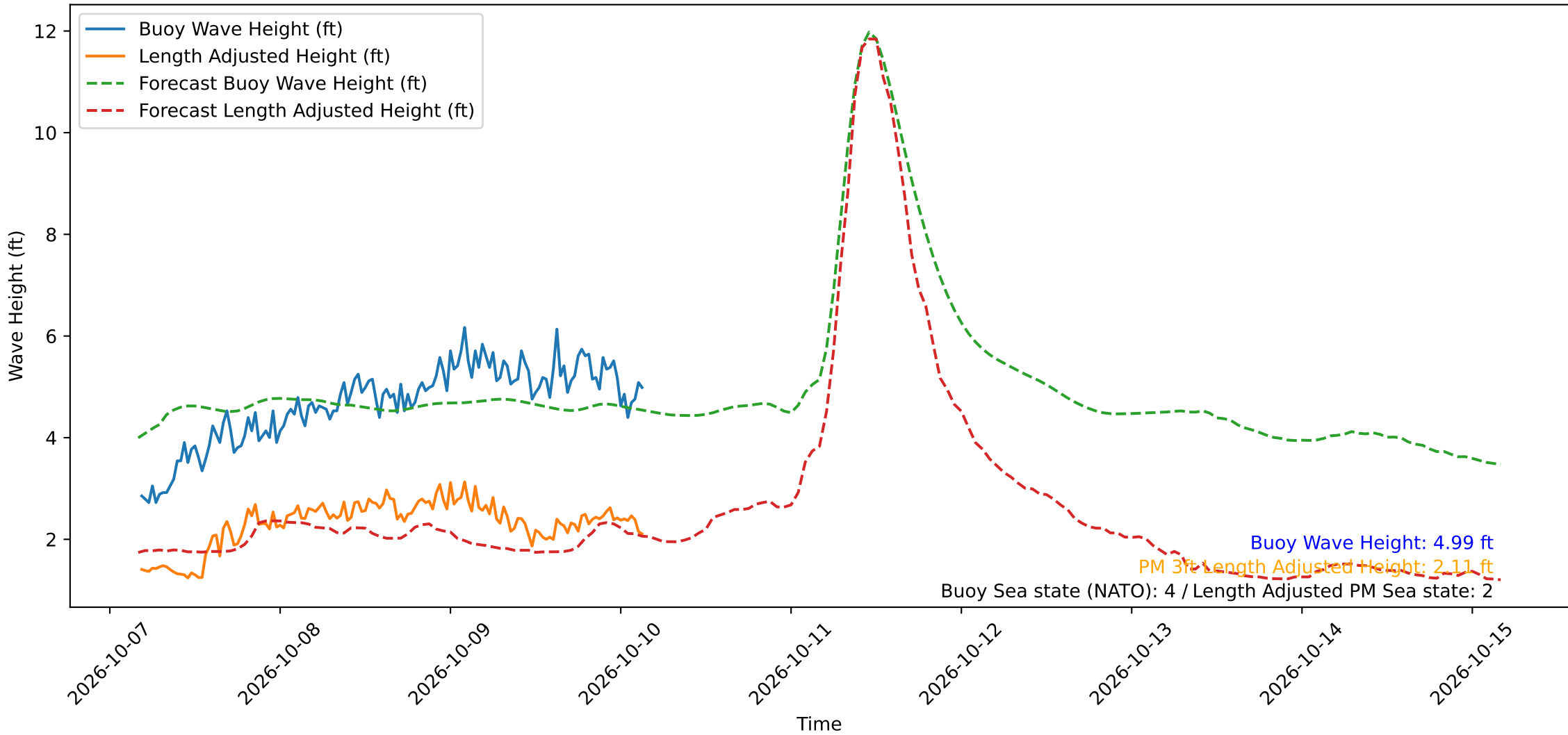
Wave Heights over Time for Green Beach at 2026-10-10 04:01:11
