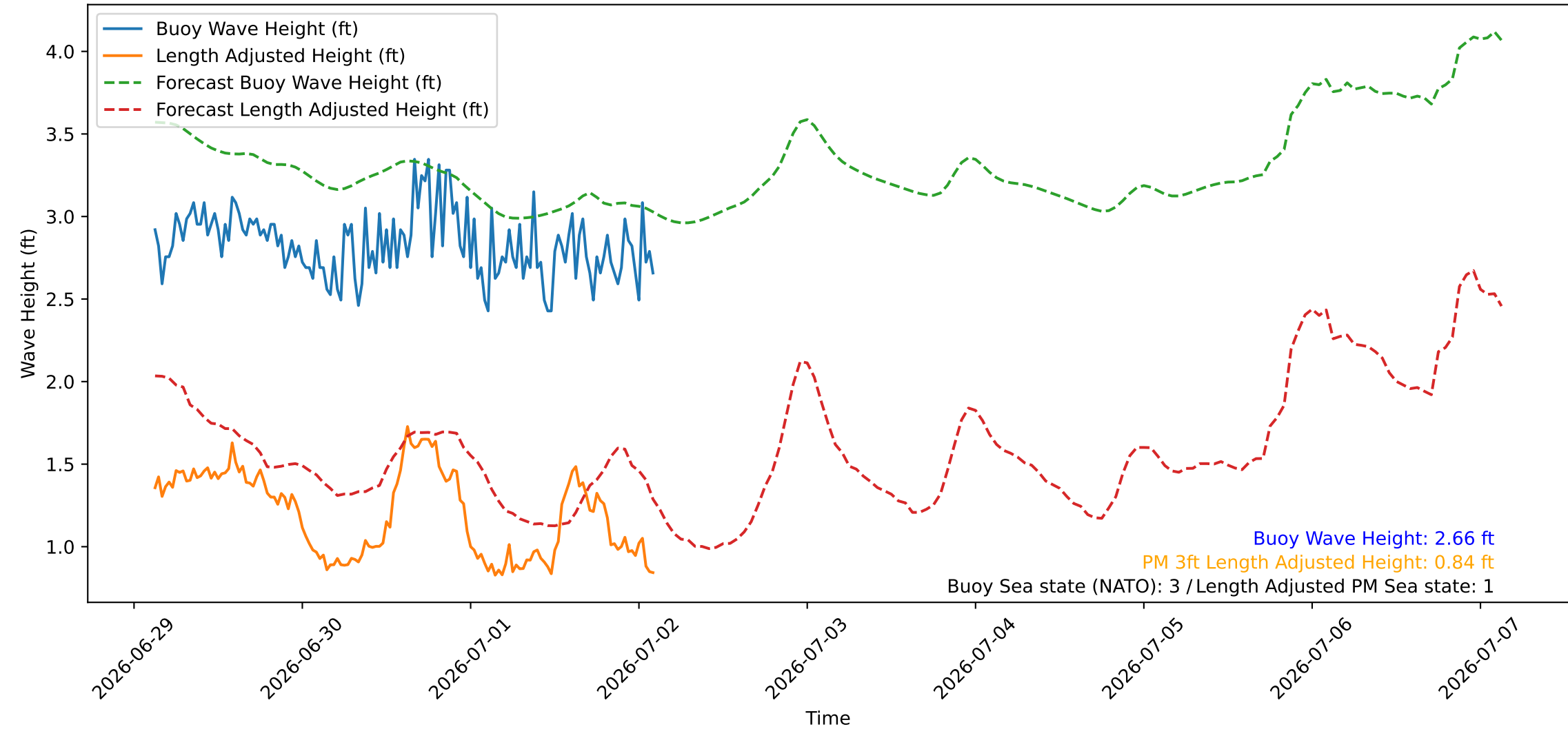
Wave Heights over Time for Red Beach at 2026-07-02 02:50:47
