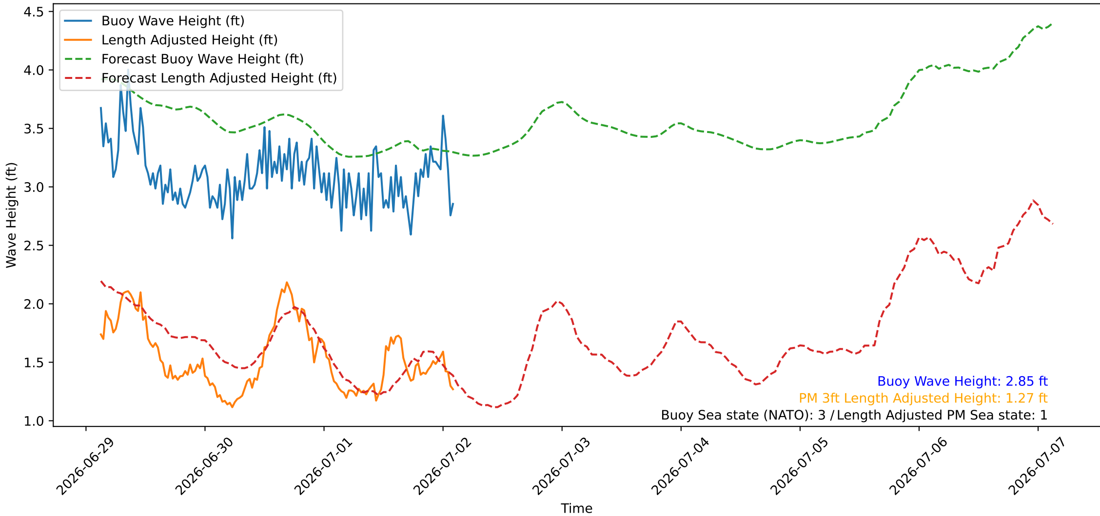
Wave Heights over Time for Oceanside Harbor at 2026-07-02 02:50:26
