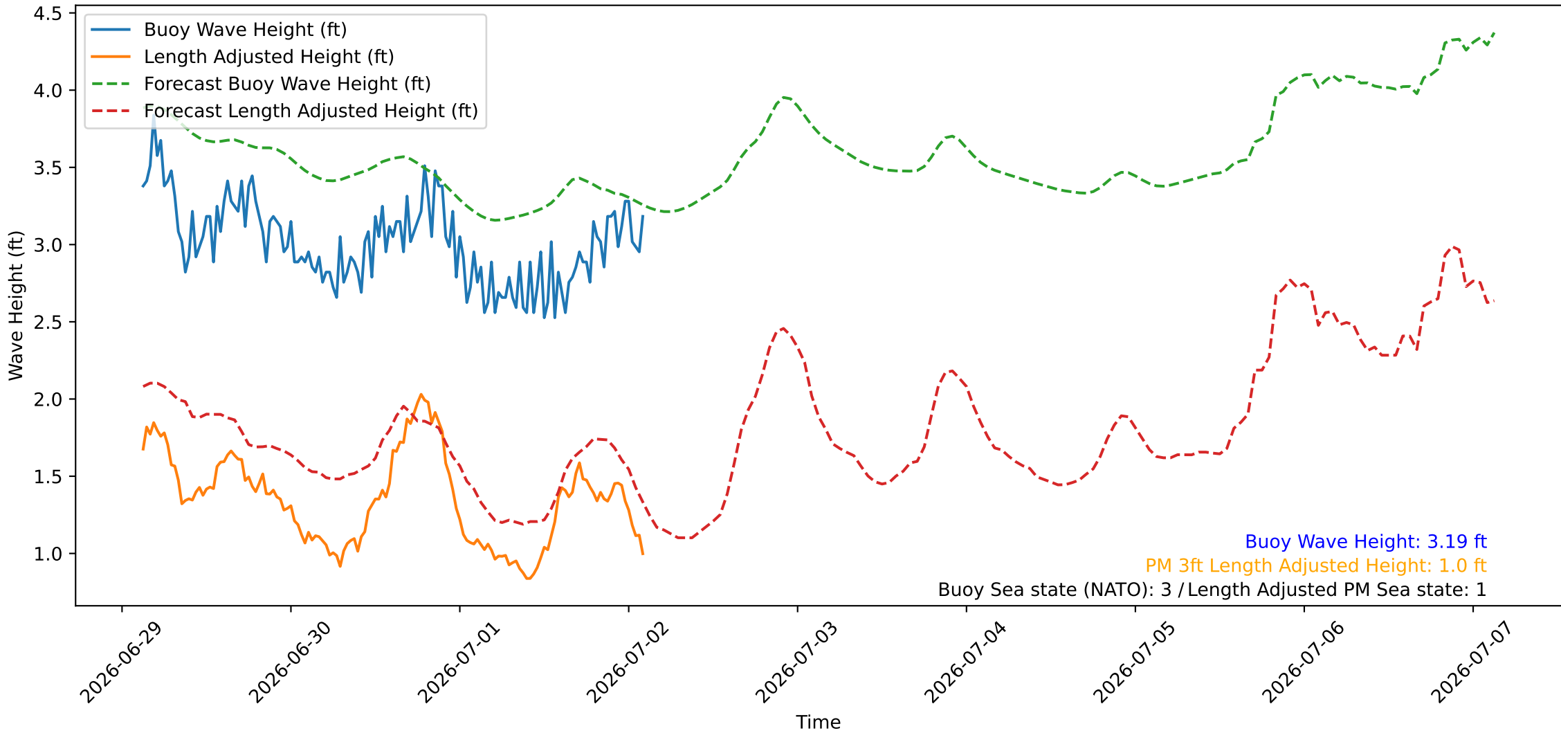
Wave Heights over Time for Green Beach at 2026-07-02 02:51:09
