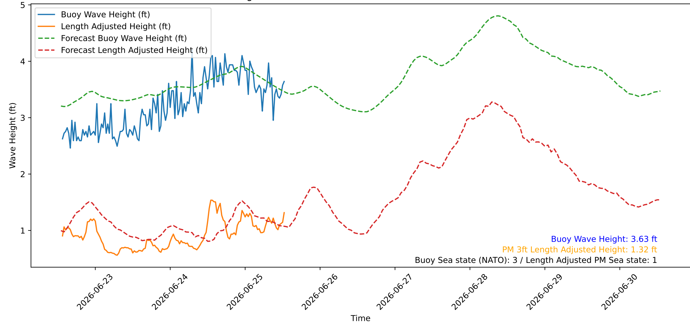
Wave Heights over Time for Green Beach at 2026-06-25 13:21:09
