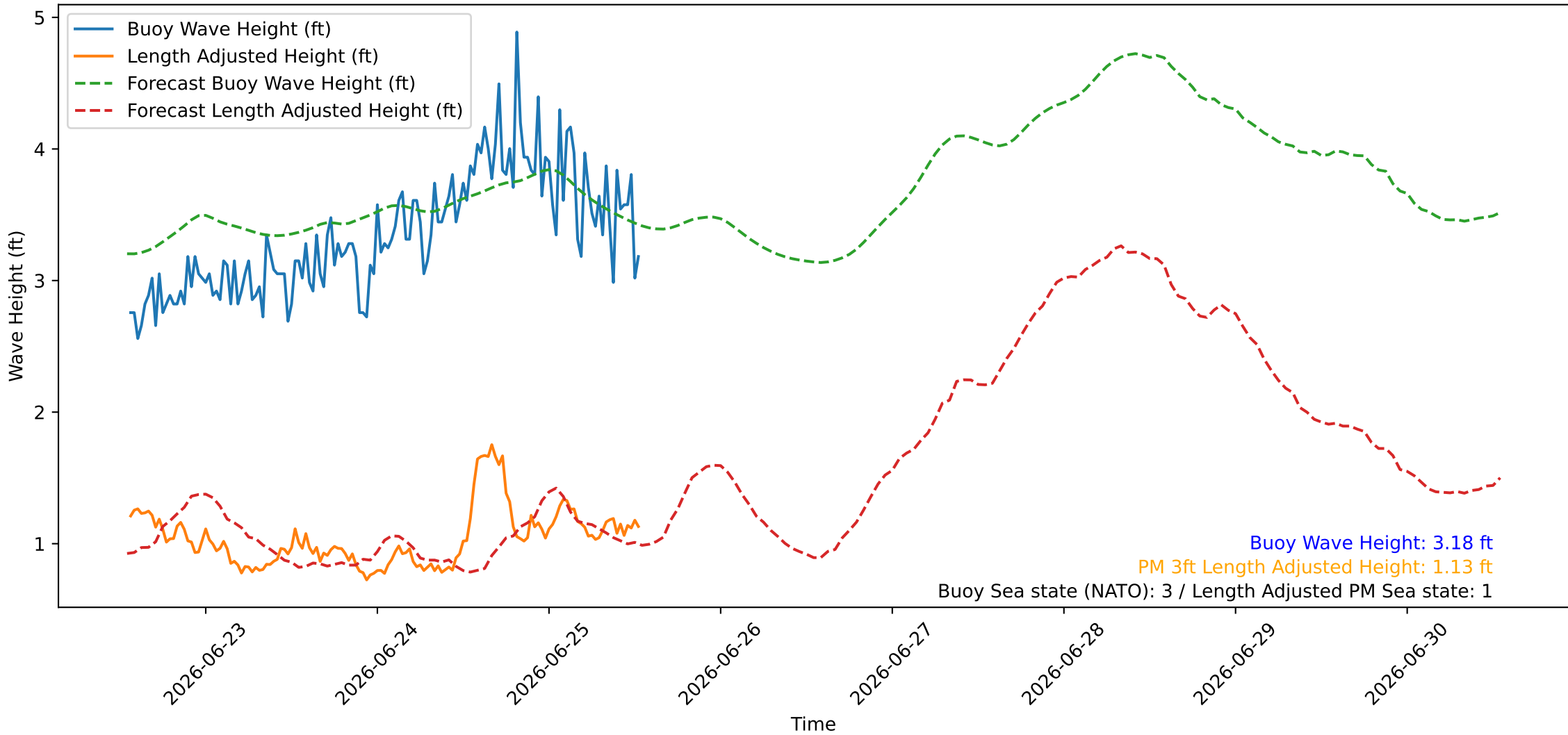
Wave Heights over Time for Oceanside Harbor at 2026-06-25 13:20:26
