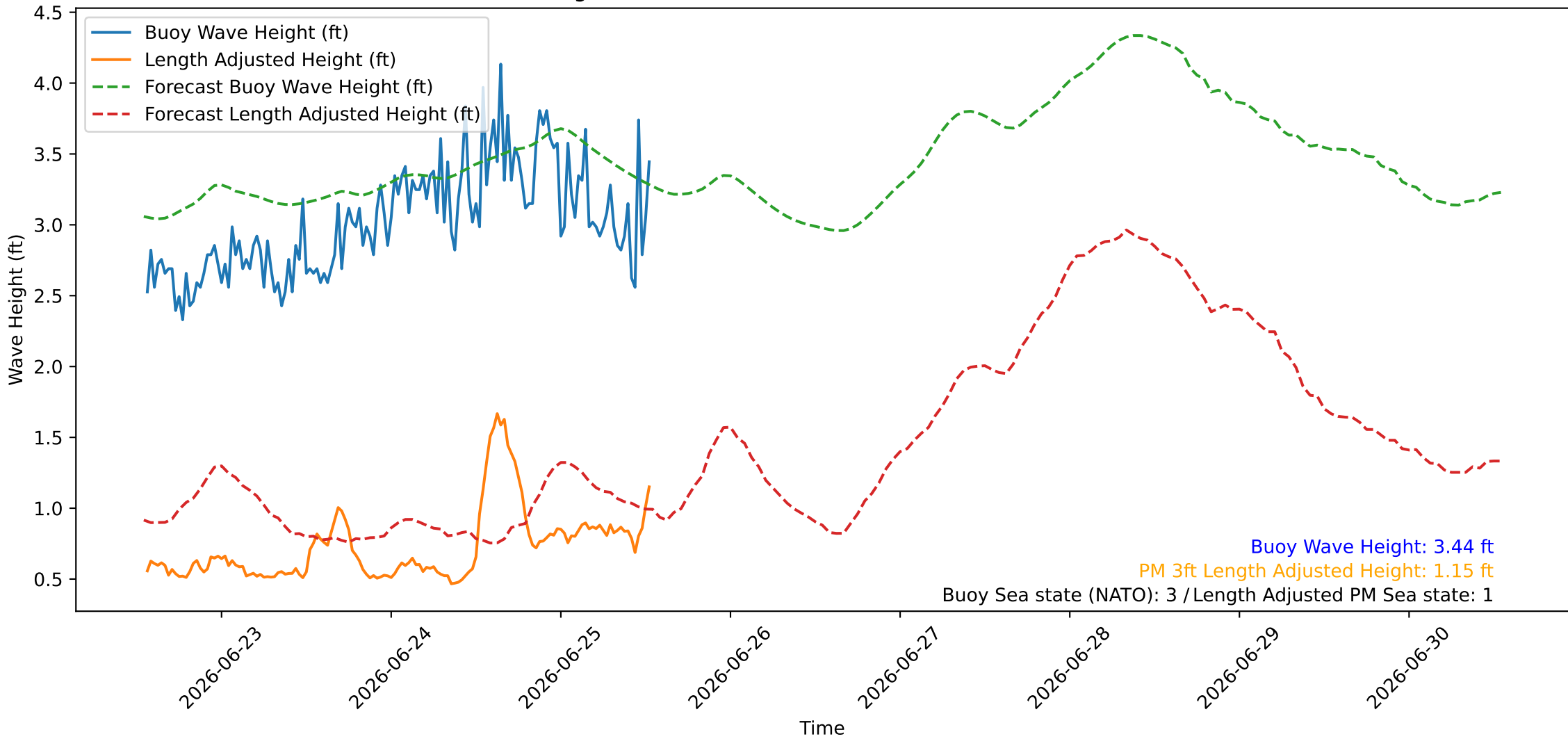
Wave Heights over Time for Red Beach at 2026-06-25 13:20:47
