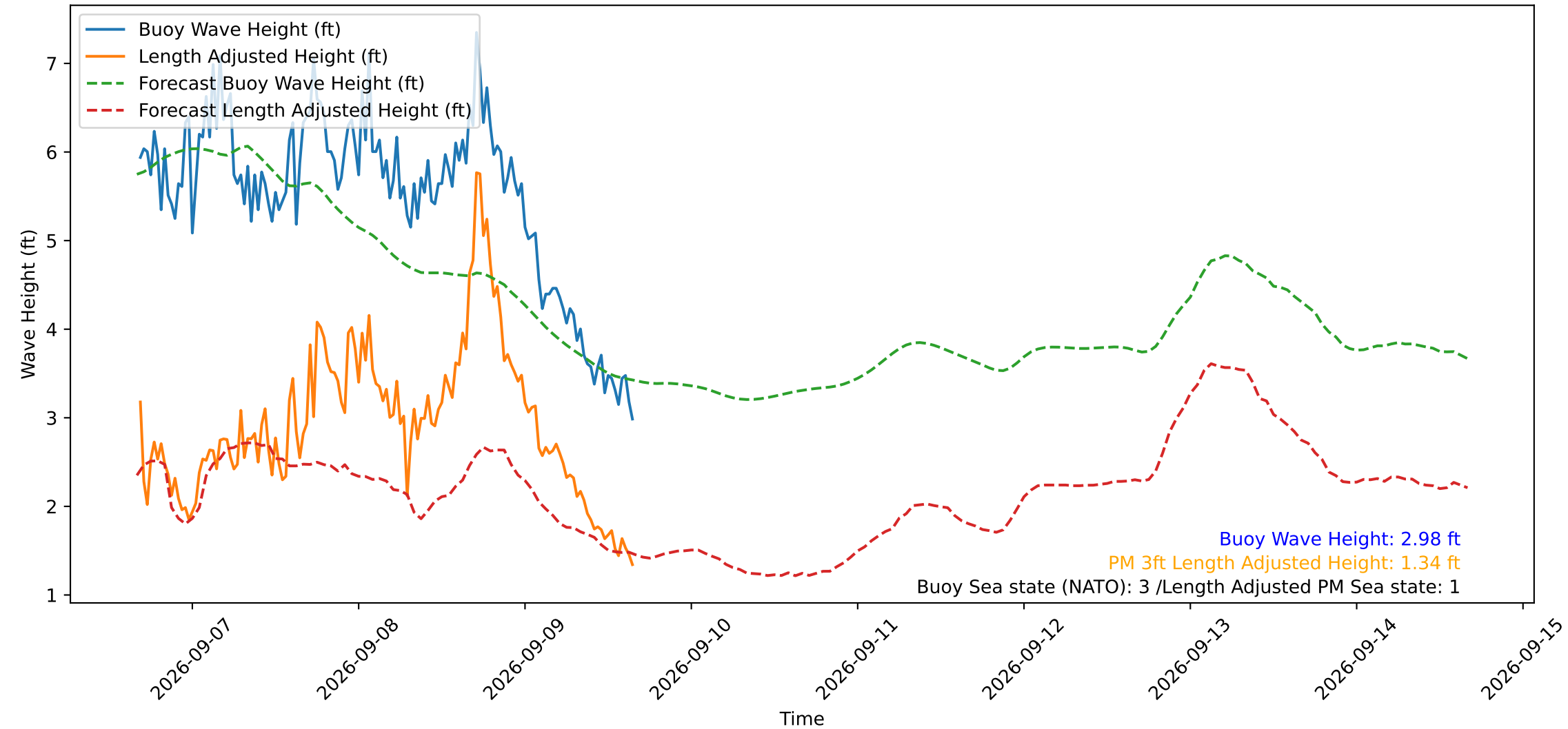
Wave Heights over Time for Oceanside Harbor at 2026-09-09 16:20:29
