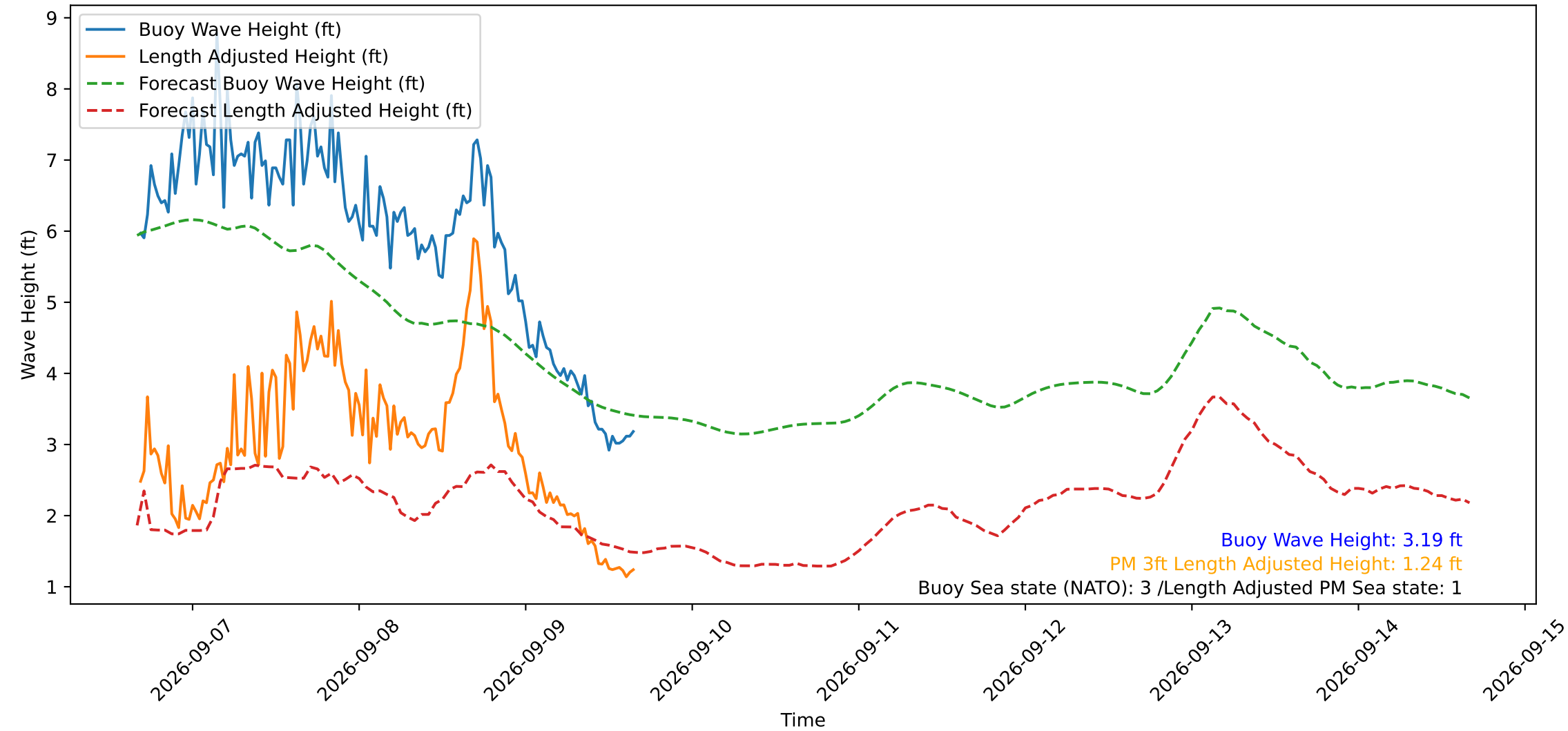
Wave Heights over Time for Green Beach at 2026-09-09 16:21:14
