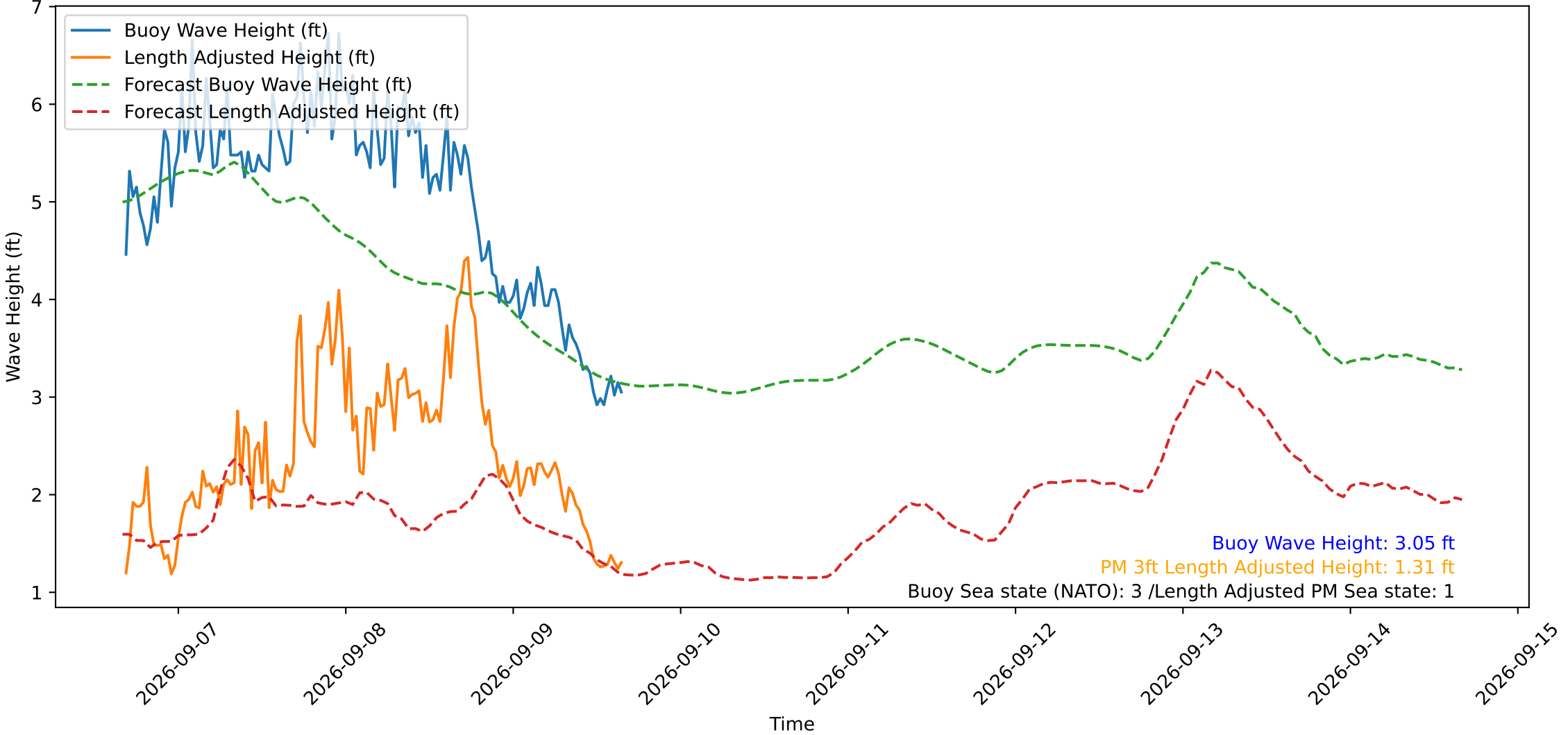
Wave Heights over Time for Red Beach at 2026-09-09 16:20:50
