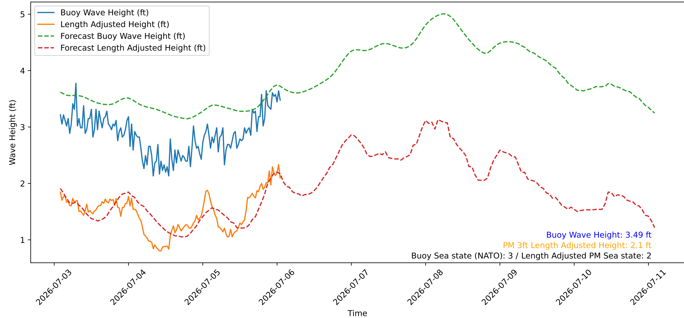
Wave Heights over Time for Oceanside Harbor at 2026-07-06 01:50:26
