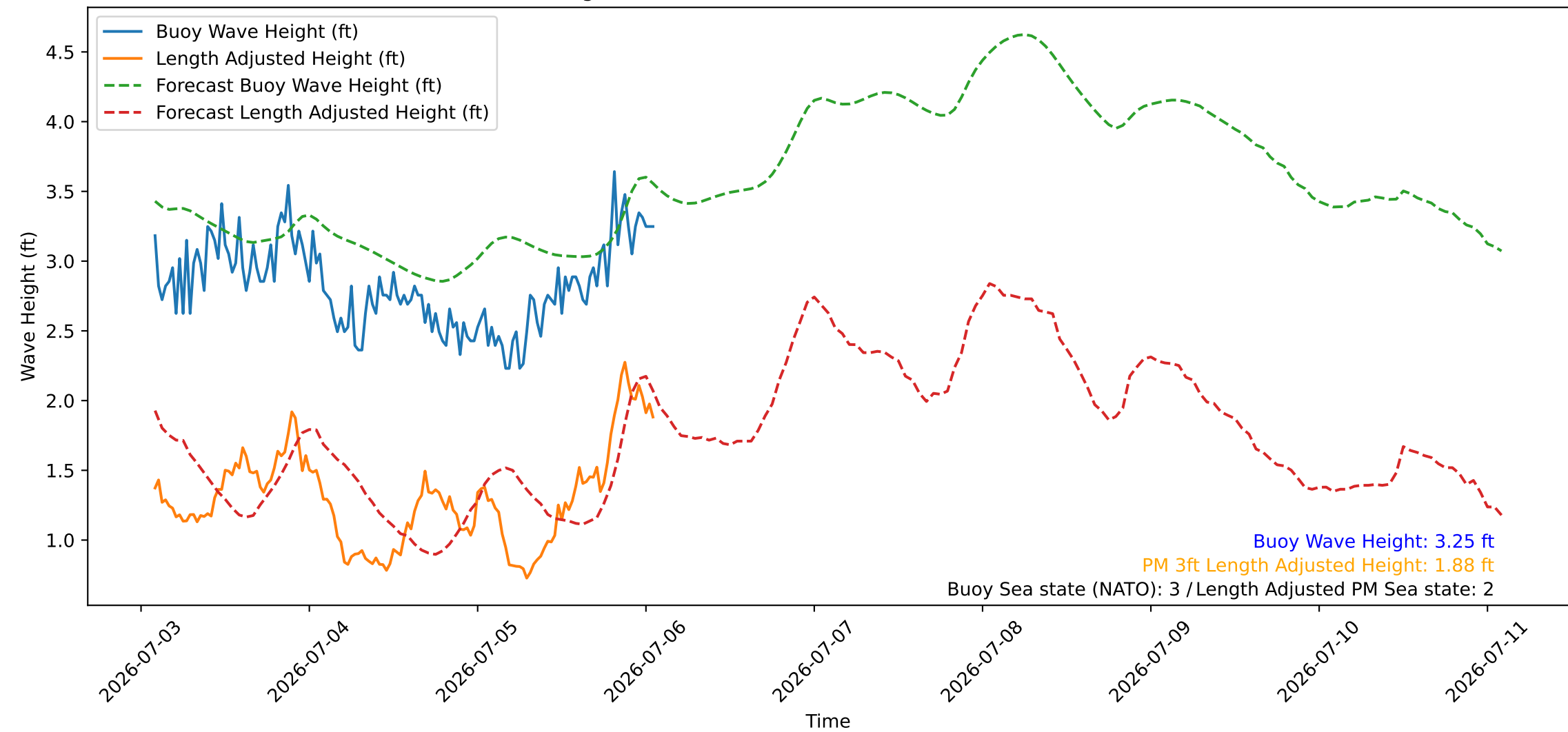
Wave Heights over Time for Red Beach at 2026-07-06 01:50:47
