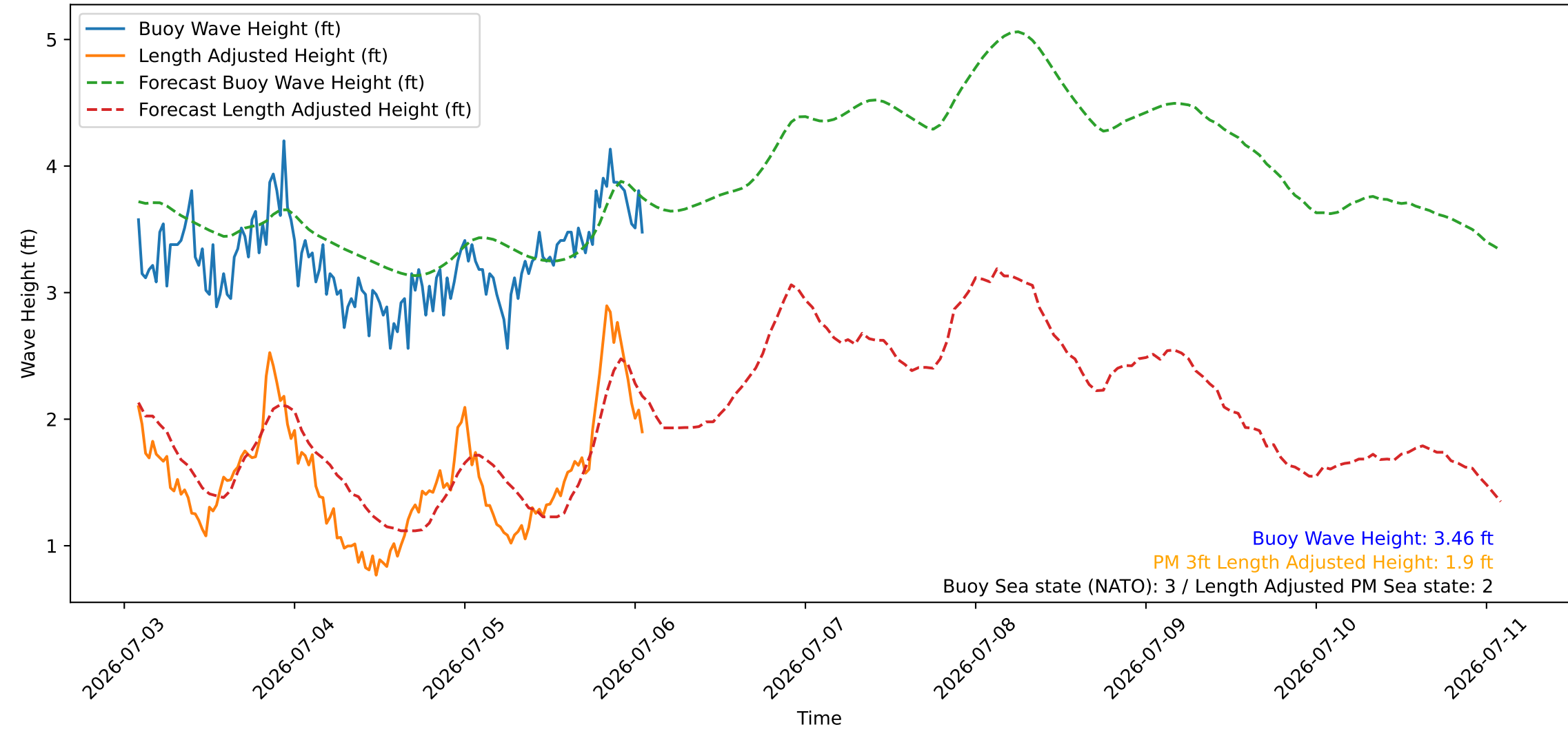
Wave Heights over Time for Green Beach at 2026-07-06 01:51:10
