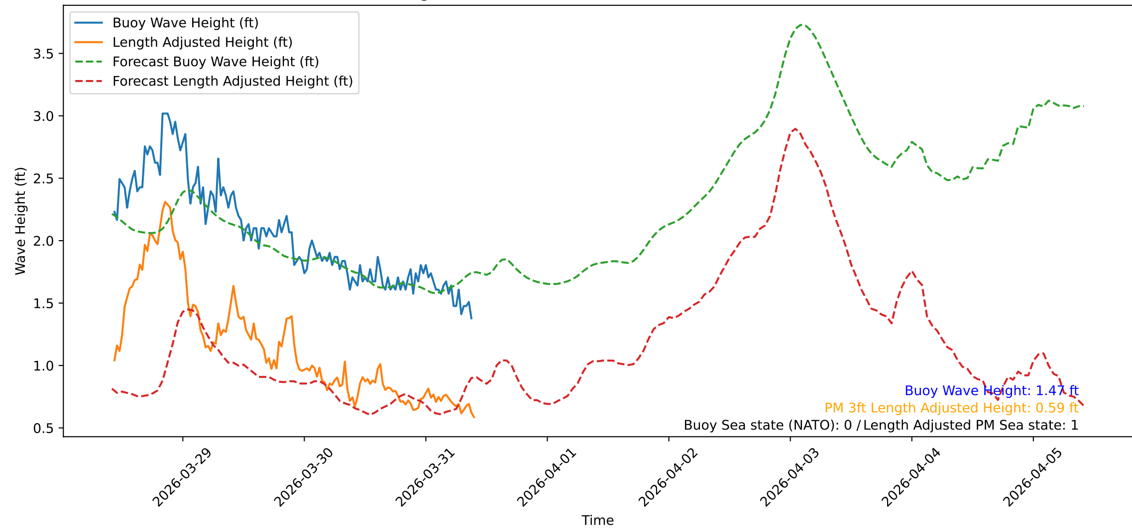
Wave Heights over Time for Red Beach at 2026-03-31 10:10:48
