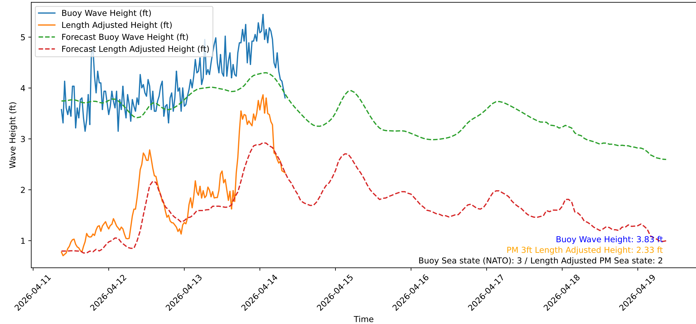
Wave Heights over Time for Oceanside Harbor at 2026-04-14 08:50:31
