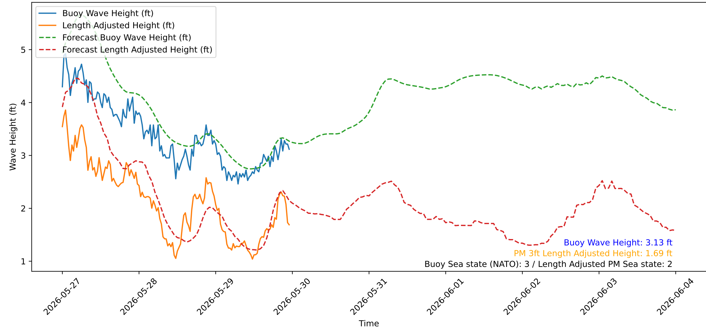
Wave Heights over Time for Green Beach at 2026-05-30 00:01:04
