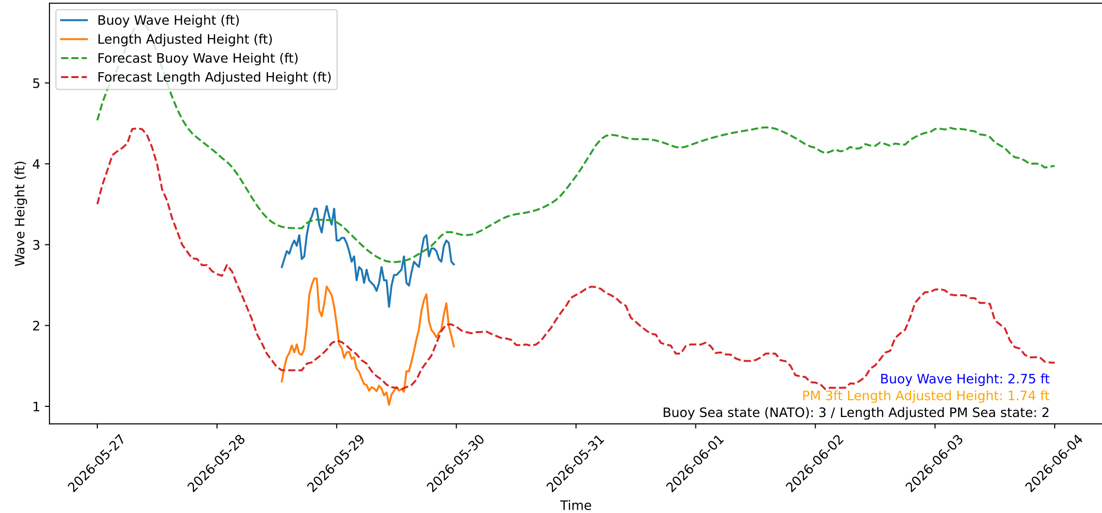
Wave Heights over Time for Oceanside Harbor at 2026-05-30 00:00:22
