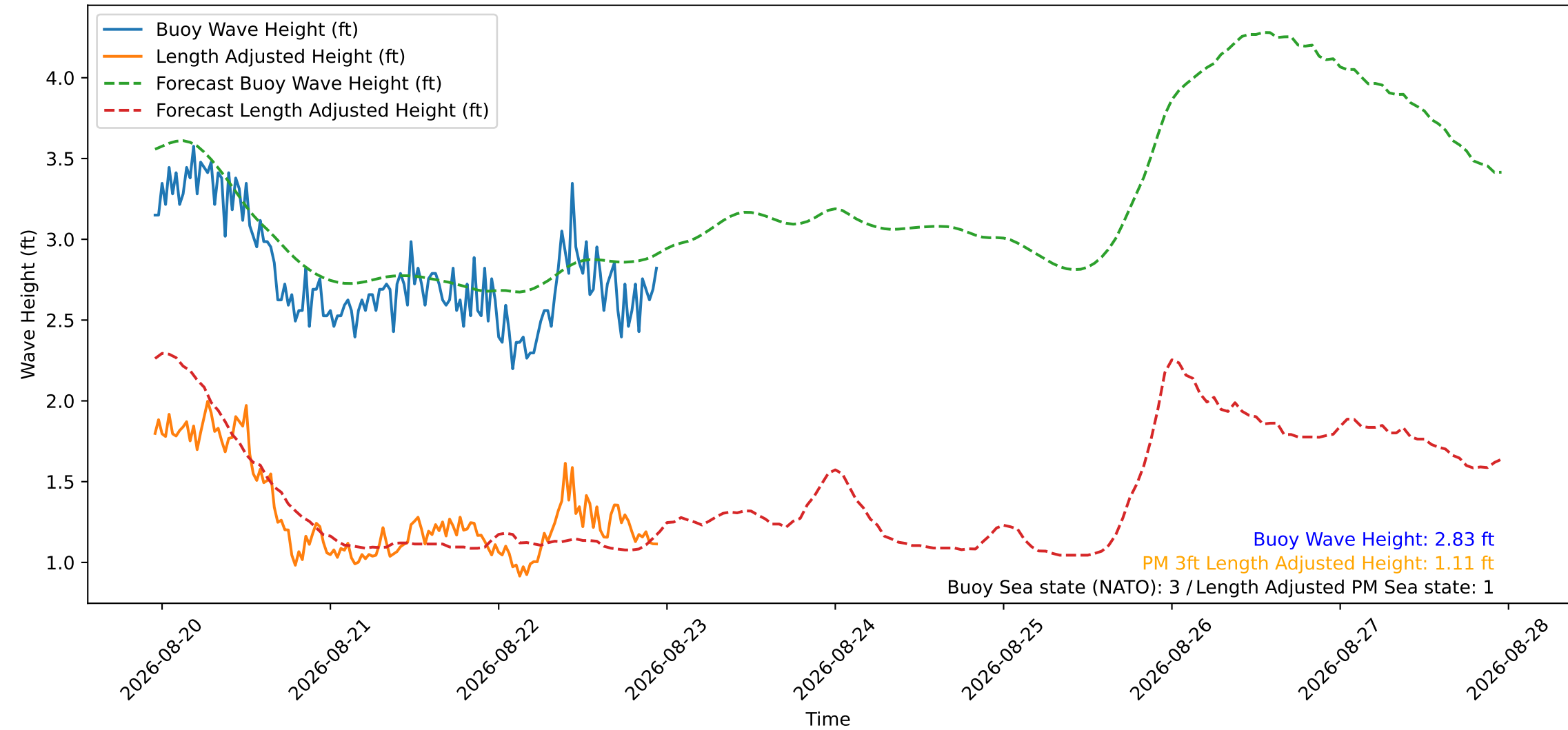
Wave Heights over Time for Oceanside Harbor at 2026-08-22 23:10:30
