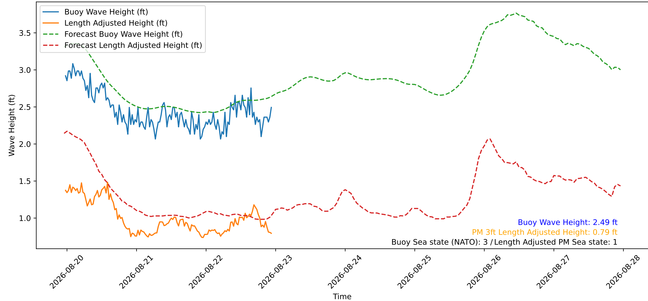
Wave Heights over Time for Red Beach at 2026-08-22 23:10:50
