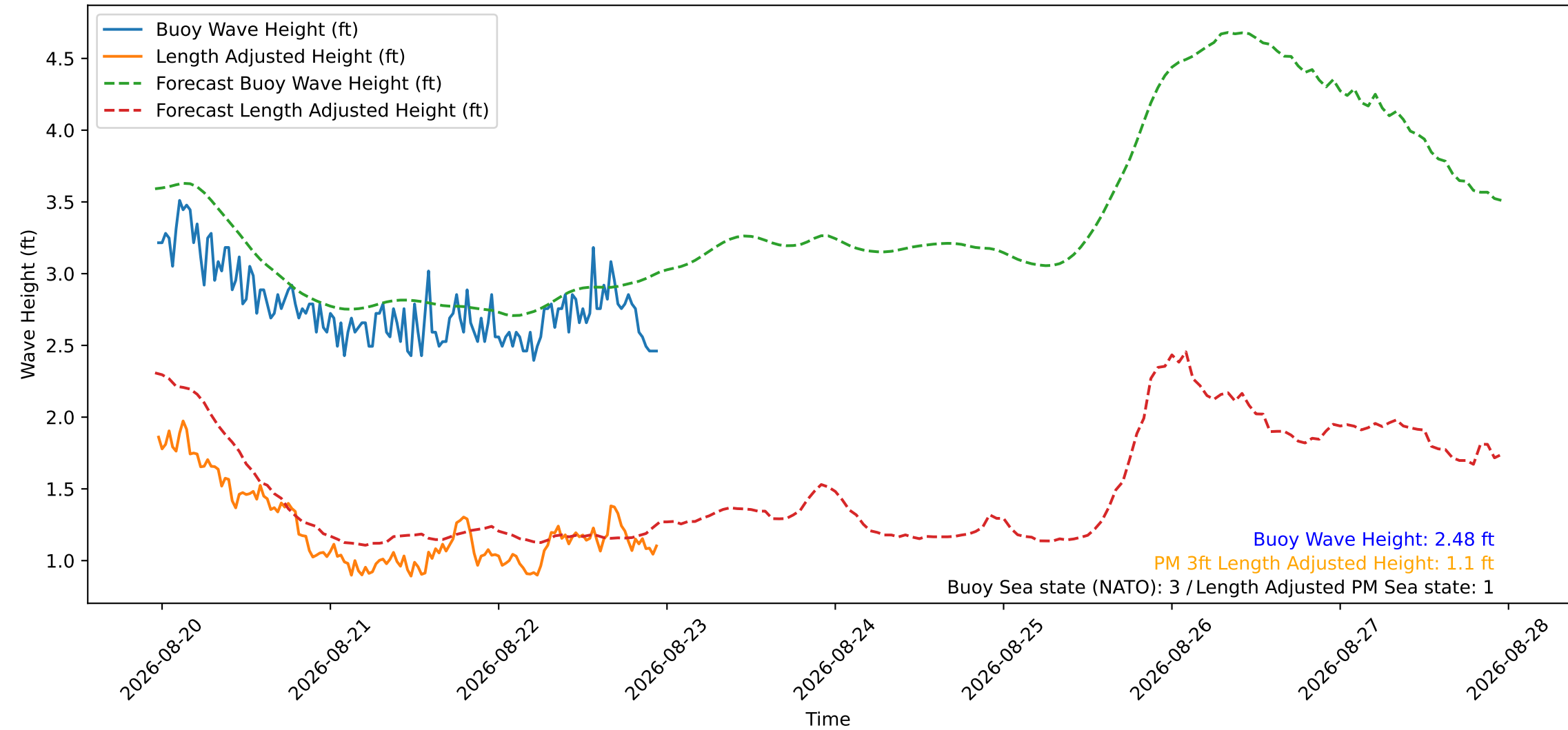
Wave Heights over Time for Green Beach at 2026-08-22 23:11:12
