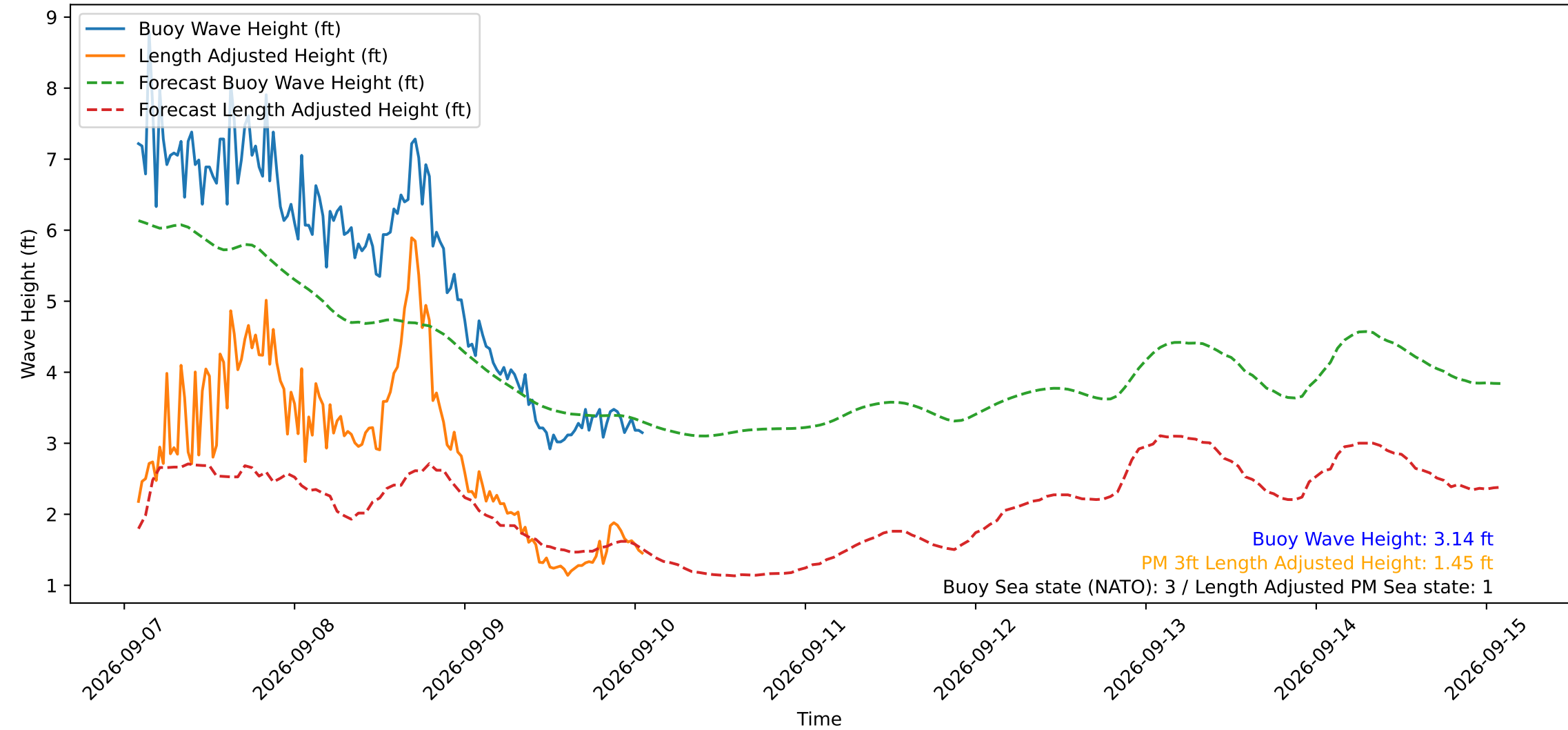
Wave Heights over Time for Green Beach at 2026-09-10 01:51:14
