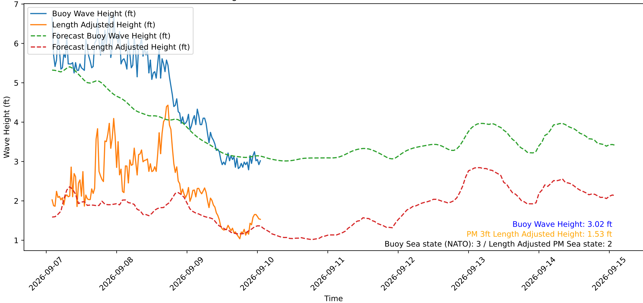
Wave Heights over Time for Red Beach at 2026-09-10 01:50:50
