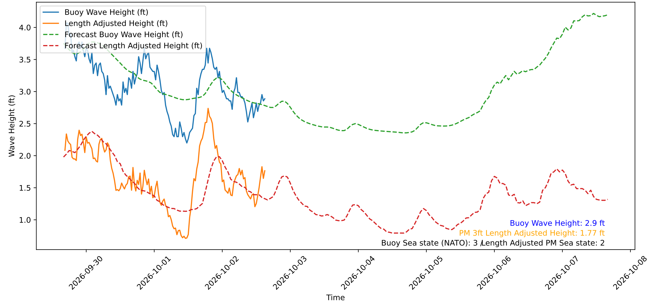
Wave Heights over Time for Green Beach at 2026-10-02 16:01:11
