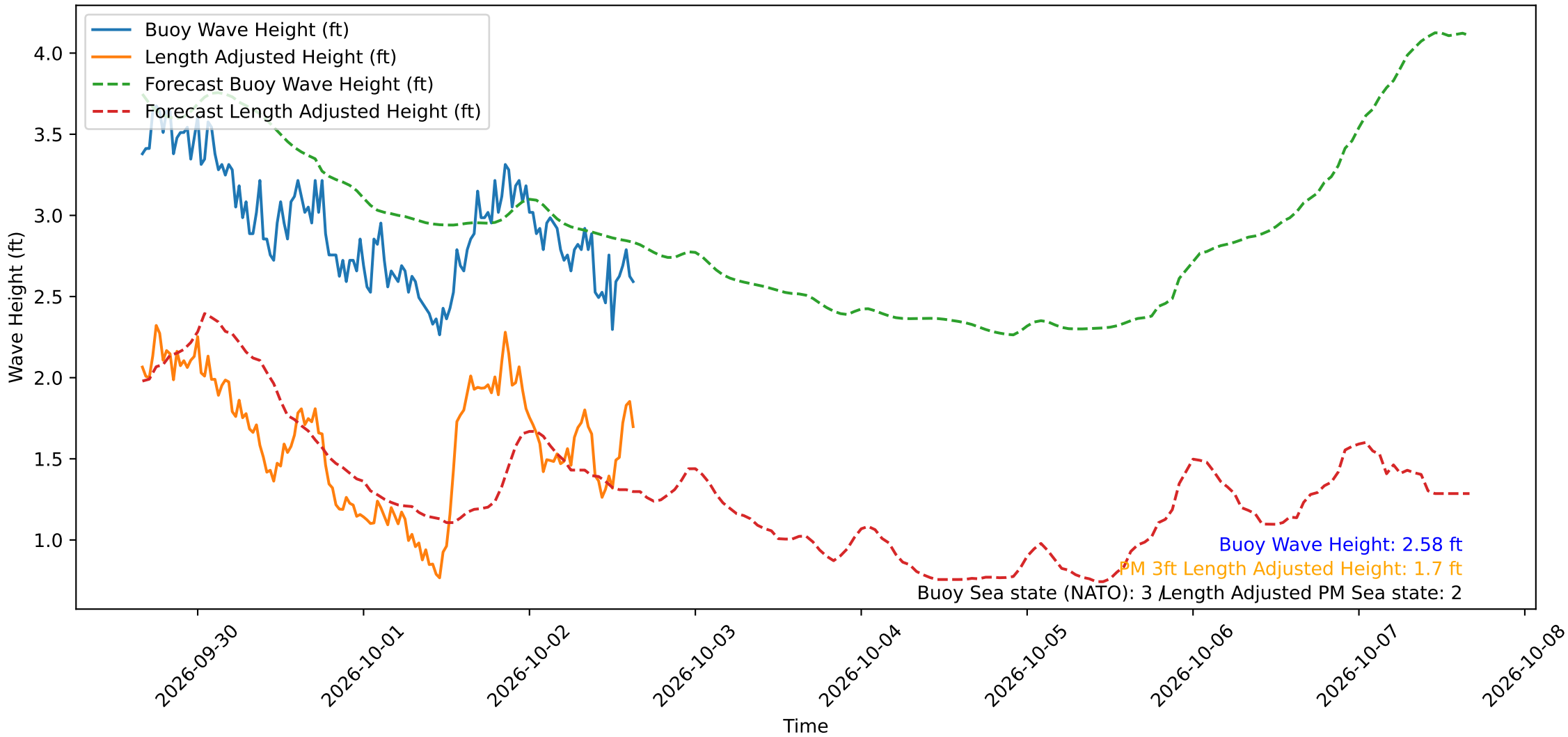
Wave Heights over Time for Oceanside Harbor at 2026-10-02 16:00:29
