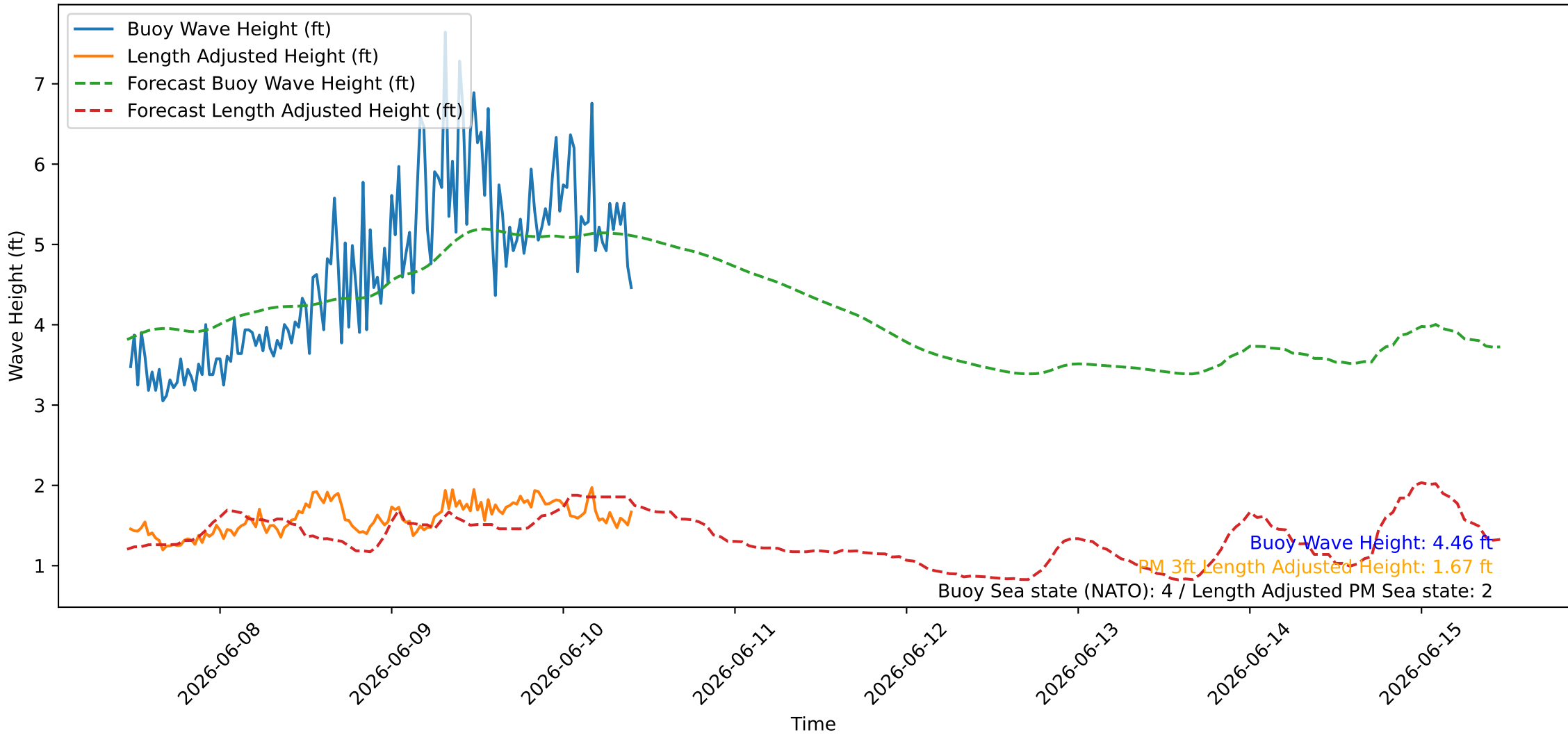
Wave Heights over Time for Red Beach at 2026-06-10 11:00:46
