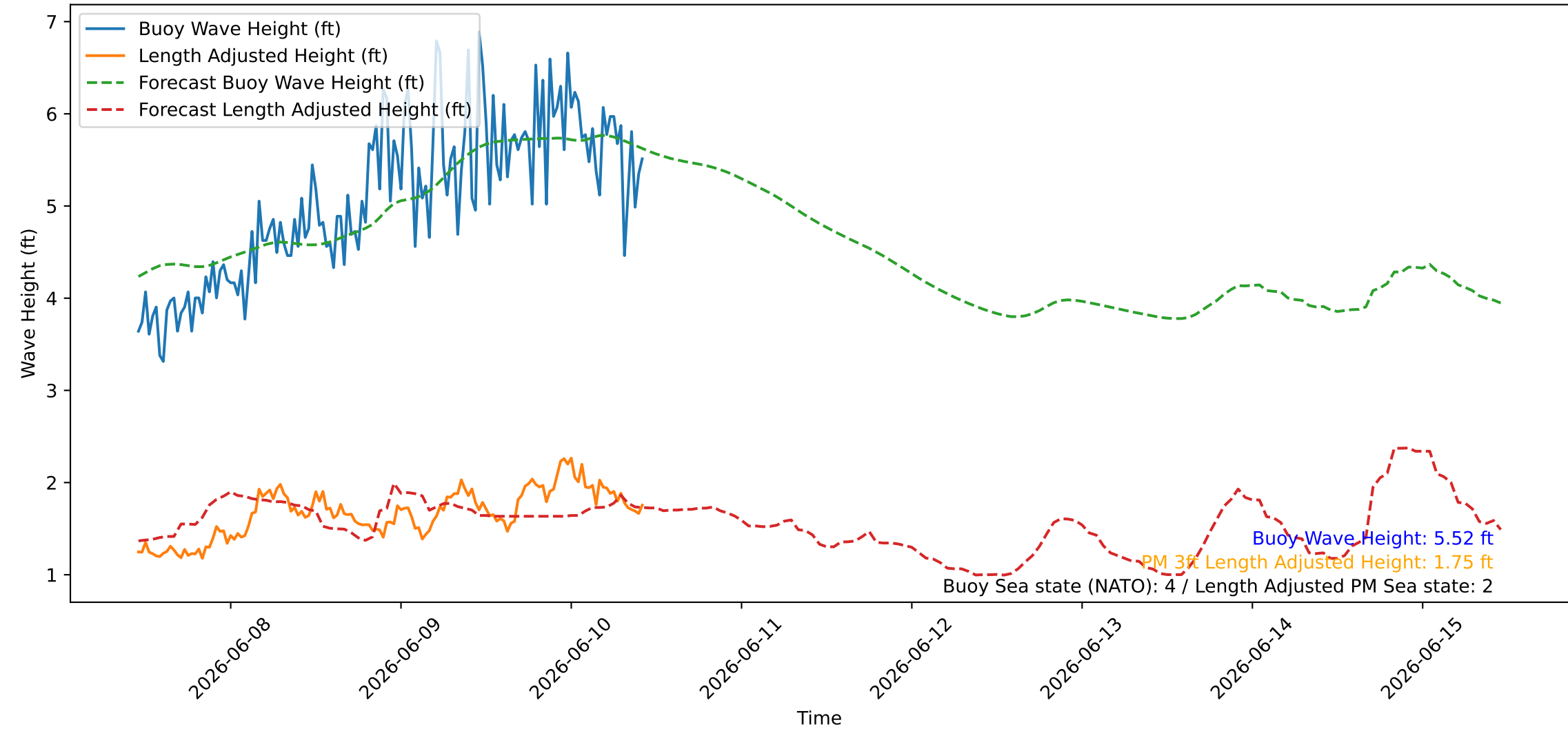
Wave Heights over Time for Green Beach at 2026-06-10 11:01:10
