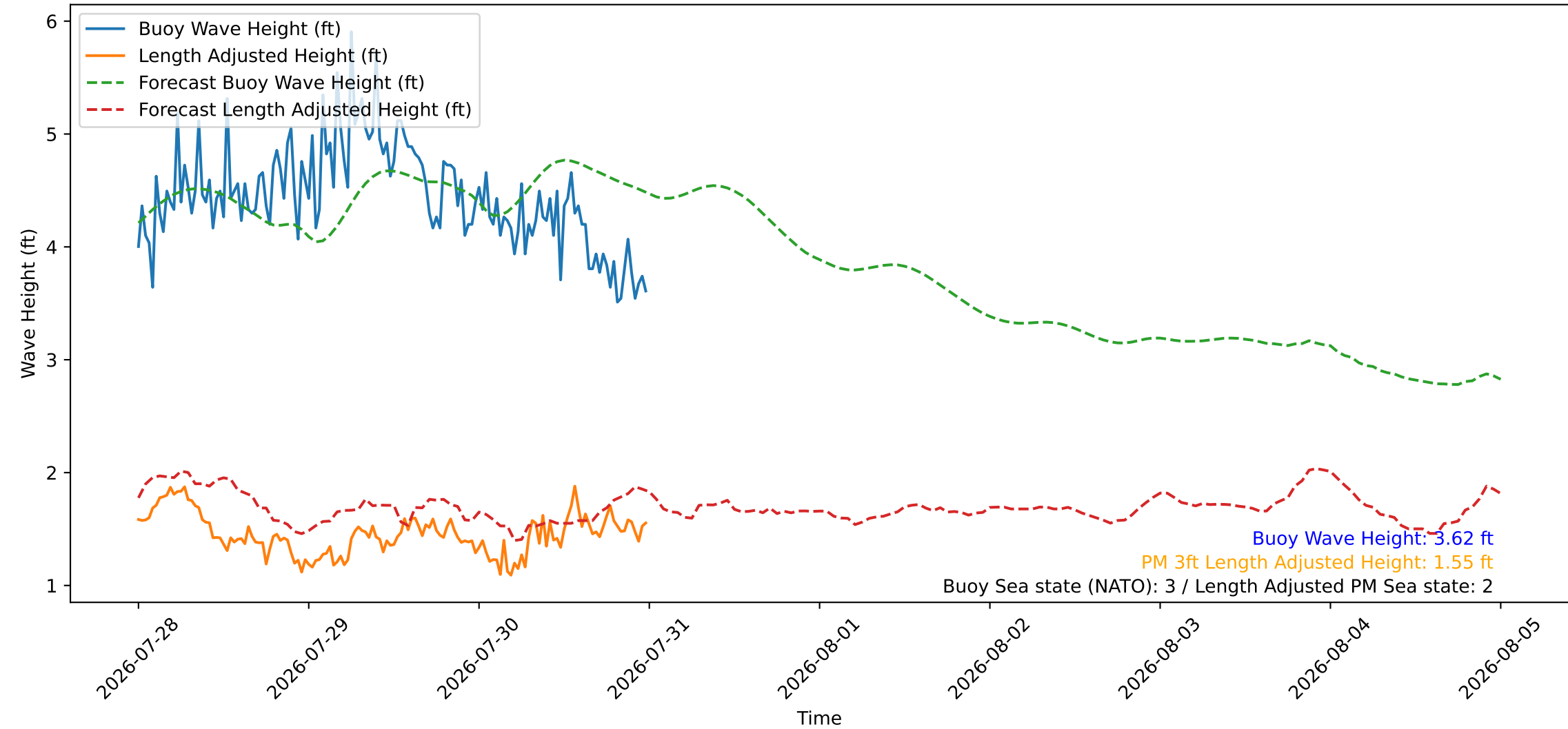
Wave Heights over Time for Oceanside Harbor at 2026-07-31 00:10:27
