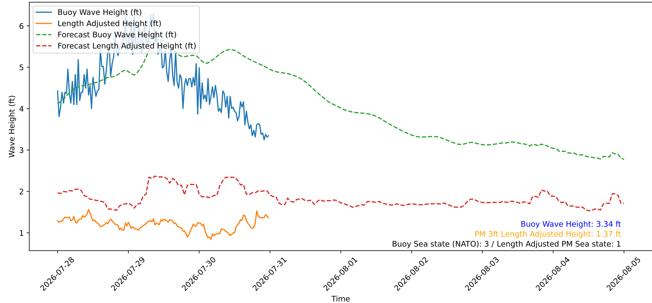
Wave Heights over Time for Green Beach at 2026-07-31 00:11:09
