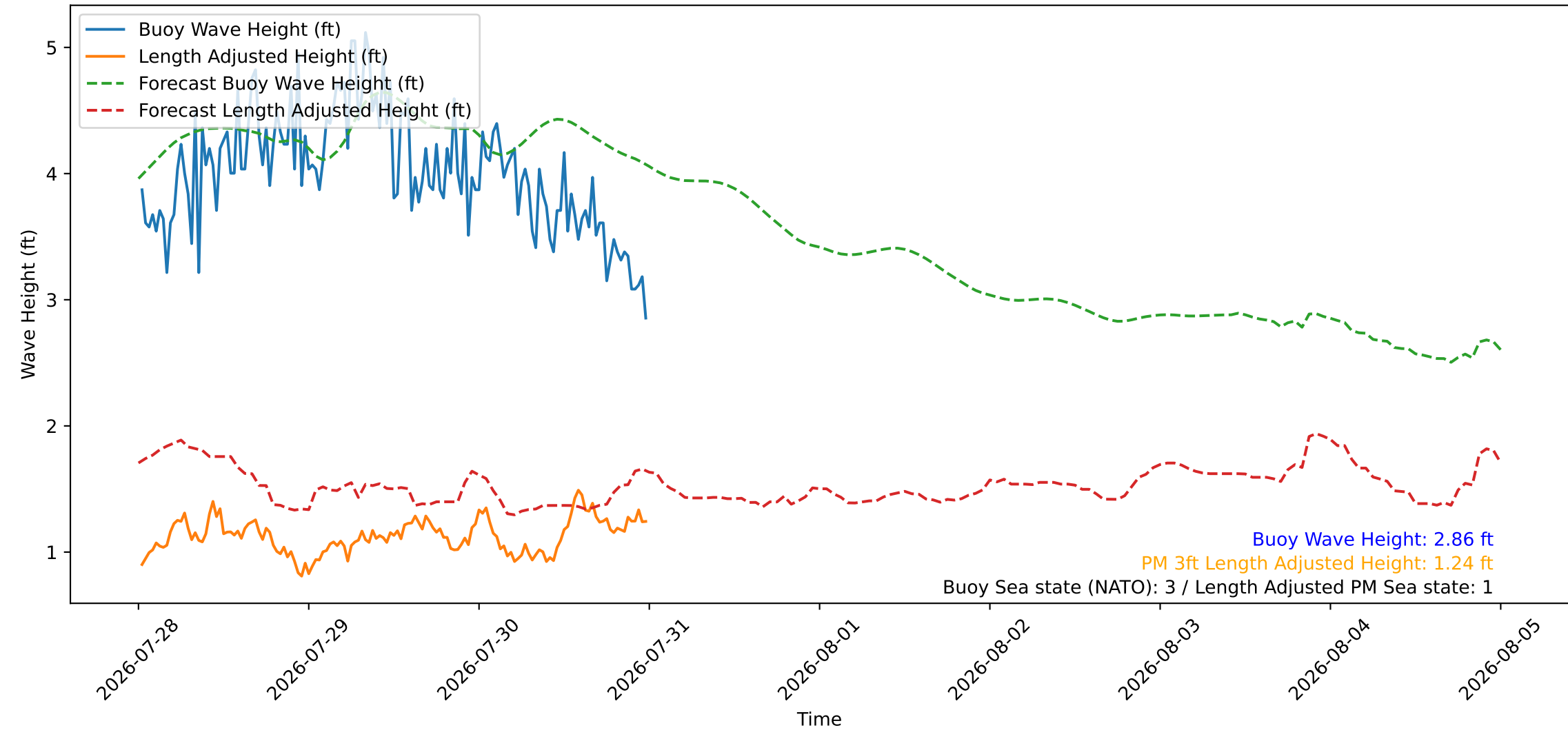
Wave Heights over Time for Red Beach at 2026-07-31 00:10:46
