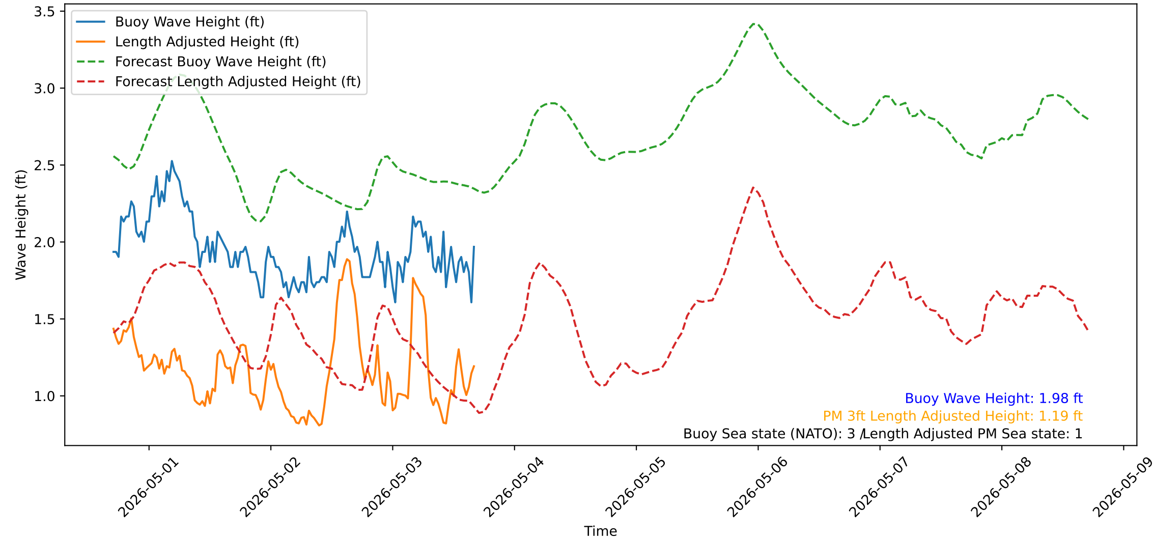
Wave Heights over Time for Red Beach at 2026-05-03 16:50:52
