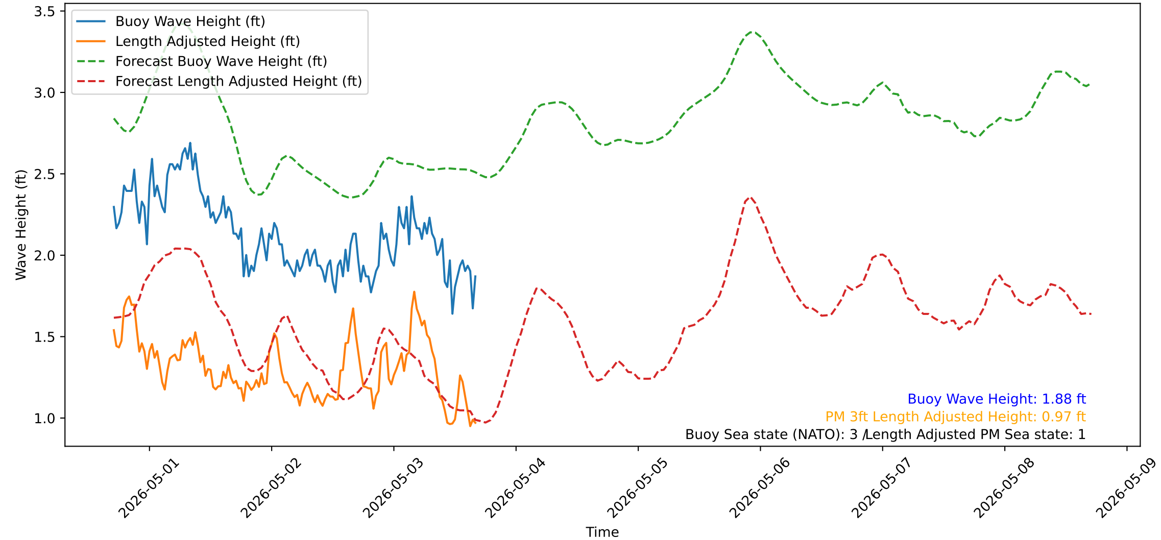
Wave Heights over Time for Oceanside Harbor at 2026-05-03 16:50:31
