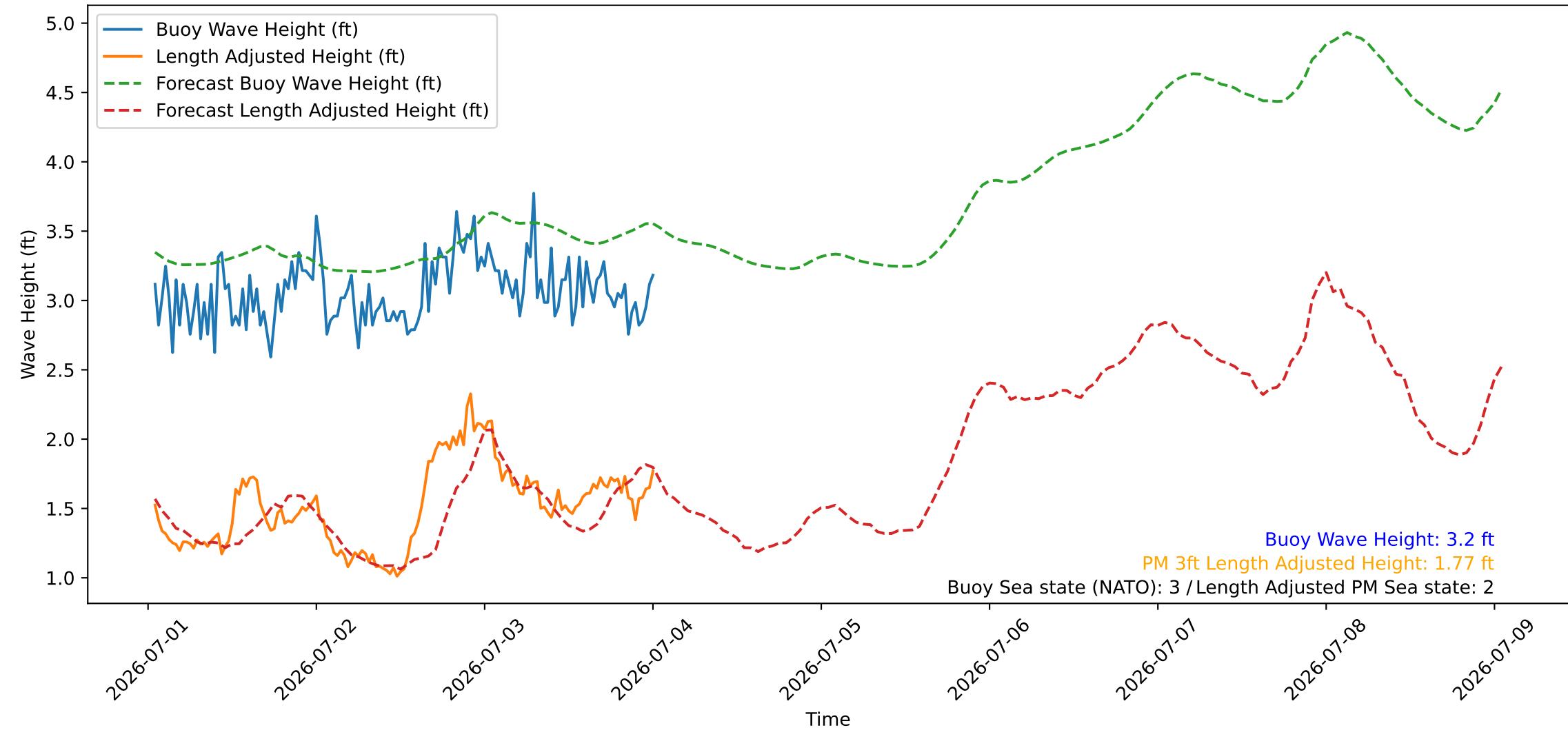
Wave Heights over Time for Oceanside Harbor at 2026-07-04 01:00:26
