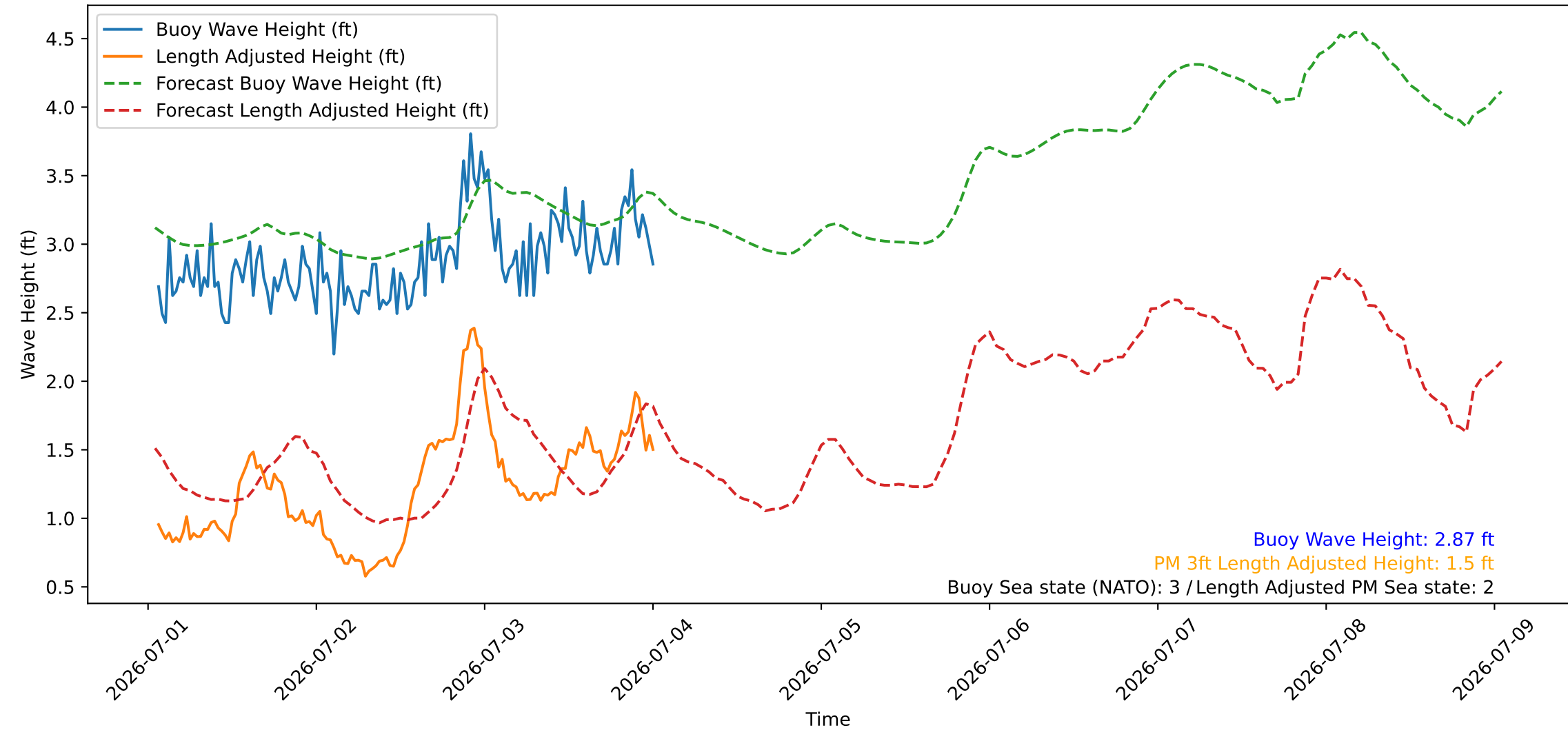
Wave Heights over Time for Red Beach at 2026-07-04 01:00:46
