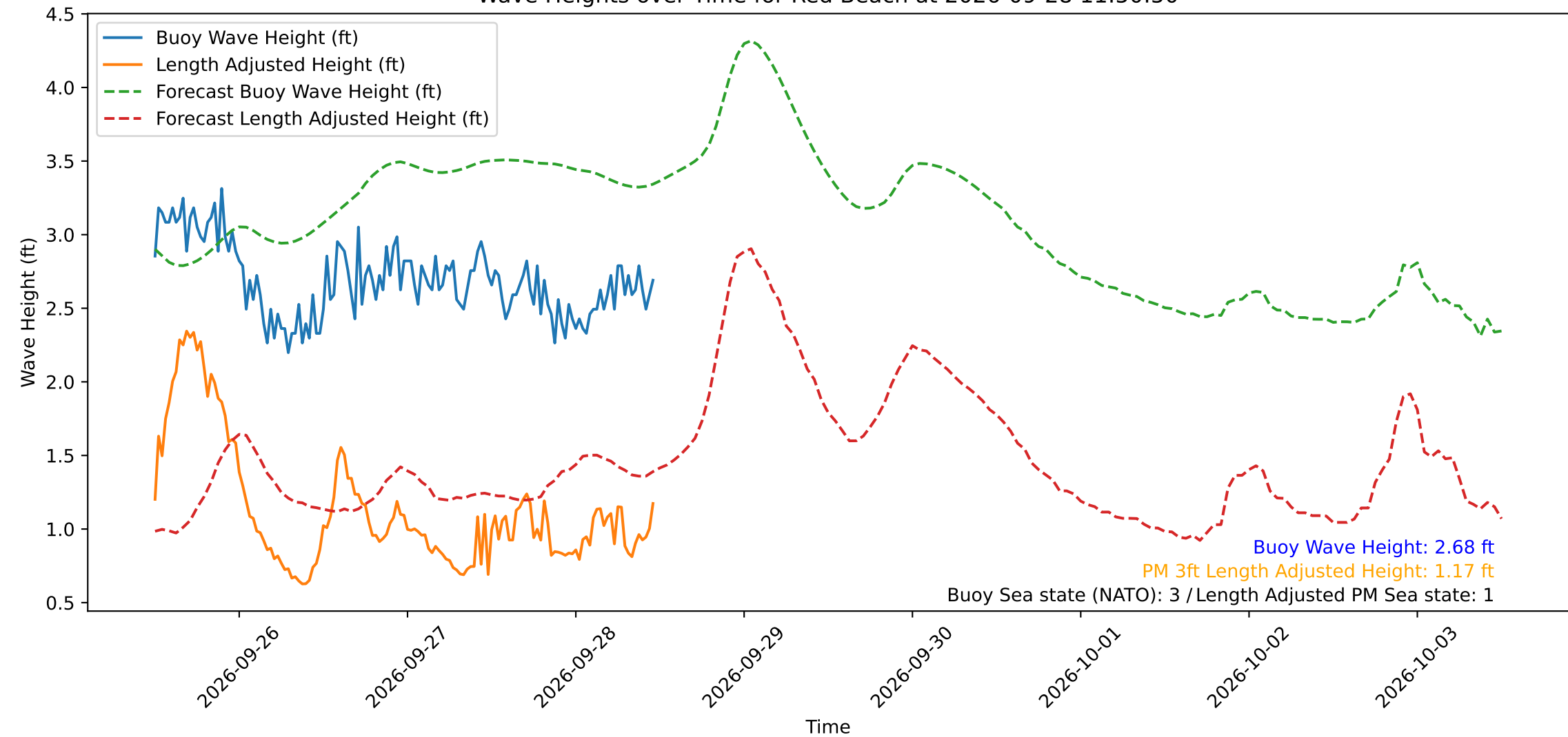
Wave Heights over Time for Red Beach at 2026-09-28 11:50:50
