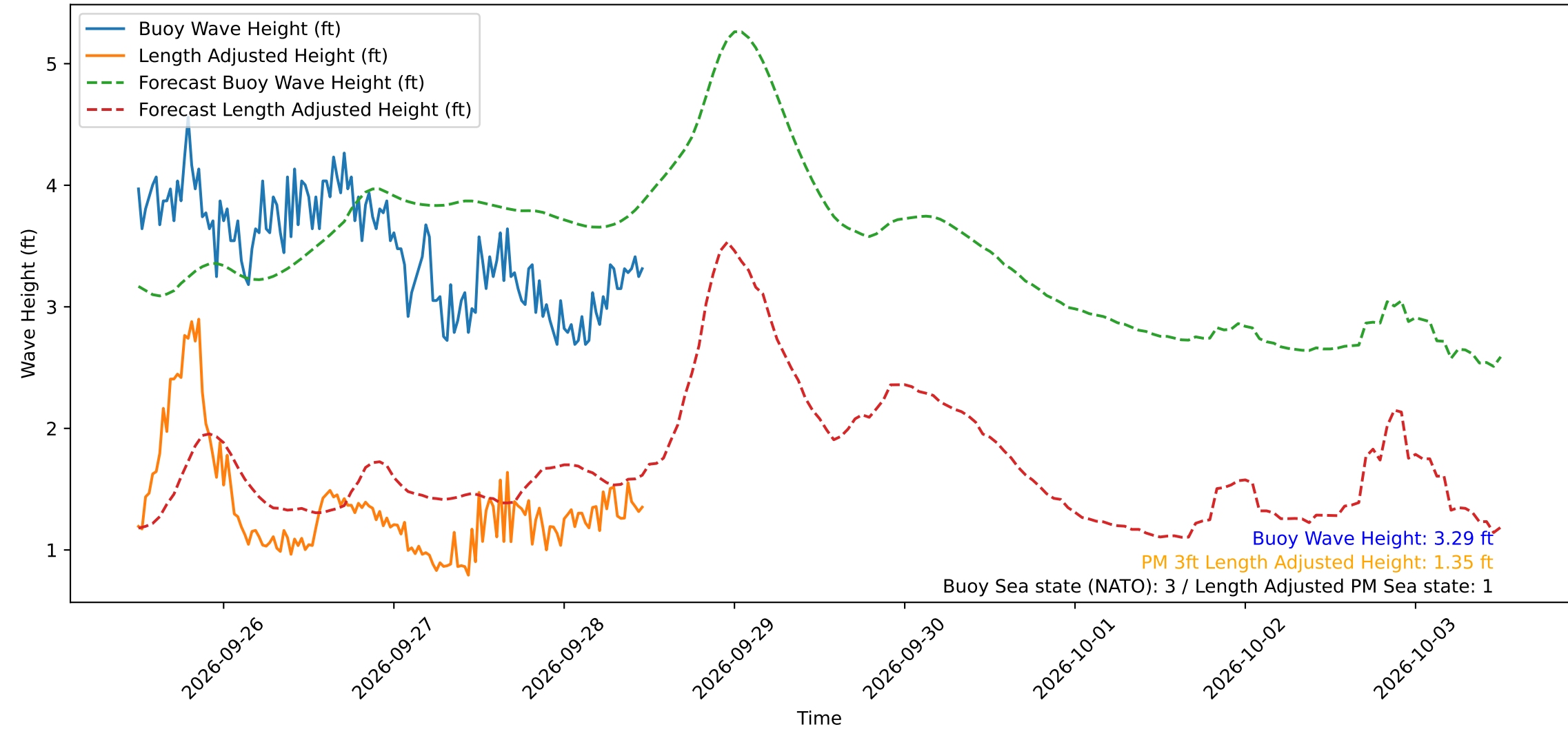
Wave Heights over Time for Green Beach at 2026-09-28 11:51:14
