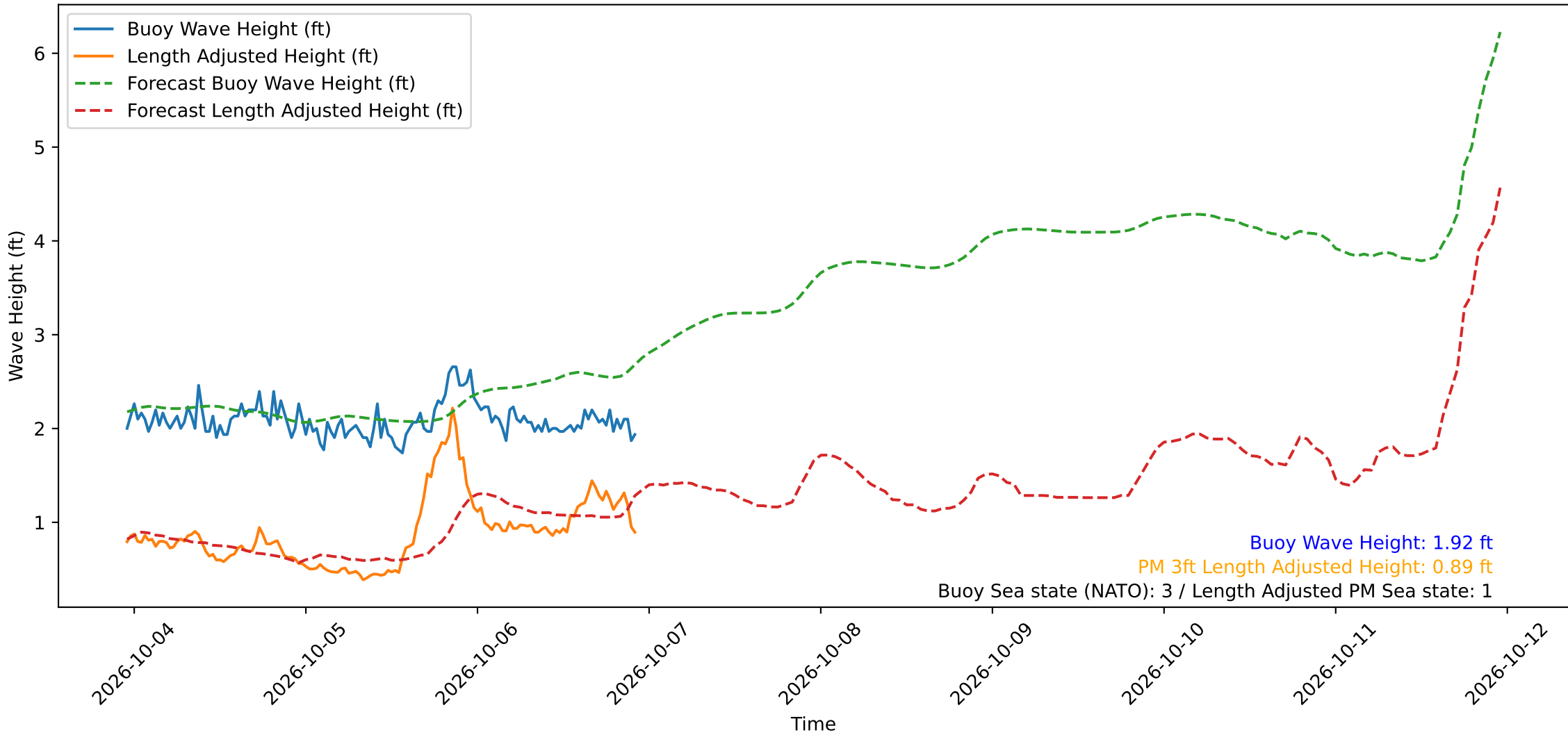
Wave Heights over Time for Red Beach at 2026-10-06 22:50:50
