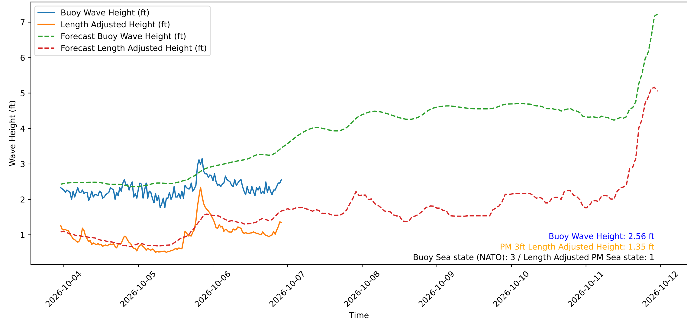
Wave Heights over Time for Green Beach at 2026-10-06 22:51:14
