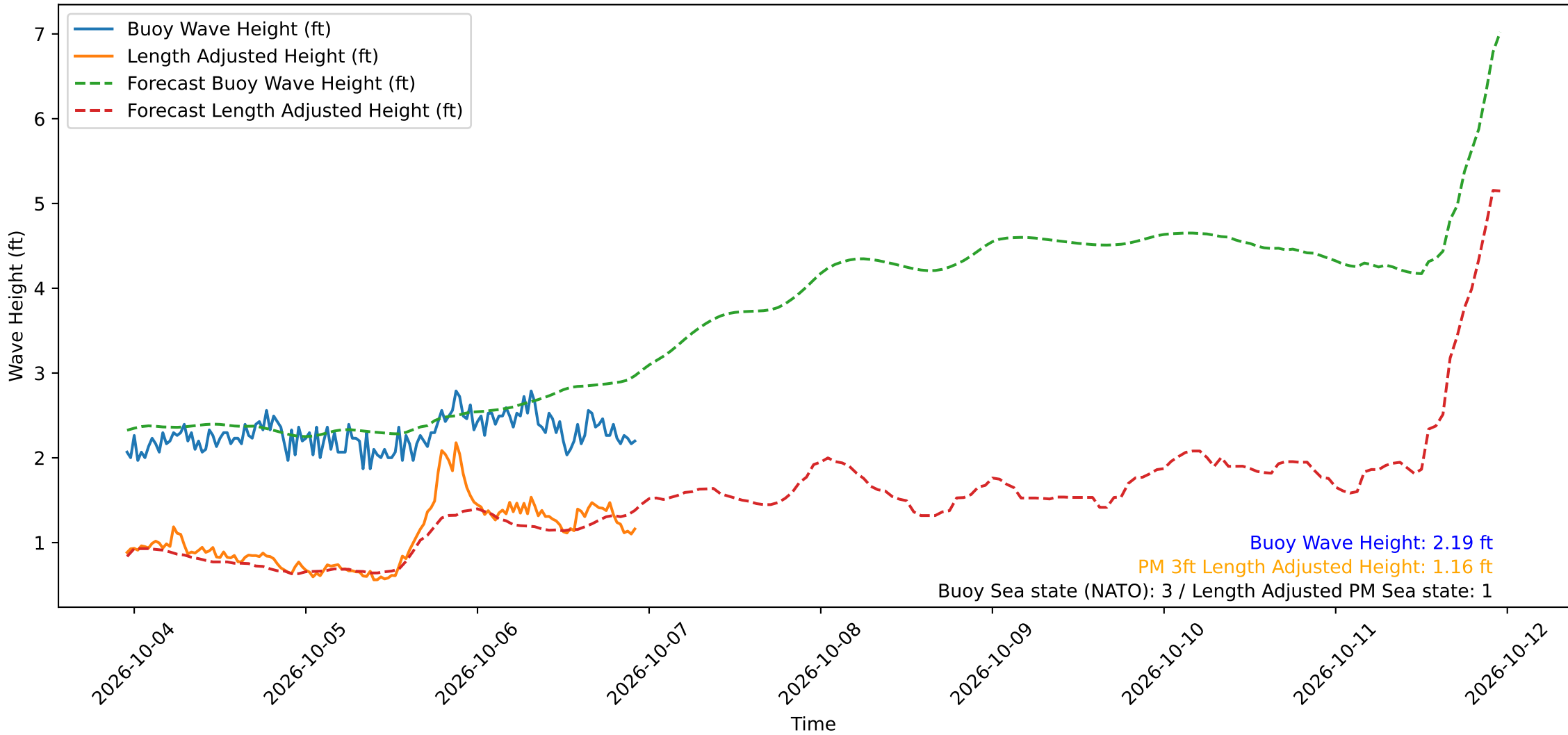
Wave Heights over Time for Oceanside Harbor at 2026-10-06 22:50:29
