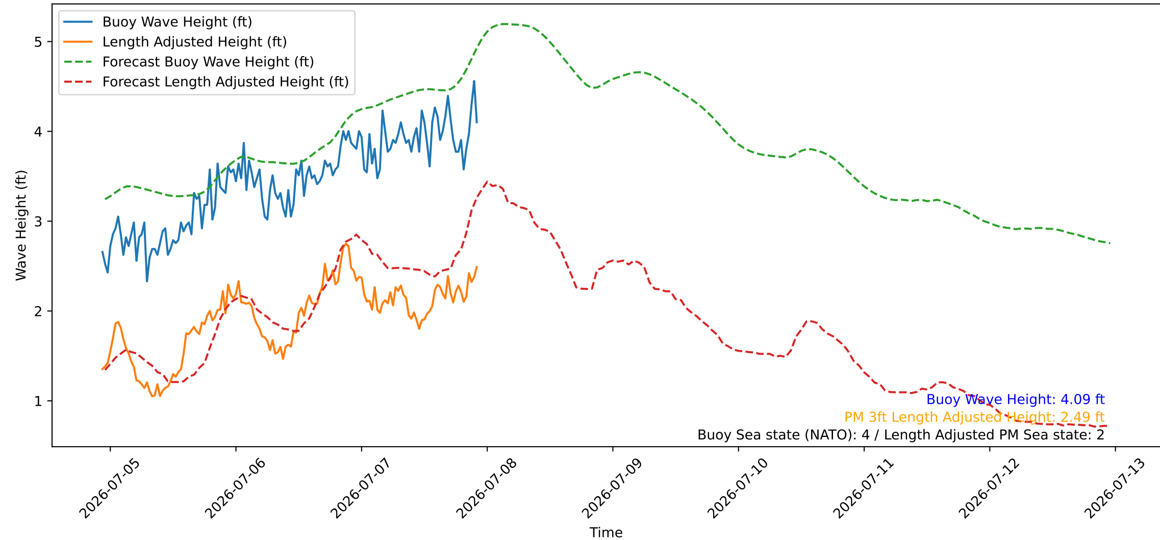
Wave Heights over Time for Oceanside Harbor at 2026-07-07 22:40:26
