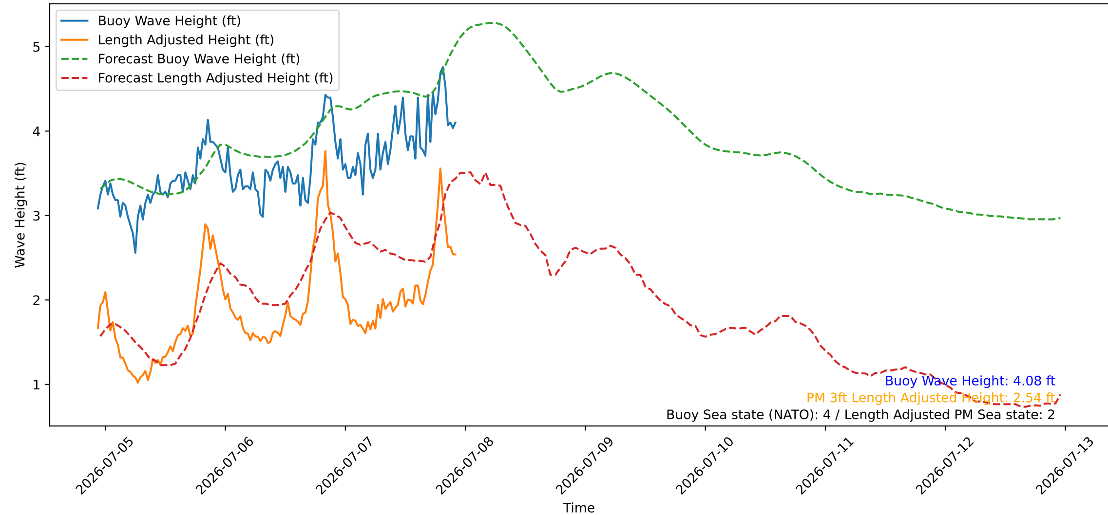
Wave Heights over Time for Green Beach at 2026-07-07 22:41:08
